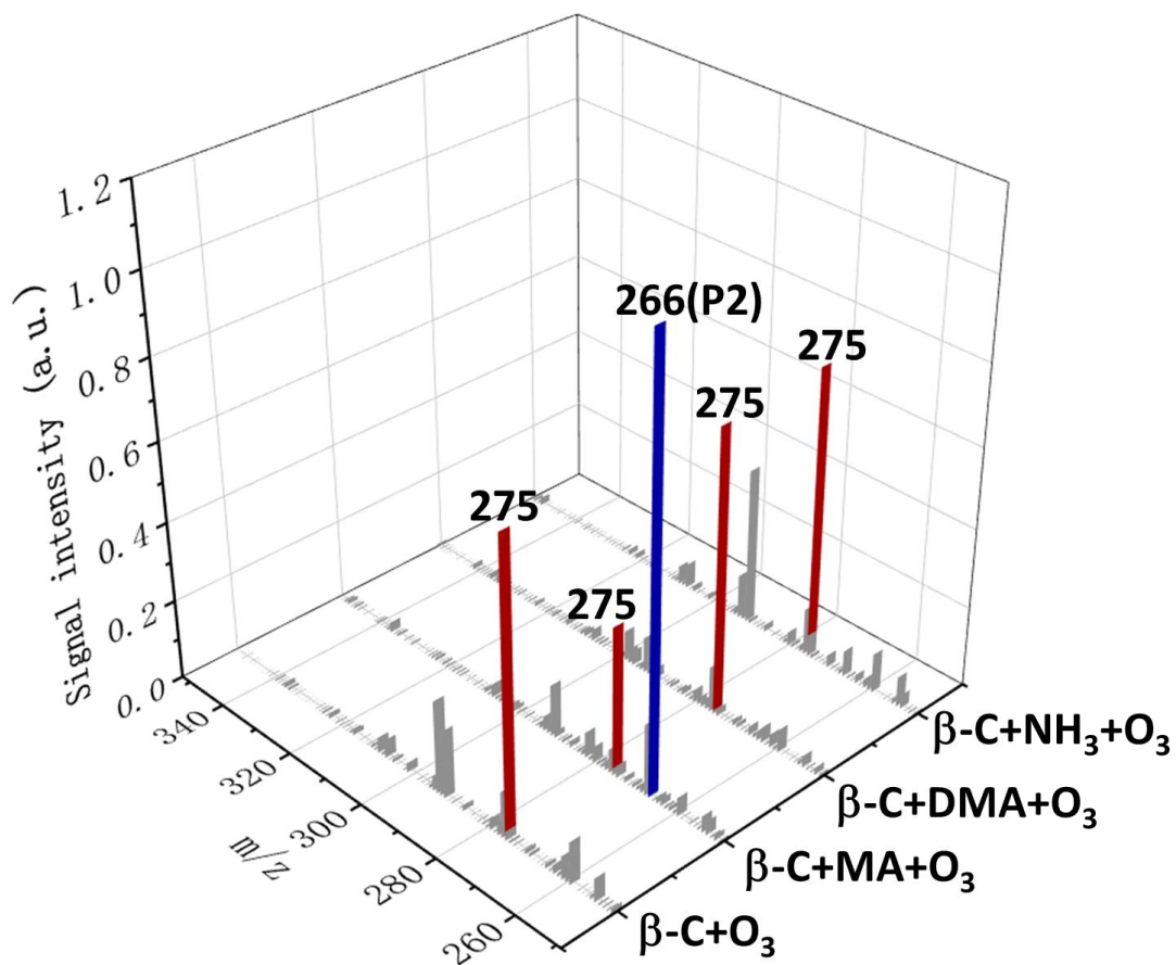
510 Figure 3 Positive-ion ESI mass spectra of the products extracted in AN/W (vol/vol = 4/1) from ozonolysis of \beta\text{-C} in the absence/presence of MA, DMA, or ammonia
