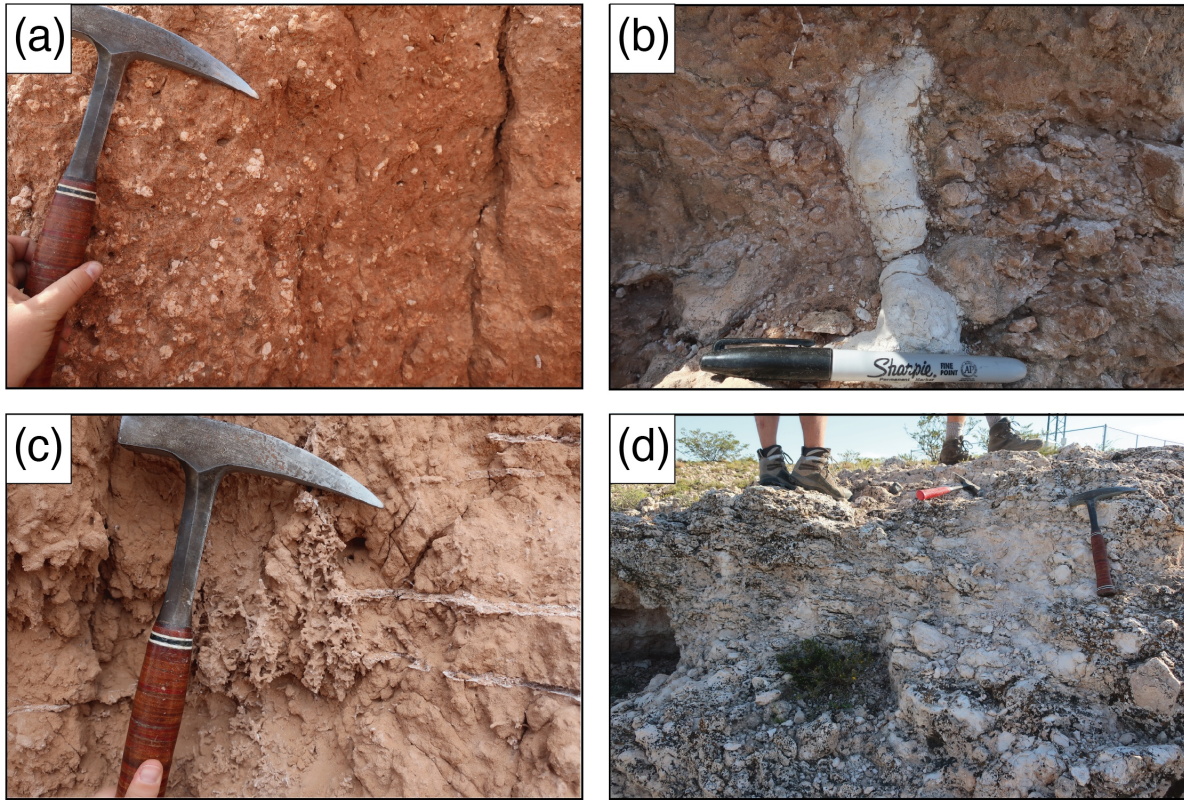
Figure 2. Field photos representing the primary types of authigenic carbonate sampled in this study. (a) Carbonate nodules. (b) Burrows. (c) Root casts. (d) The caprock Caprock calccrete, as pictured in SE New Mexico.
