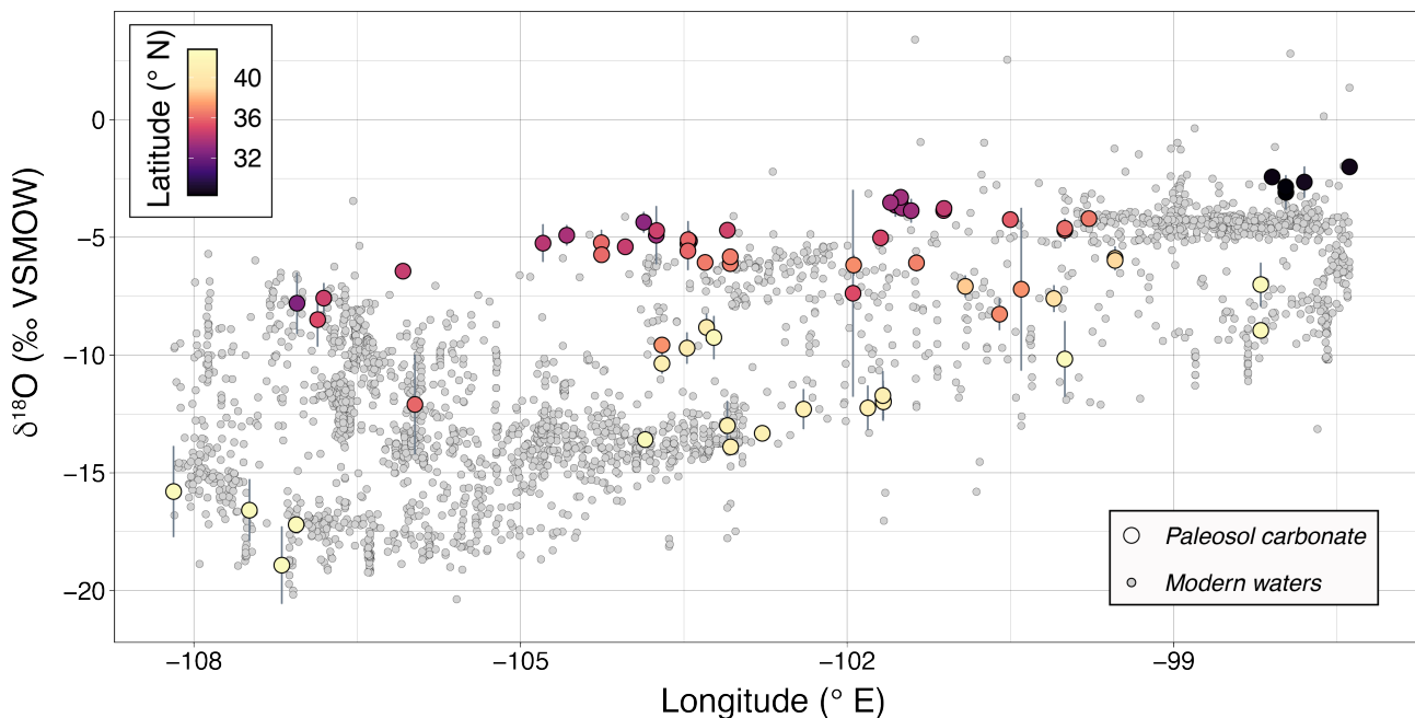
Figure 6. Modern meteoric water \delta^{18}\text{O} (small, gray circles) and reconstructed \delta^{18}\text{O}_p (large, colored circles) versus longitude. Reconstructed \delta^{18}\text{O}_p is colored with respect to latitude. Modern meteoric water data includes \delta^{18}\text{O} data from groundwater, river, and stream water, retrieved from the waterisotopes database (Waterisotopes Database, 2019). Vertical error bars are 1\sigma of the mean section \delta^{18}\text{O} data.
