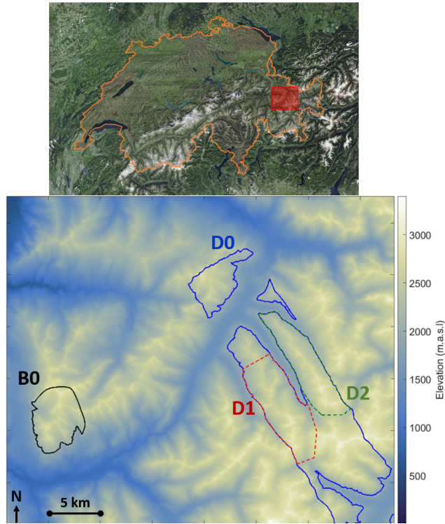
Figure 1. Overview of the study area: location of the domain in Switzerland (top, domain in red, Swiss borders in orange, source: swisstopo) and digital elevation model of the domain at 25 m resolution (bottom), with borders of subdomains B0, D0, D1 and D2. D1 and D2 are part of D0.
