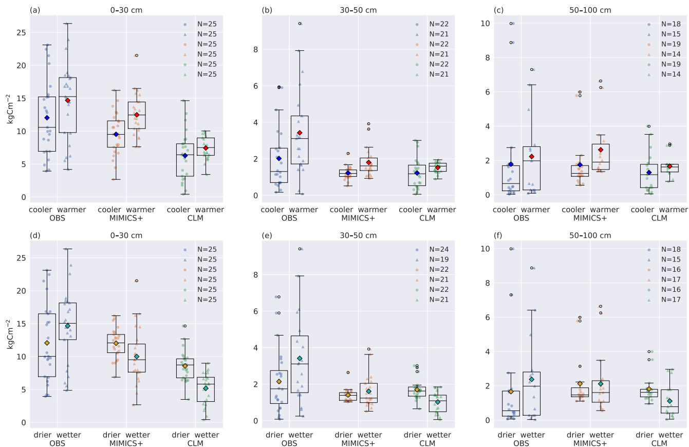
Figure 6. Total carbon stocks for cooler/warmer (a–c) and dryer/wetter (d–f) parts of the dataset. Box plots of carbon stocks in the (a), (d) top 30 cm, (b), (e) 30–50 cm, (c), (f) 50–100 cm soil depths for observed profiles from Strand et al. (2016) (left), simulated with MIMICS+ (center) and with CLM (right). In (a–c) the leftmost quartiles represent the coldest 50 % of the dataset, while the rightmost represent the warmest 50 % of the dataset. In (d–f) the leftmost boxes represent the drier 50 % of the total subset, while the rightmost represent the wetter 50 %. The line in each box is the median, while the diamonds mark the mean values. The diamond color represent the climate category; yellow: drier, turquoise: wetter, blue: cooler, red: warmer. The box upper and lower edges are the 75th and 25th percentiles, respectively. The whiskers extend from the box by 1.5 times the inter-quartile range.
