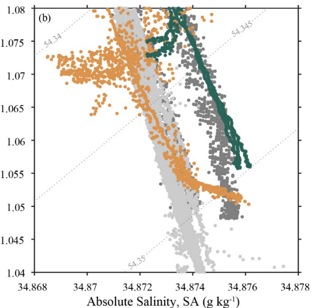
Figure 7. As in Figure 2 for the Japan Trench (JPT) and Izu-Ogasawara Trench (IOT). The grey is WOCE section P09 and P10. N.B the fresh tail increases in GO-SHIP P10 are statically unstable but within the \pm 0.002 instrument uncertainty. The same applies to shallow JPT profiles, but not shallower IOT profiles. These IOT profiles were excluded from further analysis.
