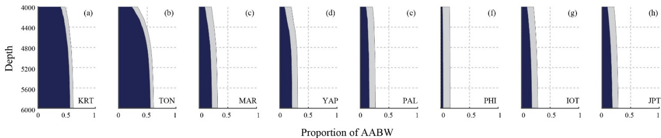
330 Figure 11. Proportion of Antarctic Bottom Water (AABW) in the abyssal waters above (a) KRT, (b) TON, (c) MAR, (d) €, (e) PAL, (f) PHI, (g) IOT and (h) JPT in the blue shaded profile. The proportion of LCDW is 1 minus the proportion shown. The grey area represents the range uncertainty between possible source water type combinations of AABW and LCDW in the SWT analysis. The standard error of the mean was less than 10^{-4} in all instances.
