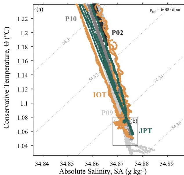
Figure 7. As in Figure 2 for the Japan Trench (JPT) and Izu-Ogasawara Trench (IOT). The grey is WOCE section P09 and P10. N.B the fresh tail increases in GO-SHIP P10 are statically unstable but within the \pm 0.002 instrument uncertainty. The same applies to shallow JPT profiles, but not shallower IOT profiles. These IOT profiles were excluded from further analysis.
