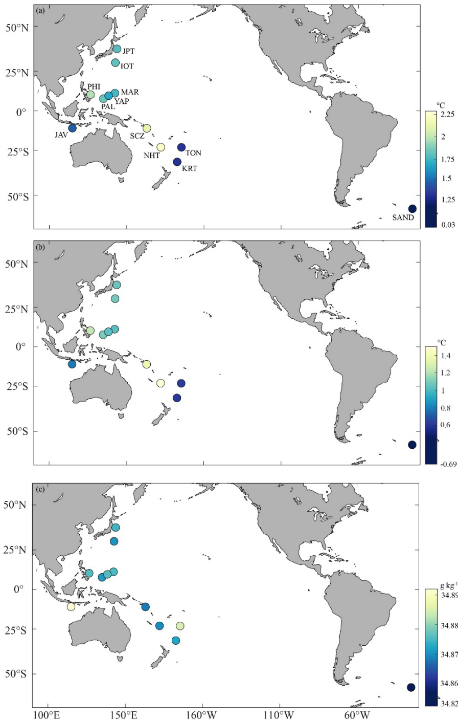
Figure 9. Conditions in each trench at 7000 m depth of (a) In-situ Temperature ( ^{\circ}\text{C} ) (b) Conservative Temperature ( ^{\circ}\text{C} ) and (c) Absolute Salinity ( \text{g kg}^{-1} ). JPT, Japan Trench, IOT, Izu-Ogasawara Trench, PHI, Philippine Trench, PAL, Palau Trench, YAP, Yap Trench, MAR, Mariana Trench, SCZ, Santa Cruz Trench, NHT, New Hebrides Trench, KRT, Kermadec Trench, TON, Tonga Trench, JAV, Java Trench, SAND, South Sandwich Trench.
