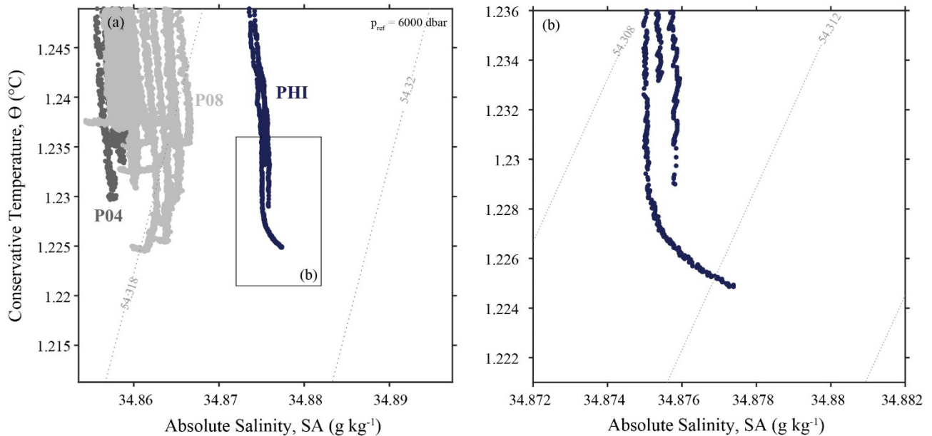
290 Figure 8. As in Figure 2 for the Philippine Trench. The grey is WOCE section P08 and GO-SHIP P04. N.B the fresh tail increase in P08 is statically unstable.
