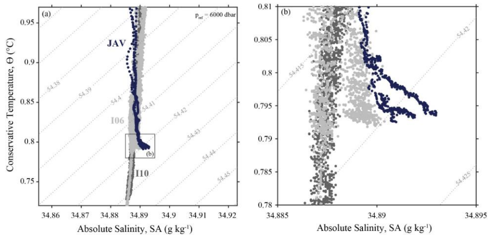
305 Figure 3. As in Figure 2 for the Java Trench. The grey is WOCE section I06 and I10.
