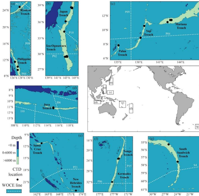
Figure 1. Geographic locations of the hadal trenches used in this study, including CTD deployment locations marked in black. (a) Ryukyu Trench and Philippine Trench; (b) Japan Trench and Izu-Ogasawara Trench; (c) Palau Trench, Yap Trench, and Mariana Trench; (d) Java Trench (e) Santa Cruz Trench and New Hebrides Trench; (f) Tonga Trench and Kermadec Trench and (g) South Sandwich Trench. Individual deployment details are provided in Table S1. Bathymetric details and features are provided in Table S1. Ocean elevation data was sourced from the GEBCO Compilation Group (2021) and reproduced using m_map in MATLAB (Pawlowicz 2020).
