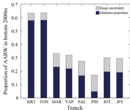
365 Figure 12. Proportion of AABW in the bottom 2000 m of trenches in the western Pacific. The proportion of LCDW is the remainder of the proportion to equal 1. The range uncertainty is the mean range between possible source water type combinations of AABW and LCDW in the SWT analysis (Table 2). The standard error of the mean was less than 10^{-4} in all instances.
