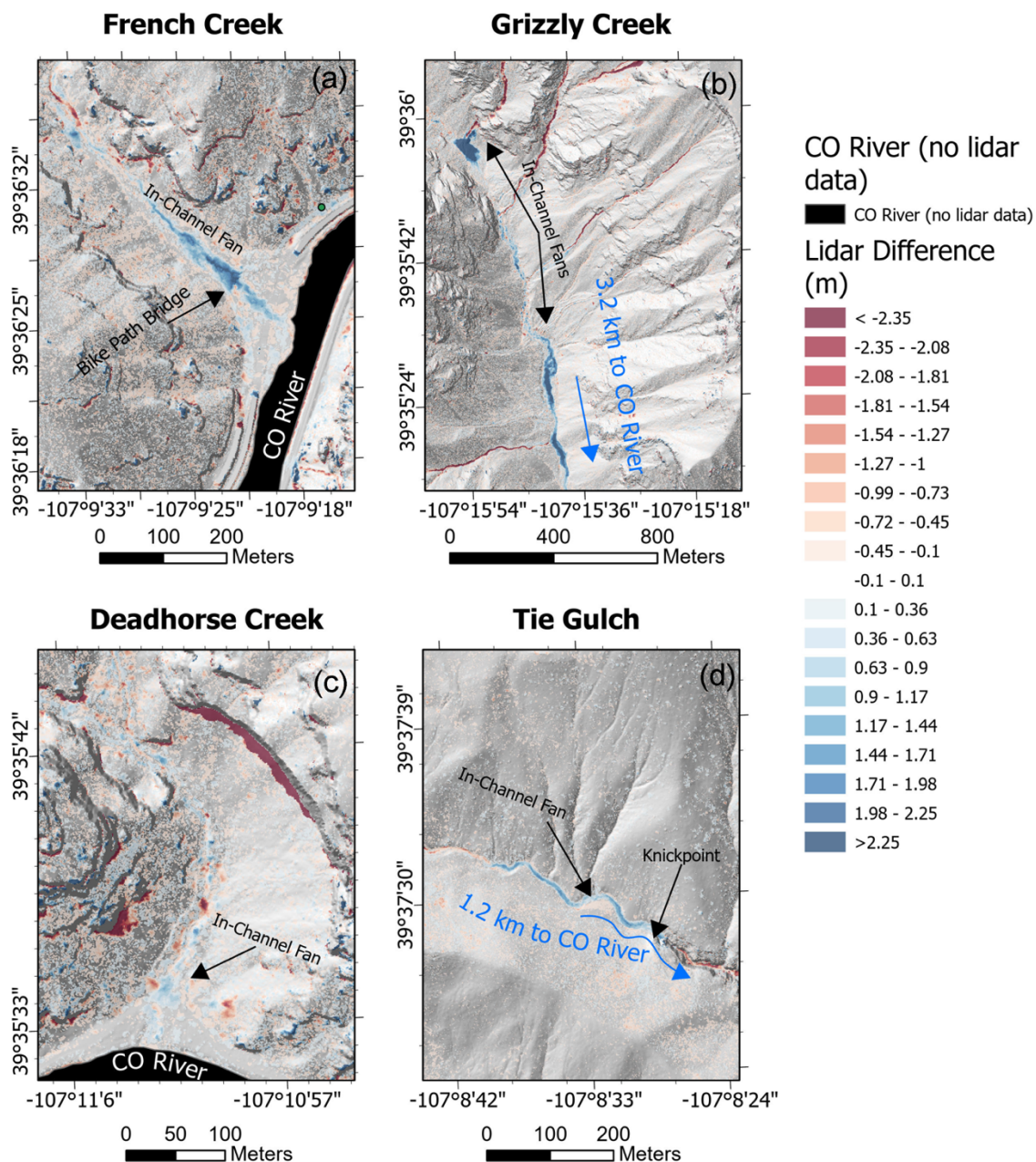
745 Figure 5. In-channel sediment deposits in large drainage basins. (a) French Creek: a fan forms upstream of the Colorado River, primarily because sediment is blocked by a concrete bike path bridge. (b) Grizzly Creek: Several in-channel fans formed several kilometers upstream of the Colorado River. No fan formed at the outlet of Grizzly Creek. (c) Deadhorse Creek: relatively minor depositional fan forms upstream of the Colorado River. (d) Tie Gulch: In-channel fan develops upstream of a knickpoint.
