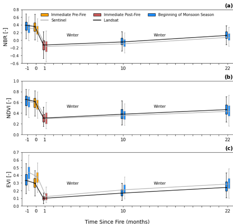
785 Figure 10. Landsat- (black outline) versus Sentinel-derived (gray outline) measurements of the (a) Normalized Burn Ratio (NBR), (b) Normalized Difference Vegetation Metric (NDVI), and (c) Enhanced Vegetation Index (EVI) for the 2020 Grizzly Creek Fire. Boxplots summarize the distribution of the mean reflectance metric for each modelled basin (USGS 2022) that intersects the burn area for the beginning of monsoon season (blue), immediately before the fire (orange), and immediately after the fire (red).
