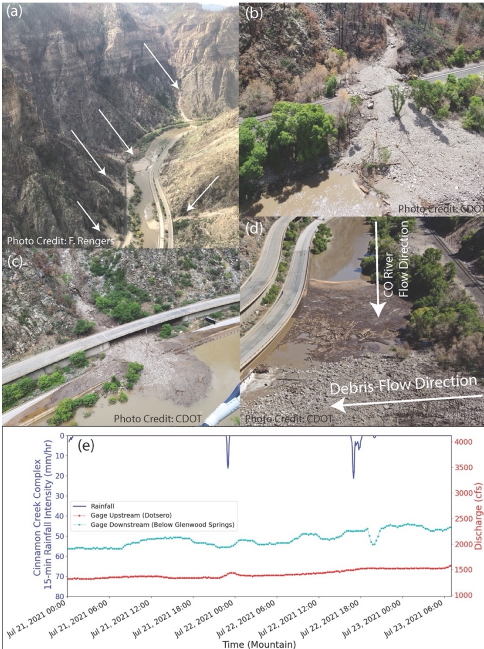
795 Figure 11. (a) View of debris flow paths and deposits in the Colorado River looking southwest on 18 August 2021. Arrows indicate new debris flow paths. (b) Sedimentation on the railroad in Glenwood Canyon on 1 August 2021. (c) Sedimentation on the lower deck of I-70 on 1 August 2021. (d) Photo of temporary damming of the Colorado River on 22 July 2021. Damming can be observed in the discharge record of the Colorado River on 22 July 2021. The upstream discharge in the Colorado River (Red) rises steadily in response to the closest measured 15-minute rainfall intensity (Blue). When the debris flow at Devil's Hole temporarily dammed the Colorado River, a drop in discharge is observed at the downstream river gauge (Cyan).
