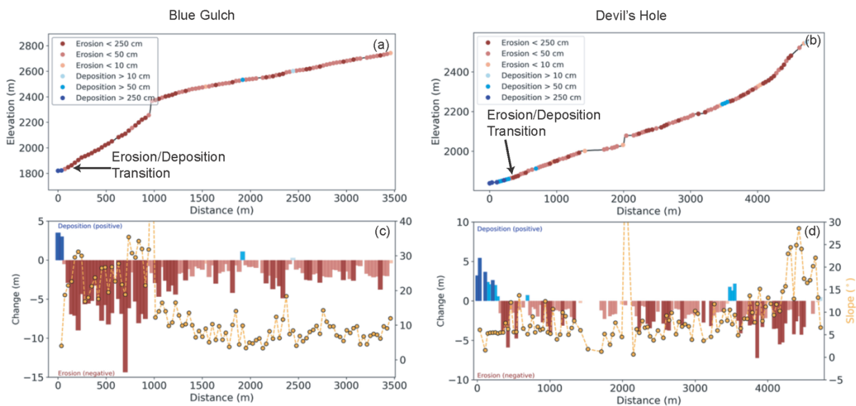
Figure 3. (a and b) Elevation as a function of distance from the watershed outlet for the Blue Gulch watershed (a) and Devil's Hole watershed (b). Red dots and blue dots represent erosion/deposition, respectively. Areas without a dot did not experience change beyond the level of detection. (c and d) Measured deposition and erosion as a function of distance from the watershed outlet (primary y-axis). Local slope is shown on the secondary y-axis.
