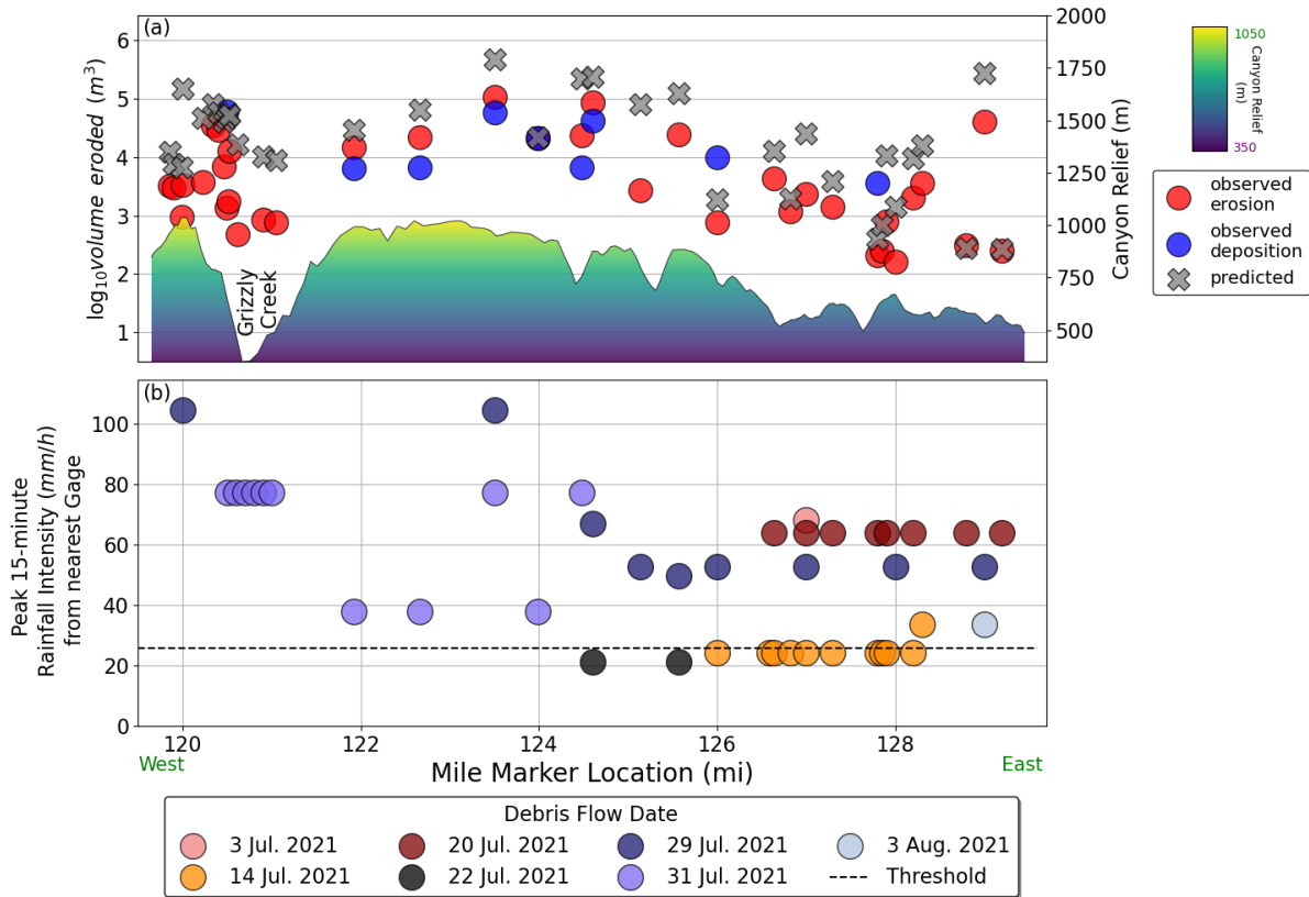
760 Figure 7. (a) Observed sediment volume (erosional and depositional) and predicted sediment volume using Equation 2 shown as a function of the mile marker location in Glenwood Canyon. For context, the canyon relief is shown on secondary axis. The relief profile indicates the elevation from the north side of the canyon approximately parallel to I-70. (b) Peak 15-minute rainfall intensity from the nearest representative gauge shown at locations identified by debris flow date. Note that channel polygons were associated with a mile marker location at the watershed outlet, as this was the preferred method of identification by CDOT personnel. In cases where the channel outlet did not directly intersect I-70, the outlet was simply translated onto a line segment representing I-70 to estimate a mile marker location.
