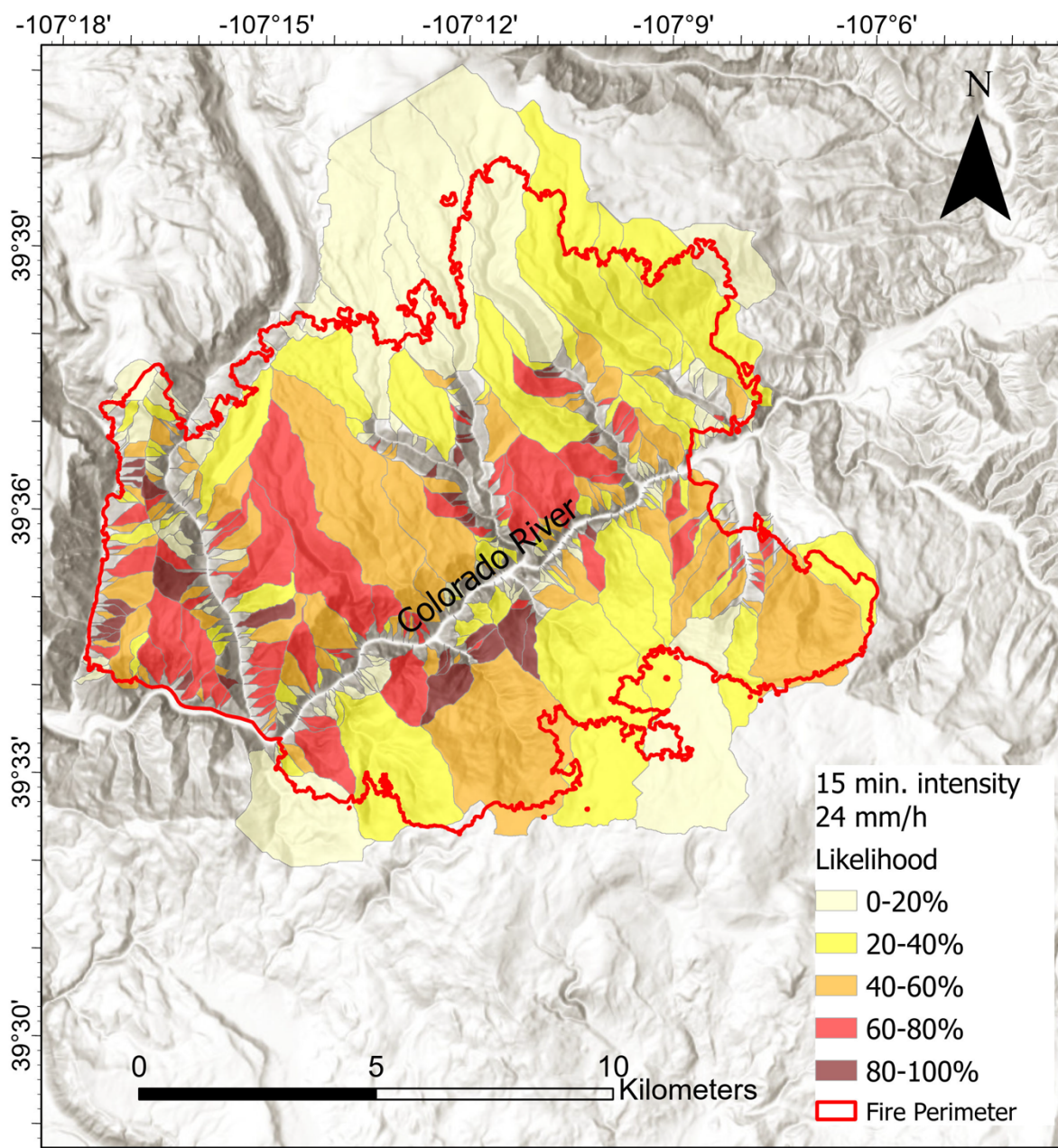
720 Figure 1. USGS Debris Flow Hazard likelihood estimate produced for the Grizzly Creek Fire perimeter using Equation 1. The likelihood of debris flow initiation is shown for a modeled rainstorm with a 15-minute rainfall intensity of 24 mm h -1 .
