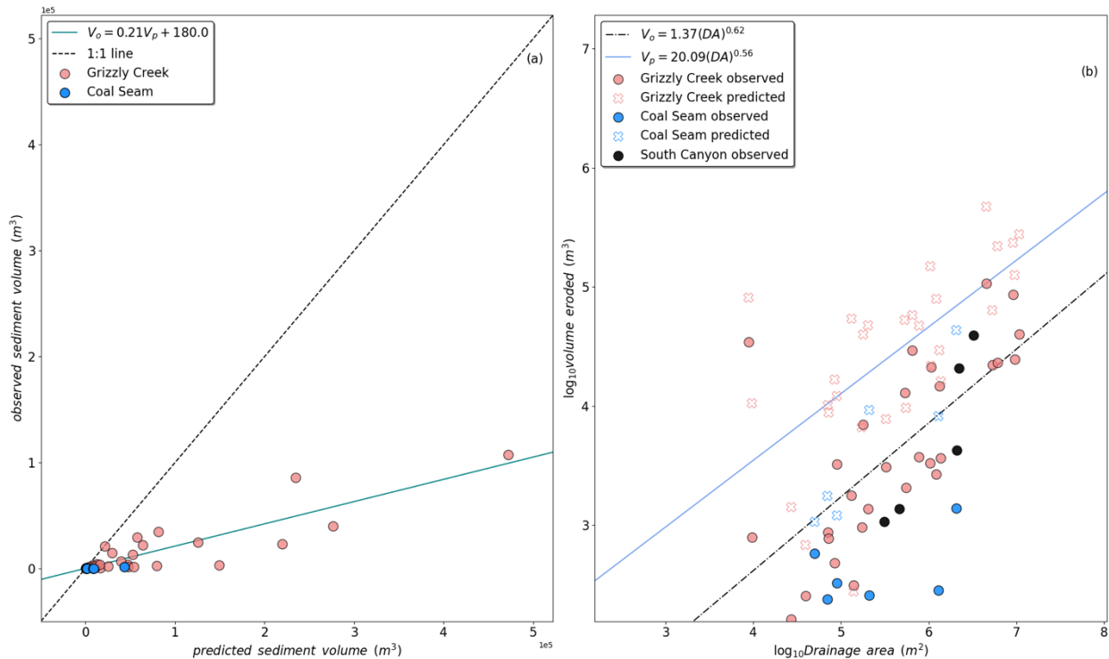
Figure 9. (a) Observed sediment volume (erosional) versus predicted sediment volume using Equation 2 . Linear trendline shows the relationship between the predicted ( V_p ) and observed ( V_o ) volume at the Grizzly Creek Fire. (b) A comparison of the total volume of observed sediment with predicted volume from Equation 2 as a function of upstream drainage area (DA). The observation volumes represent the volume of erosion, upstream of a transition to deposition. Best-fit power law equations were fit to the observed and predicted data points for the Grizzly Creek Fire, respectively.
