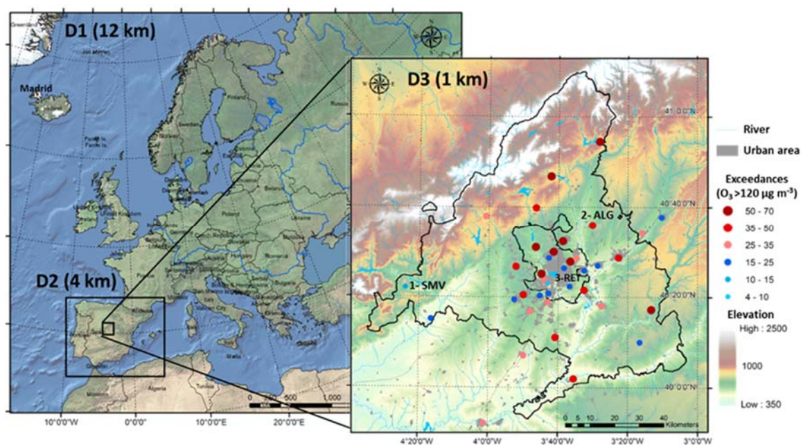
850 Figure 1. Modeling domains including the location of the air quality monitoring stations within the innermost domain and number of exceedances of the O 3 target value for protection of human health (MDA8 > 120 \mu\text{g}\cdot\text{m}^{-3} ) in 2016.
