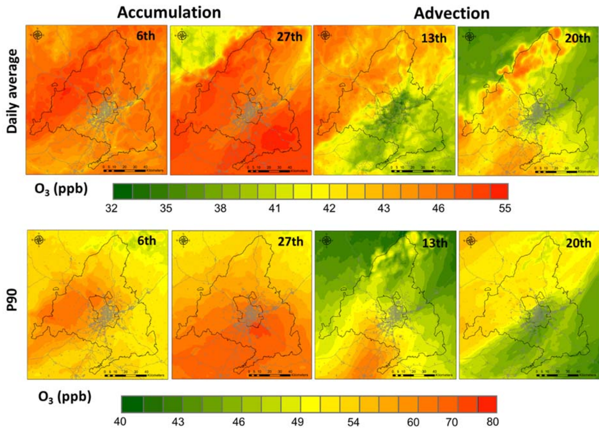
870 Figure 6. Daily mean (top) and 90 th percentile (bottom) of O 3 levels (ppb) during accumulation (6 th and 27 th July, 2016) and advective (13 th and 20 th July, 2016) periods
