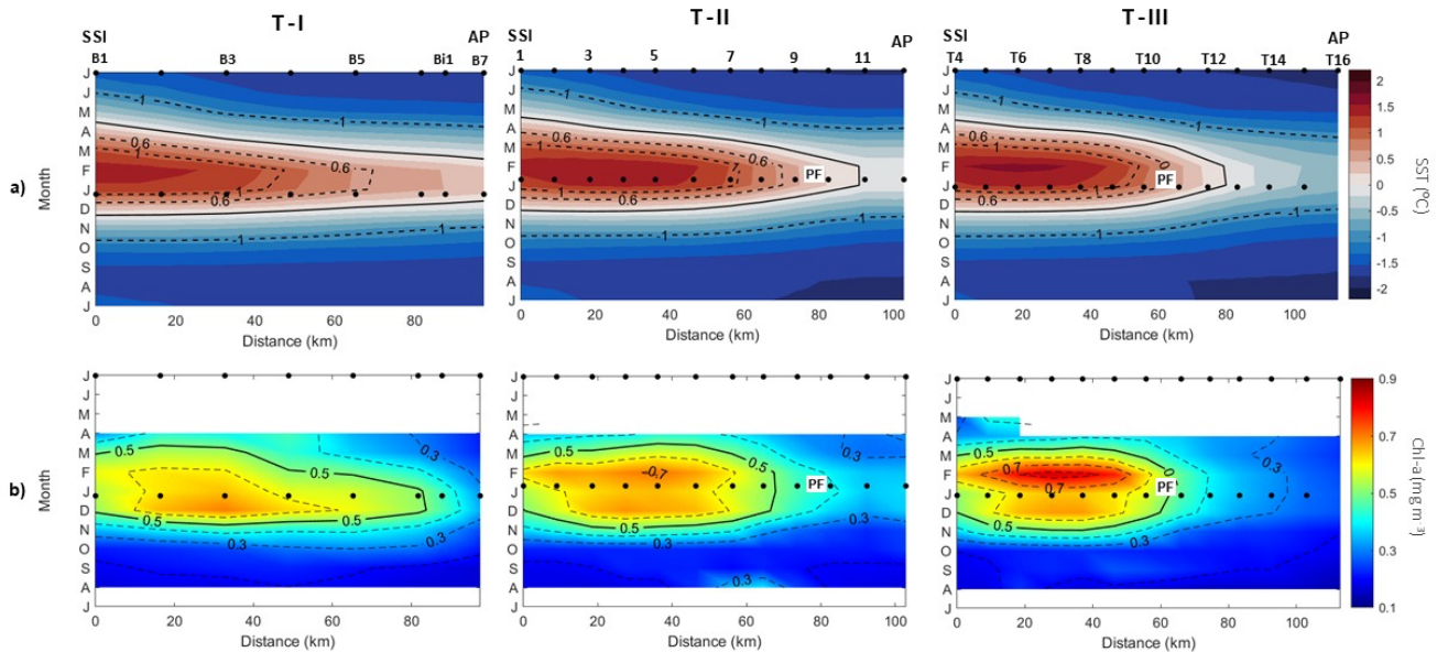
Figure 10. Monthly climatology from 1998 to 2018 of a) Sea Surface Temperature (SST), and b) chlorophyll-a (chl-a) concentration for each study transect (see Figures 2-4) from the South Shetland Islands (SSI) to the Antarctic Peninsula (AP). The black markers (dots) situated at the top of the subplots represent the station's positions along the transects. These same stations are also displayed during the summer months when the cruises were carried out. Additionally, the position of the Peninsula Front (PF), as identified during the cruises and located along the isopycnal of 27.55 kg m -3 , is also indicated.
