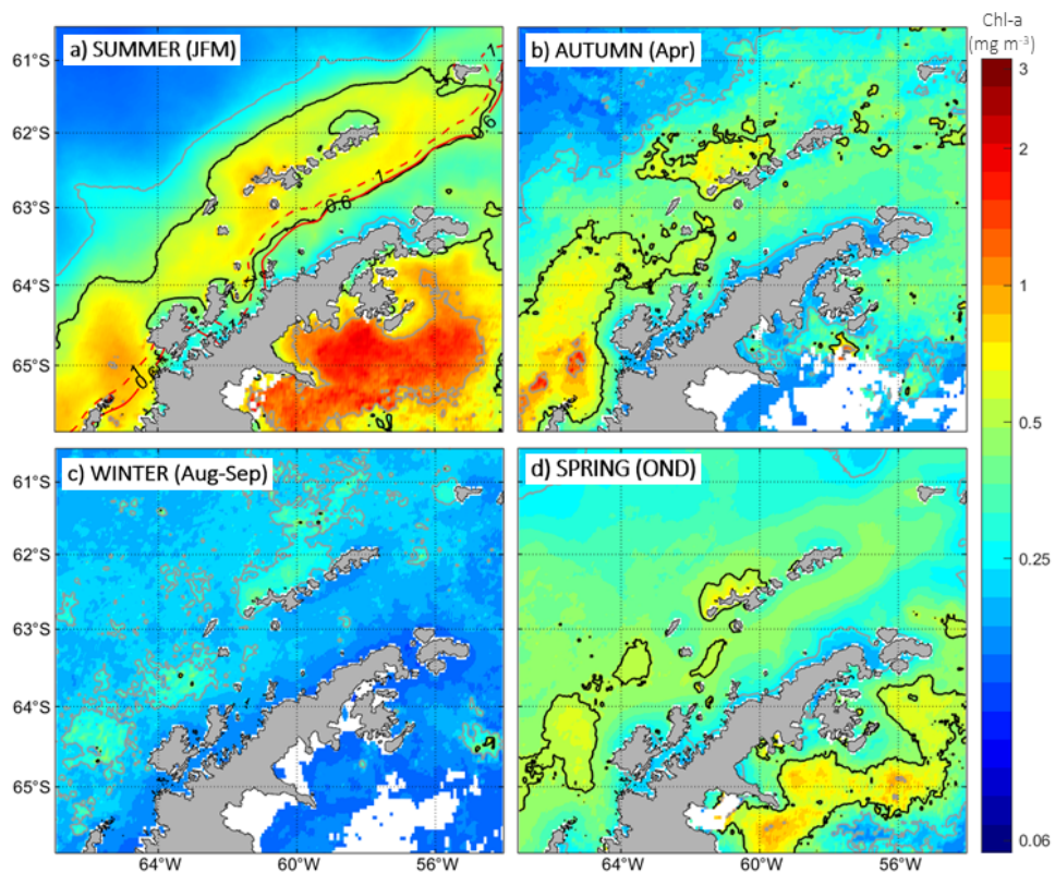
430 Figure 7. Same as Figure 5, but for chlorophyll-a concentrations (chl-a). Solid black lines indicate chl-a concentrations of 0.5 \text{ mg m}^{-3} , while solid grey lines represent chl-a concentrations of 0.25 and 1 \text{ mg m}^{-3} . Solid and dashed red lines in panel a) indicate 0.6^\circ\text{C} and 1^\circ\text{C} summer isotherms, respectively (see Figure 5a). For the autumn season (panel b), only the mean of April month is considered due to the absence of data during other months, which results from the presence of ice cover. Similarly, for the winter season (panel c), the mean of August and September months are solely considered for the same reason.
