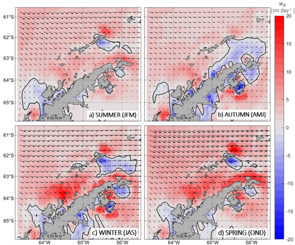
435 Figure 8. Same as Figure 5 but for Ekman pumping. Positive (negative) vertical velocities are indicated in shades of red (blue) and represent upwelling (downwelling) processes. Solid black lines refer to zero-velocities. Solid red and blue lines represent vertical velocities of 10 \text{ cm day}^{-1} and -10 \text{ cm day}^{-1} , respectively. Black vectors depict the wind stress. Wind stress reference vector is displayed over the southern AP with a value of 0.02 \text{ N m}^{-2} .
