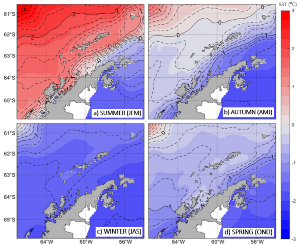
Figure 5. Seasonal maps of Sea Surface Temperature (SST; in shades of colours) for: a) summer, b) autumn, c) winter and d) spring. The capital letters between brackets stand for the initial letter of the month. The SST climatologies are averaged from January 1998 to December 2018. The dashed isotherms are plotted at intervals of 0.2^{\circ}\text{C} , while the solid line marks each 1^{\circ}\text{C} interval.
