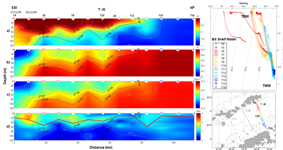
310 Figure 4. Same as in Figure 2 but for T-III, surveyed during the CIEMAR cruise (December 1999) and running from King George Island to the Antarctic Peninsula. Additionally, the dashed black line represents the isopycnal of 27.55 kg m -3 which is used as a reference more adjusted to our dataset to distinguish between TBW and TWW.
