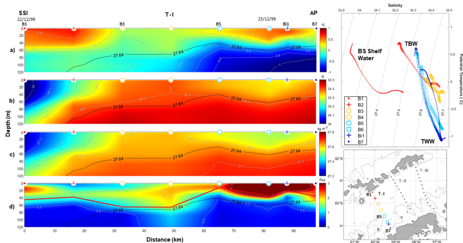
265 Figure 2. Vertical sections of ocean properties along transect T-I surveyed during the CIEMAR cruise (December 1999), running from Livingston Island to the Antarctic Peninsula. (a) Potential temperature, (b) salinity, (c) potential density, and (d) fluorescence are shown in the left-hand side panels. The solid black line represents the isopycnal of 27.64 kg m -3 , used as a reference to distinguish between Transitional Zonal Water with Bellingshausen influence (TBW) and Transitional Zonal Water with Weddell influence (TWW; Sangrà et al. , 2017). The solid red line in panel d) shows the upper mixed layer depth computed following Holte and Talley (2009). The top right-hand side panel displays a Temperature-Salinity diagram to highlight water masses: Bransfield Strait (BS) Shelf Water, TBW, and TWW. Different marks and colours are displayed to represent data in each station. The bottom right-hand side panel shows a map depicting the stations of the transect T-I.
