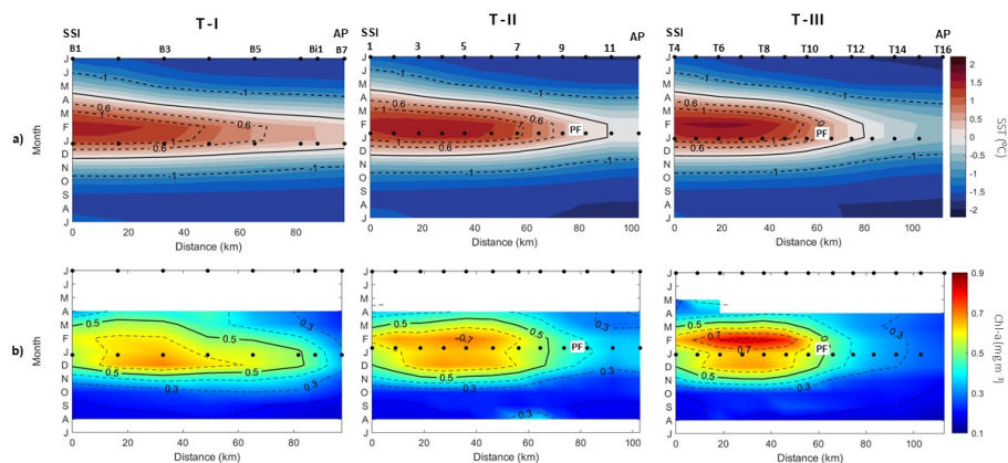
740 Figure 10. Monthly climatology from 1998 to 2018 of a) Sea Surface Temperature (SST), and b) chlorophyll-a (chl-a) concentration for each study transect (see Figures 2-4) from the South Shetland Islands (SSI) to the Antarctic Peninsula (AP). The black markers (dots) situated at the top of the subplots represent the station's positions along the transects. These same stations are also displayed during the summer months when the cruises were carried out. Additionally, the position of the Peninsular Front (PF), as identified during the cruises and located along the isopycnal of 27.55 kg m -3 , is also indicated.
