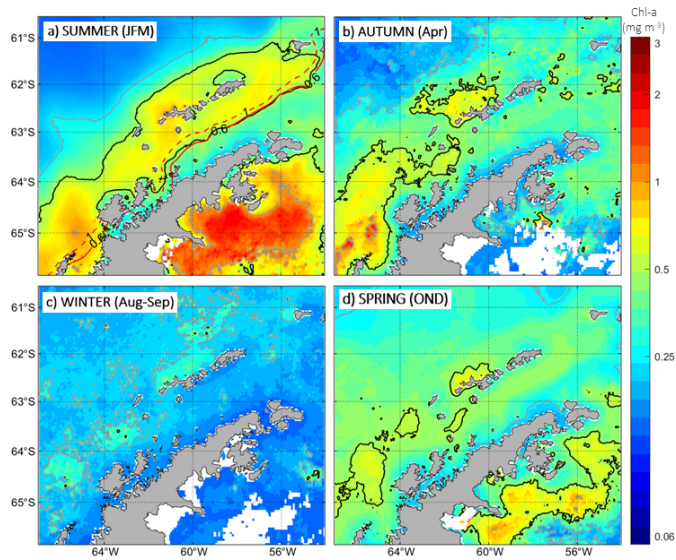
Figure 7. Same as Figure 5, but for chlorophyll-a concentrations (chl-a). Solid black lines indicate chl-a concentrations of 0.5 \text{ mg m}^{-3} , while solid grey lines represent chl-a concentrations of 0.25 and 1 \text{ mg m}^{-3} . Solid and dashed red lines in panel a) indicate 0.6^\circ\text{C} and 1^\circ\text{C} summer isotherms, respectively (see Figure 5a). For the autumn season (panel b), only the mean of April month is considered due to the absence of data during other months, which results from the presence of ice cover. Similarly, for the winter season (panel c), the mean of August and September months are solely considered for the same reason.
