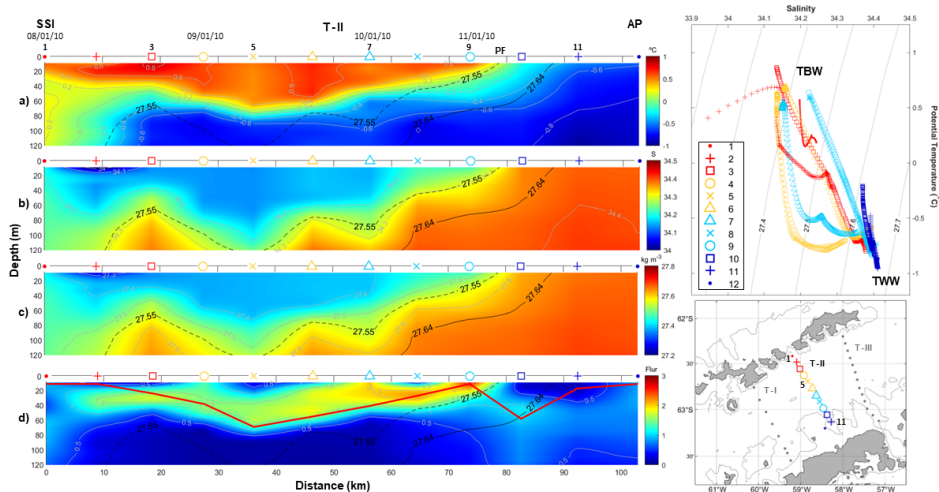
285 Figure 3. Same as in Figure 2 but for T-II, surveyed during the COUPLING cruise (January 2010) and running from Nelson Strait to the Antarctic Peninsula. Additionally, the dashed black line represents the isopycnal of 27.55 \text{ kg m}^{-3} which is used as a reference more adjusted to our dataset to distinguish between TBW and TWW.
