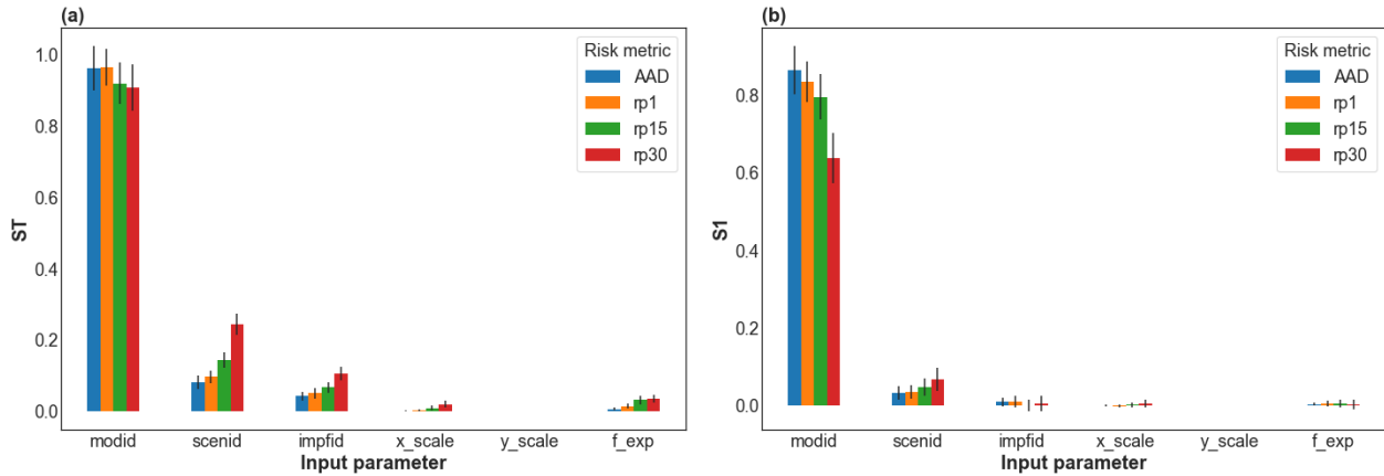
Figure B2. Total and first order Sobol' sensitivity indices (ST, S1) for the future-minus-historical change relative to the historical period ( \Delta climate-Delta Climate) in winter storm damage in Europe, comparing a future (2070-2100) to a historical period (1980-2010), and combining members from the climate models into single 90 years simulations. Panels (a) and (b) respectively show ST and S1 indices for the \Delta climate-Delta Climate change in average annual damage (AAD), and in damage amounts with return periods of one, 15, and 30 years (rp1, rp15, and rp30), aggregated over all exposure points of the entire European domain. The uncertainty factors (cf. sec. 2.6) are modid : climate model choice, scenid : future climate scenario choice, impfid : impact function choice, x_scale : impact function input intensity scaling factor, y_scale : impact function output MDD scaling factor, and f_exp : the exposure layer choice. The vertical black bars in (a) and (b) indicate the 95th percentile confidence intervals.
