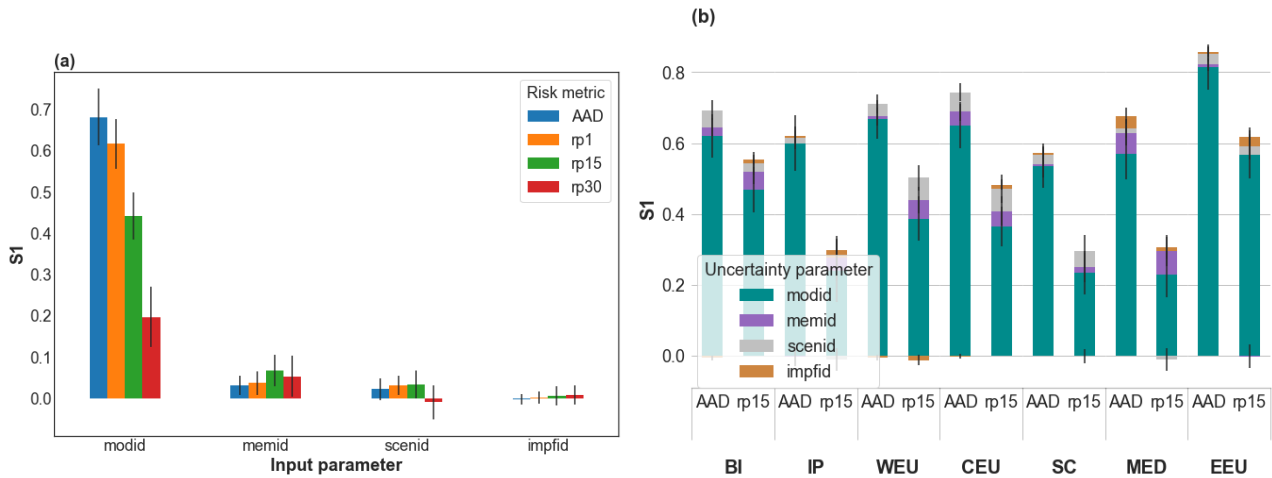
Figure 4. First order Sobol' sensitivity indices (S1) for the future-minus-historical change relative to the historical period ( delta-Climate-Delta Climate ) in winter storm damage in Europe, comparing a future (2070-2100) to a historical period (1980-2010). Panel (a) shows results for the delta-Climate-Delta Climate change in average annual damage (AAD), and in damage amounts with return periods of one, 15, and 30 years (rp1, rp15, and rp30), aggregated over all exposure points of the entire European domain; Panel (b) shows results for the delta-Climate-Delta Climate change in average annual damage (AAD), and in damage amount with a return periods of 15 years (rp15), aggregated over all exposure points in each of the seven regions defined in Fig. 2: British Isles (BI), Iberian Peninsula (IP), Western Europe (WEU), Central Europe (CEU), Mediterranean and Balkan region (MED), Scandinavia (SC), and Eastern Europe (EEU). The uncertainty factors (cf. sec. 2.6) are modid : climate model choice, memid : climate model member choice, scenid : future climate scenario choice, and impfid : impact function choice. The vertical black bars in (a) and (b) indicate the 95th percentile confidence intervals.
