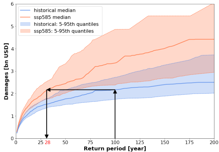
Figure 7. Exceedance Frequency Curves (EFCs) for future (2070–2100) SSP585 conditions, and historical (1980–2010) winter storm damage aggregated to the entire European domain. The EFCs are Each EFC is obtained using with an ensemble of opportunity approach, by combining the simulations 20 random subsamples of 20 years of data drawn from all the 30 a random subselection of 20 climate models. Bootstrapped distributions of the EFCs are derived to simulate the combined effects of internal variability and their ensemble members; climate model uncertainty. The damages are estimated using the impact function from Schwierz et al. (2010). The effects of internal variability on the EFCs are simulated by generating multiple EFCs via bootstrapping. Solid lines represent the medians, and dashed lines the 5th and 95th percentiles of the distributions of the multiple EFCs generated via bootstrapping. The arrows highlight that the intensity of a damage event with a return period of 100 years under historical climate conditions corresponds to the intensity of a damage event with a return period of 28 years under future SSP585 climate conditions.
