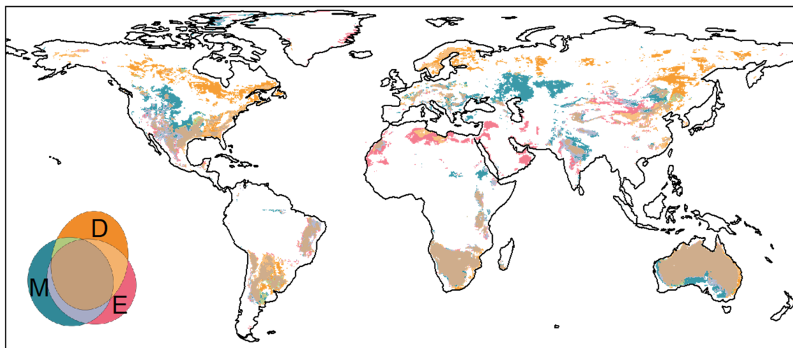
Figure 4: Two-legged metric analysis demonstrating the impact of different averaging periods on the assessment of coupling strength in summer (JJA and DJF for the North and the South Hemispheres, respectively). The diagnoses are based on the ERA5 (ECMWF ReAnalysis 5) reanalysis data from 1991 to 2020. The coupling strength between the sensible heat flux and p_{LCL} is estimated by the TLM algorithm (Dirmeyer et al., 2006). Strongly coupled regions (top 15% percentile of land grid cells) are diagnosed by using different time series (i.e., D: daytime-only mean; E: 24-hour entire-day mean; and M: monthly mean). The Euler diagram is employed to illustrate the spatial differences between the three diagnoses. The areas of colored components in the Euler diagram are proportional to the sizes of specific sets. (Modified from Yin et al., 2023.)
