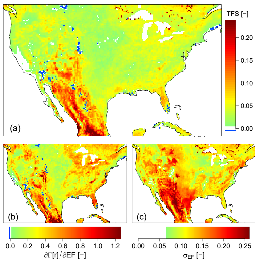
235 Figure 3: (a) The Triggering Feedback Strength (TFS; units of probability of afternoon (noon-6 pm) rain) in summer (JJA) based on ERA5 hourly data from 1991 to 2020. The TFS algorithm follows Findell et al. (2015) but with a ten-bin segmentation of daily evaporative fraction (EF). Positive values indicate the morning EF positively affects the probability of the occurrence of afternoon precipitation. (b) The mean value of the sensitivity term contributing to the TFS ( \partial\Gamma(r)/\partial EF ), thus the mean sensitivity of afternoon rainfall to morning-time surface flux partitioning. (c) The variability term contributing to the TFS: the standard deviation of EF.
