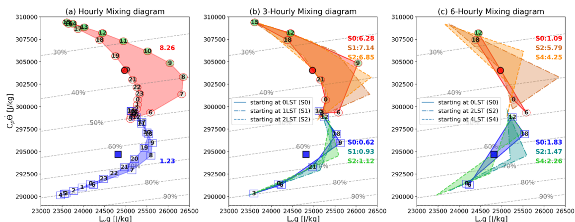
275 Figure 5: (a) The hourly mixing diagrams in water- (red) and energy- (blue) limited flux tower sites exhibits the coevolution of moisture (x axis) and thermal (y axis) energy content per unit mass within the BL (Modified from Fig. 5d in Seo and Dirmeyer, 2022). The marks are shaded by the color determined by two-legged couplings corresponding to the local hour (referring to Fig. 5a in Seo and Dirmeyer, 2022). The black edged circle and square are the mean of the 24-hourly values in water- and energy-limited regimes, respectively. The colored numbers are the area within the curves (multiply displayed value by 10^6 ; units: [\text{J}/\text{kg}]^2 ); these 280 values quantify the diurnal energetic asymmetry captured by each mixing diagram. Dashed black lines are lines of constant humidity. Note that x- and y-axis ranges differ. (b) The 3-hourly mixing diagrams in both climate regimes, computed with three different starting times: hour 0 (S0: solid), hour 1 (S1: dashed dot), and hour 2 (S2: dashed) LST. (c) The 6-hourly mixing diagrams as in (b), but with starting times at hours 0, 2, and 4 LST.
