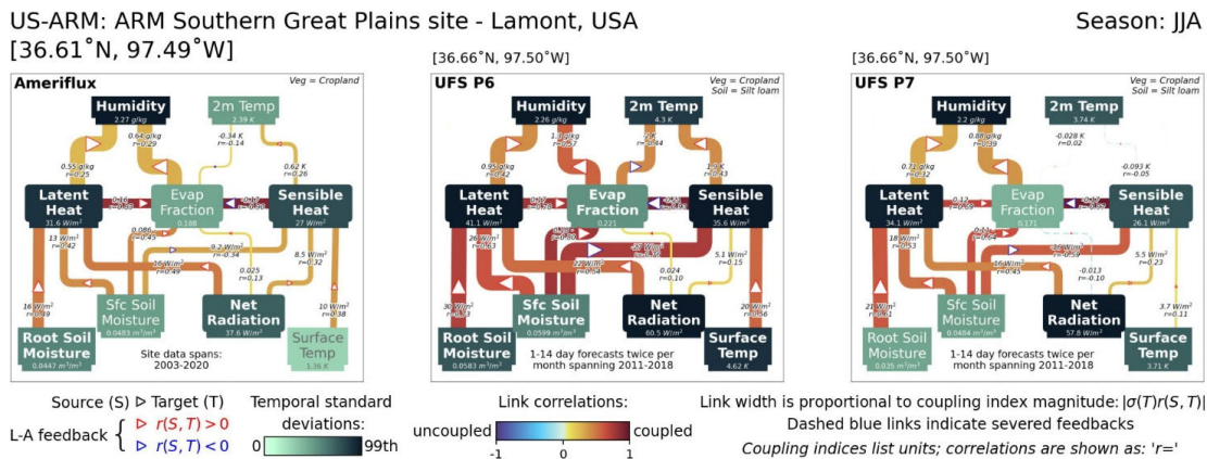
Figure 2: Land-atmosphere coupling pipe diagrams demonstrating the complexity of land-atmosphere interactions, the need for more than one measure to assess coupling, and some of the potential inadequacies of modelled coupling at this example location. (Taken from http://cola.gmu.edu/dirmeyer/ufs/P6vP7_locos_chains_AMX.html )
