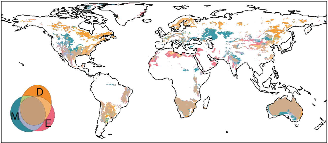
300 Figure 4: Two-legged metric analysis demonstrating the impact of different averaging periods on the assessment of coupling strength in summer (JJA and DJF for the North and the South Hemispheres, respectively). The diagnoses are based on the ERA5 (ECMWF ReAnalysis 5) reanalysis data from 1991 to 2020. The coupling strength between the sensible heat flux and p_{LCL} is estimated by the TLM algorithm (Dirmeyer et al., 2006). Strongly coupled regions (top 15% percentile of land grid cells) are diagnosed by using different time series (i.e., D: daytime-only mean; E: 24-hour entire-day mean; and M: monthly mean). The Euler diagram is employed to illustrate the spatial differences between the three diagnoses. The areas of colored components in the Euler diagram 305 are proportional to the sizes of specific sets. (Modified from Yin et al., 2023.)
