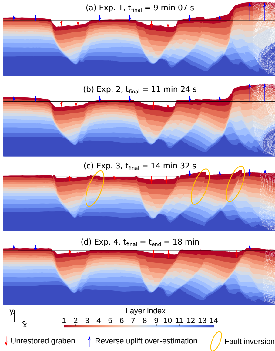
Figure 14. Results of experiments 1 to 4 (Fig. 12) to find the effective material properties inside the analogue model. For each experiment, t_{\text{final}} is the restoration time at which the simulation is stopped, and for which the model is shown. t_{\text{end}} is the time at the end of the restoration of the first layer. The black line on each result is the expected position of the topography at the end of the restoration of the first layer.
