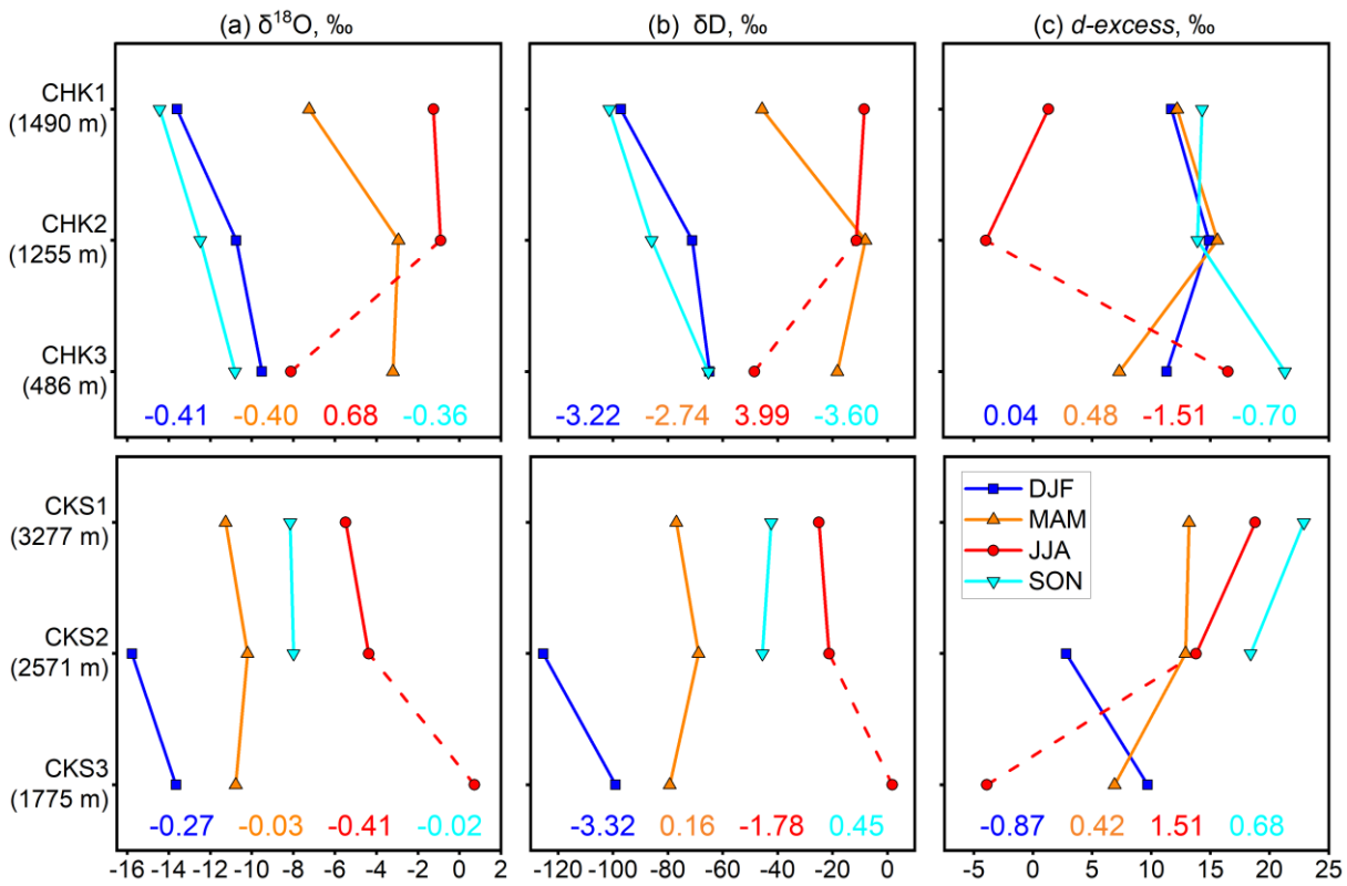
325 Figure 3: Changes with elevation in (a) \delta^{18}\text{O} , (b) \delta\text{D} , and (c) d\text{-excess} by season in CHK (upper panel) and CKS (bottom panel). Dashed lines indicate small number of samples and low precipitation per event in CHK3 and CKS3. Numbers show seasonal values of elevational gradients ( \text{‰} per 100 m).
