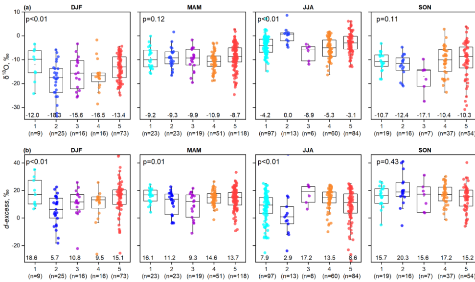
445 Figure 7: Seasonal values of (a) \delta^{18}\text{O} and (b) d-excess according to the trajectory clusters. Numbers along the X-axes show the number of events in each group and season.
