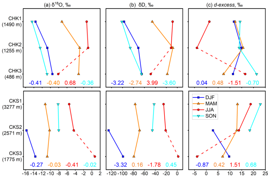
Figure 3: Changes with elevation in (a) \delta^{18}\text{O} , (b) \delta\text{D} , and (c) d -excess by season in CHK (upper panel) and CKS (bottom panel). Dashed lines indicate small number of samples and low precipitation per event in CHK3 and CKS3. Numbers show seasonal values of elevational gradients (‰ per 100 m).
