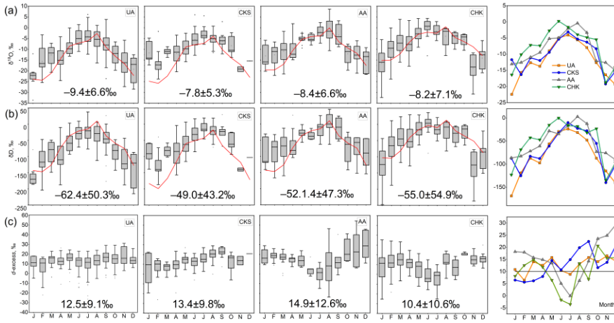
Figure 2: Boxplots of (a) \delta^{18}O , (b) \delta D , and (c) d\text{-excess} in precipitation collected at the four catchments (see Fig. 1 and Table 1 for locations of catchments and number of samples) between 2019 and 2021 (left panel) and mean monthly d\text{-excess} values (right panel). Precipitation was sampled at three sites in CHK and CKS and data from all sites are included. Annual mean values \pm standard deviation calculated for the 2019 – 2021 period are shown. The horizontal line in (c; right panel) shows the global mean d\text{-excess} (10‰). The red line shows data from the Waterisotopes Database (Bowen, 2022). The Waterisotopes Database data were averaged over all sampling locations in CKS and CHK.
