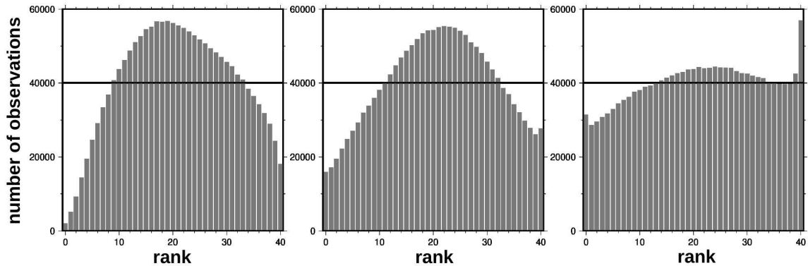
Figure 3. Rank histograms corresponding to the prior ensemble (left panel) and to the posterior ensemble, as obtained with the LETKF algorithm (middle panel) and the MCMC sampler (right panel). For the posterior ensembles, the histograms aggregate ranks from two simulations, one conditioned on observations from the odd days only, which is validated using observations from the even days, and another one conditioned on observations from the even days only, which is validated using observations from the odd days.
