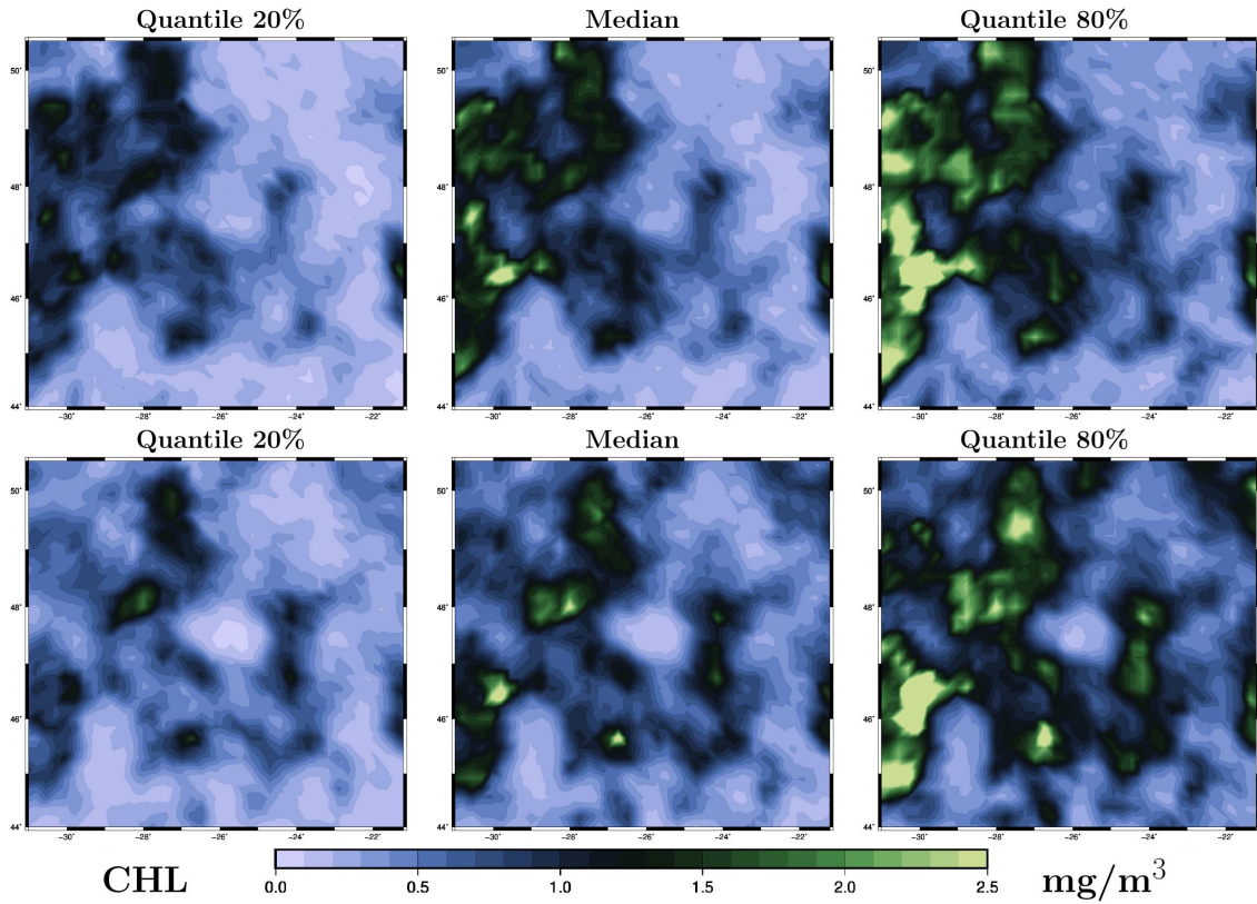
Figure 7. Ensemble forecast obtained with the LETKF algorithm for surface chlorophyll concentration (in \text{mg}/\text{m}^3 ) on May 26, 2009. The figure displays 3 quantiles (20%, 50% and 80%) of the marginal ensemble distributions, as obtained for the 1-day forecast (top panels) and the 4-day forecast (bottom panels). X-axis and Y-axis represent longitude and latitude, respectively.
