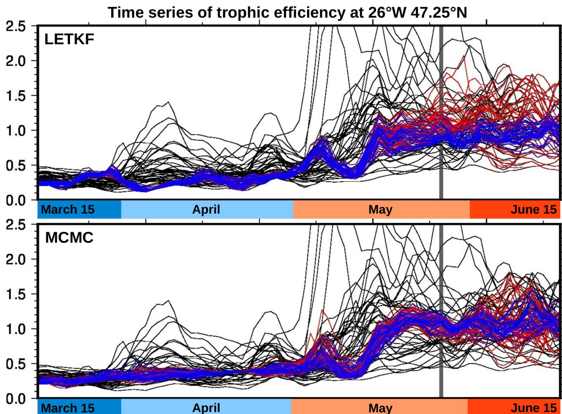
Figure 12. Timeseries of trophic efficiency. At 26^{\circ}\text{W} , 47.25^{\circ}\text{N} . With the LETKF algorithm (top) and the MCMC sampler (bottom). Prior (black), analysis (blue), forecast (red).
