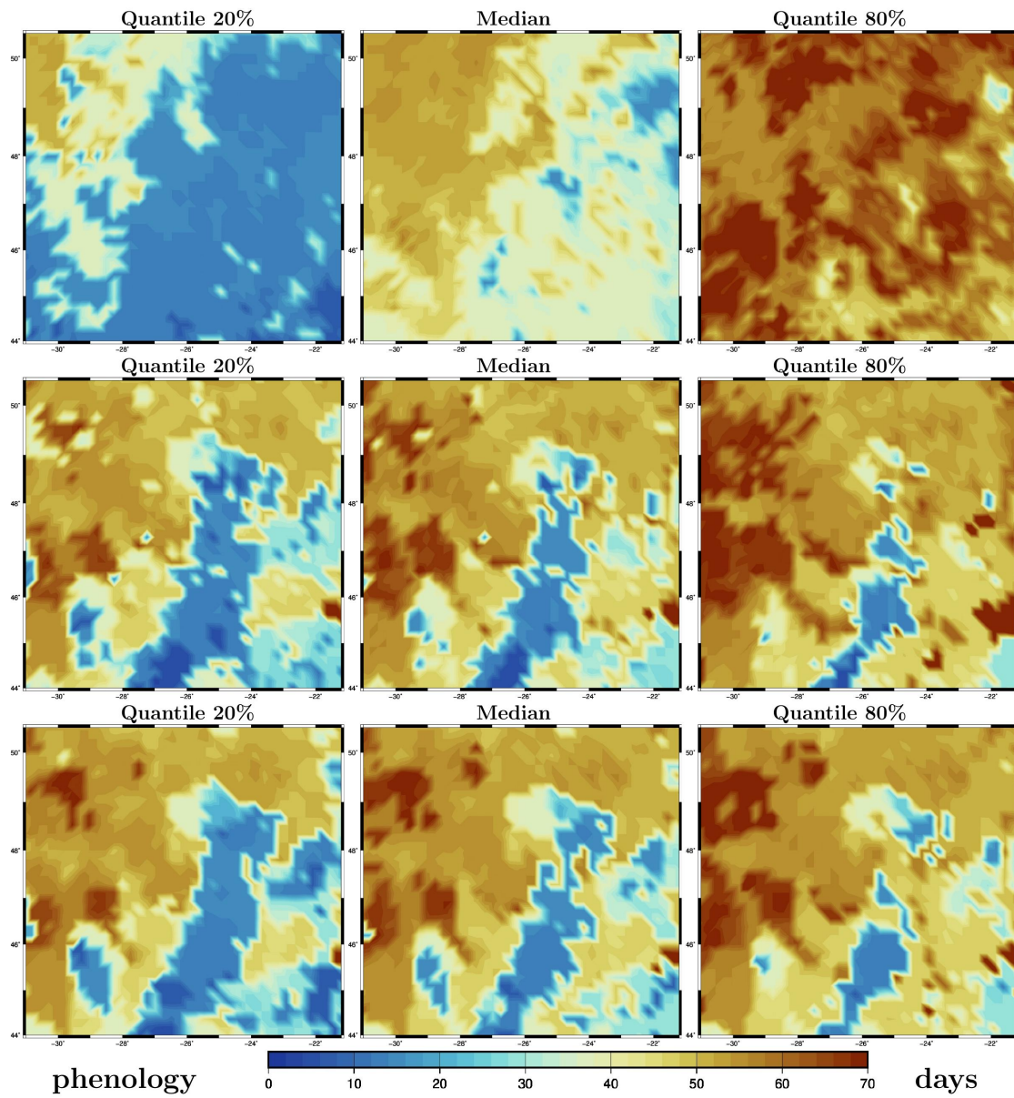
Figure 9. Quantiles of phenology (in days). Prior ensemble (top), LETKF analysis (middle) and MCMC sampler analysis (bottom). X-axis and Y-axis represent longitude and latitude, respectively.
