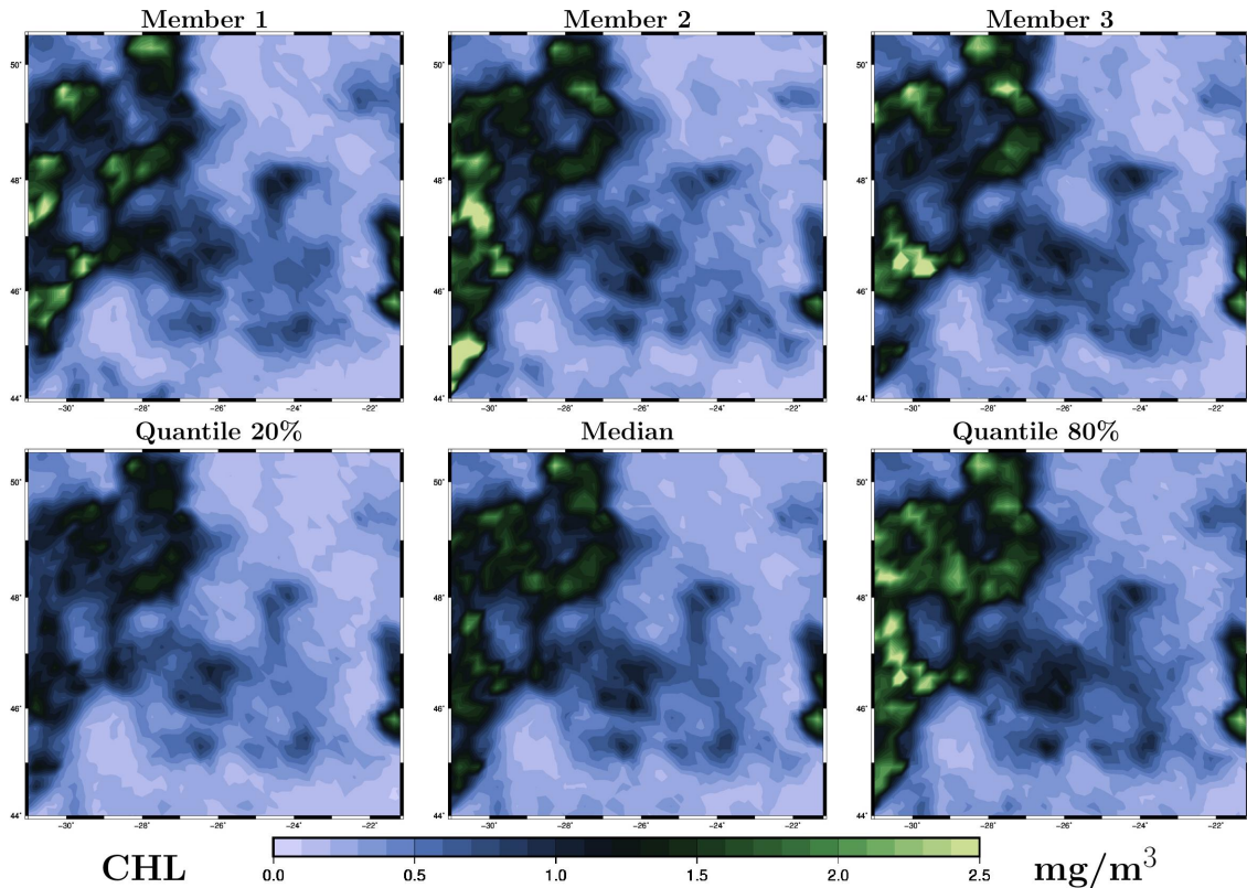
Figure 5. Ensemble analysis obtained with the LETKF algorithm for surface chlorophyll concentration (in \text{mg}/\text{m}^3 ) on May 26, 2009. The figure displays 3 members of the ensemble (top panels) and 3 quantiles (20%, 50% and 80%) of the marginal ensemble distributions (bottom panels). X-axis and Y-axis represent longitude and latitude, respectively.
