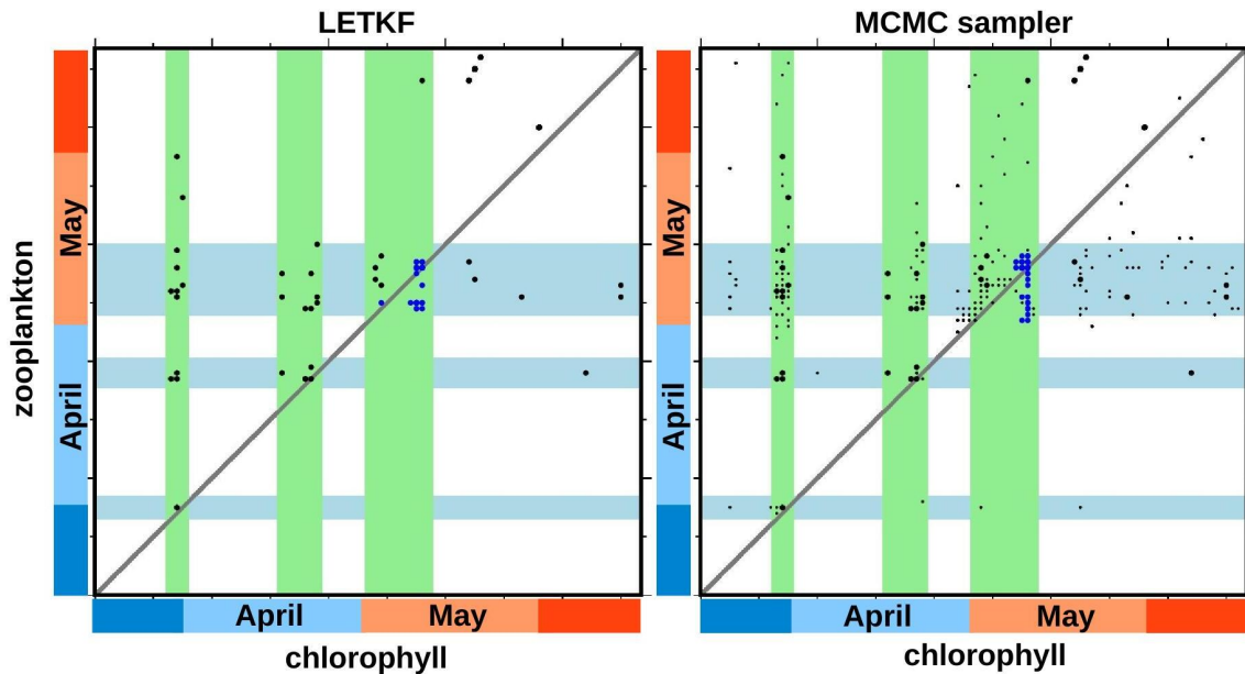
Figure 10. Scatterplot of phenology (in days) for chlorophyll (x-axis) and zooplankton (y-axis). At 26°W, 47.25°N. With the LETKF algorithm (left) and the MCMC sampler (right). Prior ensemble (black), augmented prior (small black dots), analysis (blue).
