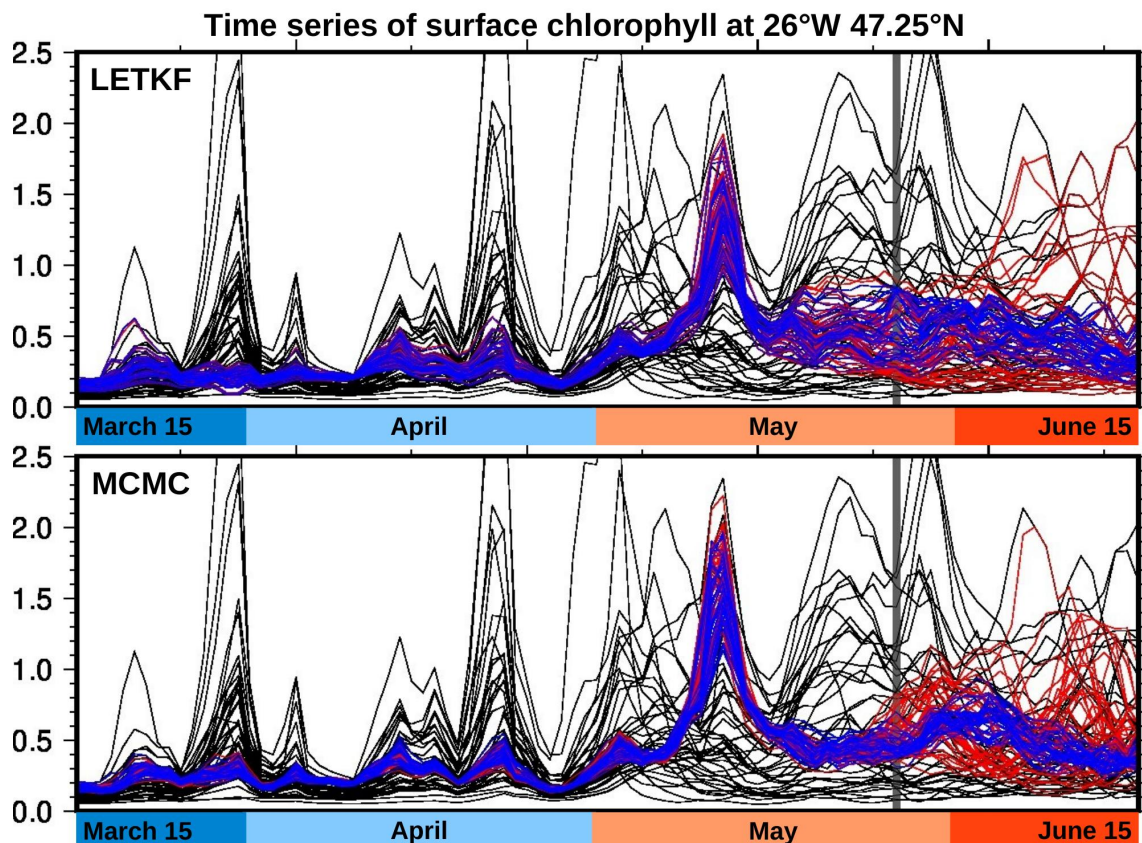
Figure 4. Ensemble surface chlorophyll time series at 26^{\circ}\text{W} , 47.25^{\circ}\text{N} . The black curves represent 40 members of the prior ensemble (as produced by the NEMO/PISCES simulator), the blue curves represent 40 members of the ensemble analysis (using observations for the entire period), and the red curves represent 40 members of the ensemble forecast (using only observations until May 25). The forecast thus starts on May 25 (vertical grey line). These results are shown for the LETKF algorithm (top panel) and the MCMC sampler (bottom panel).
