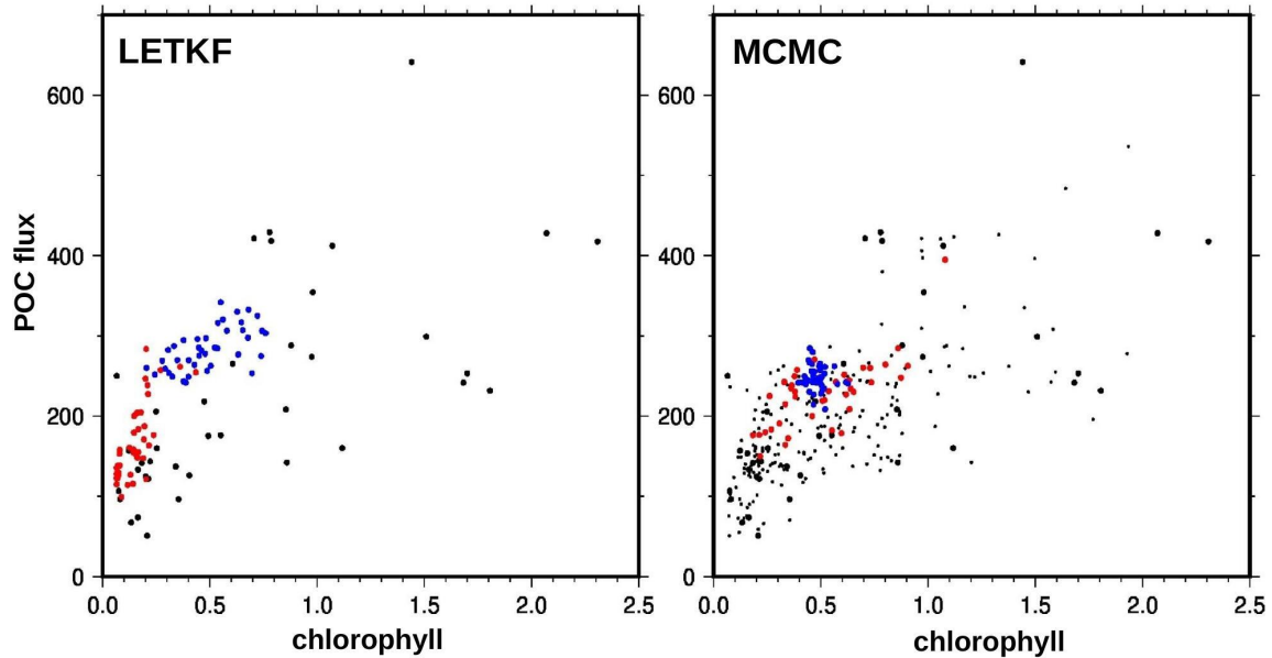
Figure 13. Scatterplot of surface chlorophyll concentration (in \text{mg}/\text{m}^3 ) vs POC flux at 100 m depth (in \text{mg C}/\text{m}^2/\text{day} ). At 26^\circ\text{W} , 47.25^\circ\text{N} , on May 26, 2019. With the LETKF algorithm (left) and the MCMC sampler (right). Prior (black), augmented prior (small black dots), analysis (blue), 4-day forecast (red).
