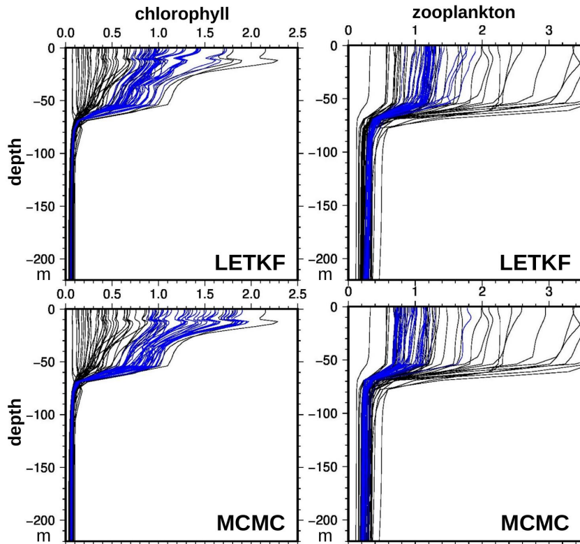
Figure 11. Vertical profile of chlorophyll (in \text{mg}/\text{m}^3 , left) and microzooplankton (in \text{mmol-C}/\text{m}^3 , right). At 26^\circ\text{W} , 47.25^\circ\text{N} . May 8, 2019. With the LETKF algorithm (top) and the MCMC sampler (bottom). Prior ensemble (black), analysis (blue).
