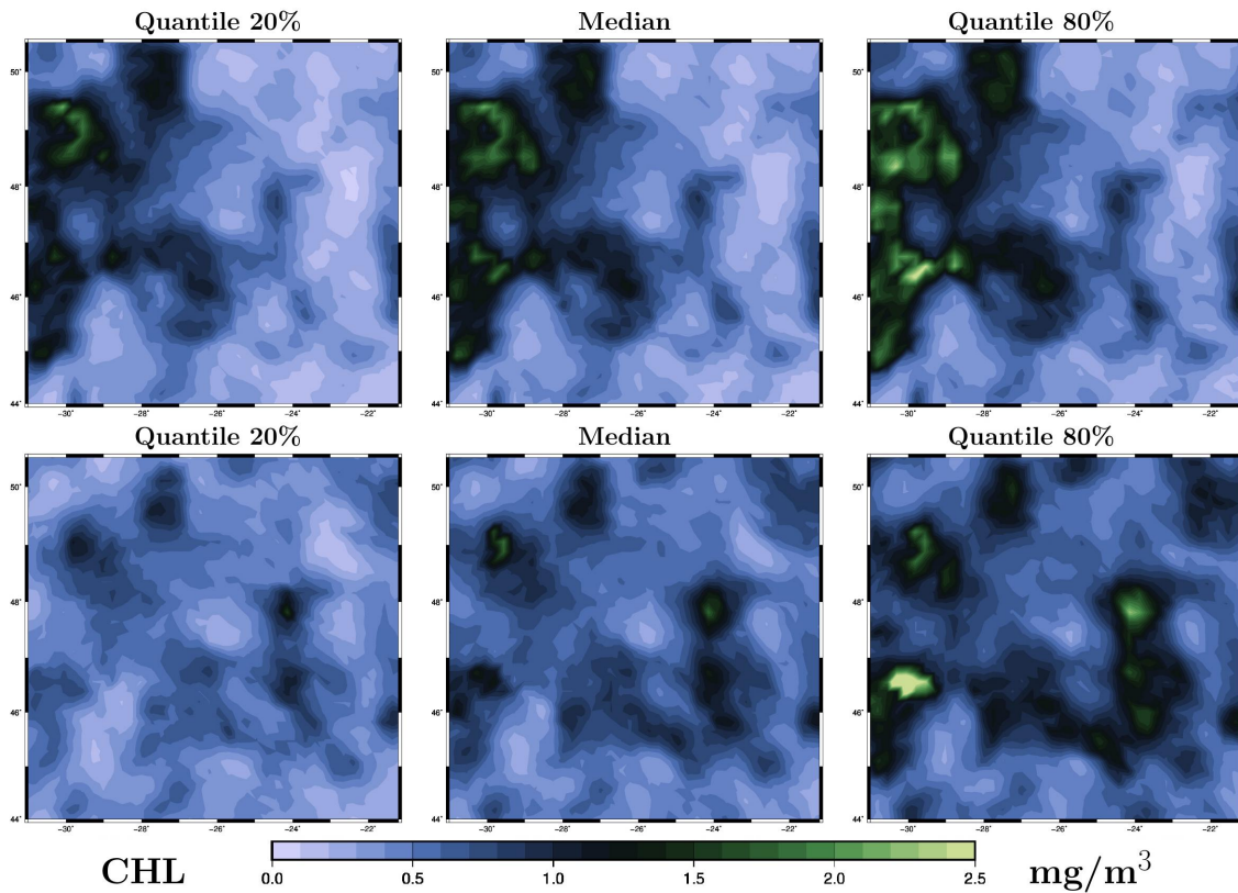
Figure 8. Ensemble forecast obtained with the MCMC sampler for surface chlorophyll concentration (in \text{mg}/\text{m}^3 ) on May 26, 2009. The figure displays 3 quantiles (20%, 50% and 80%) of the marginal ensemble distributions, as obtained for the 1-day forecast (top panels) and the 4-day forecast (bottom panels). X-axis and Y-axis represent longitude and latitude, respectively.
