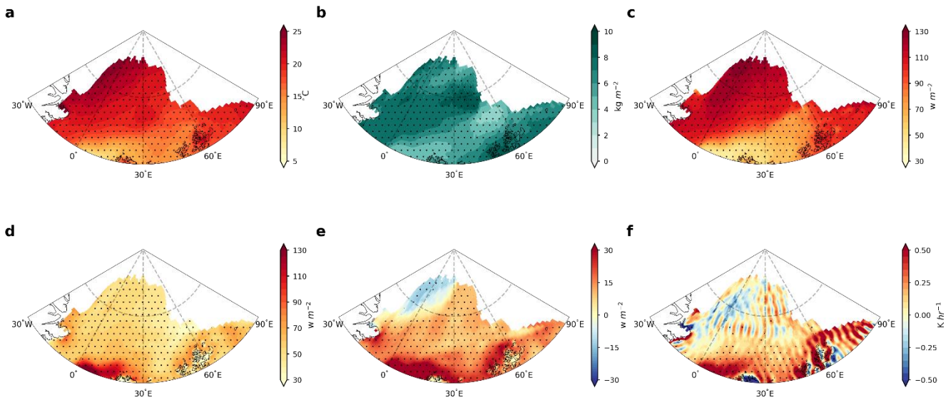
775 Figure 5. Spatial distribution of the mean anomalies of (a) T2m, (b) column-integrated water vapor (IWV), (c) downward longwave radiation (DLW), (d) sensible heat flux (SHF), (e) latent heat flux (LHF) and (f) horizontal temperature advection averaged over all hours with T2m \geq 0 °C over a grid point. Positive values in (d) and (e) indicate fluxes directed from the atmosphere toward the surface. Stippled areas indicate that anomalies are significant at the 0.05 level based on the Student's t-test.
