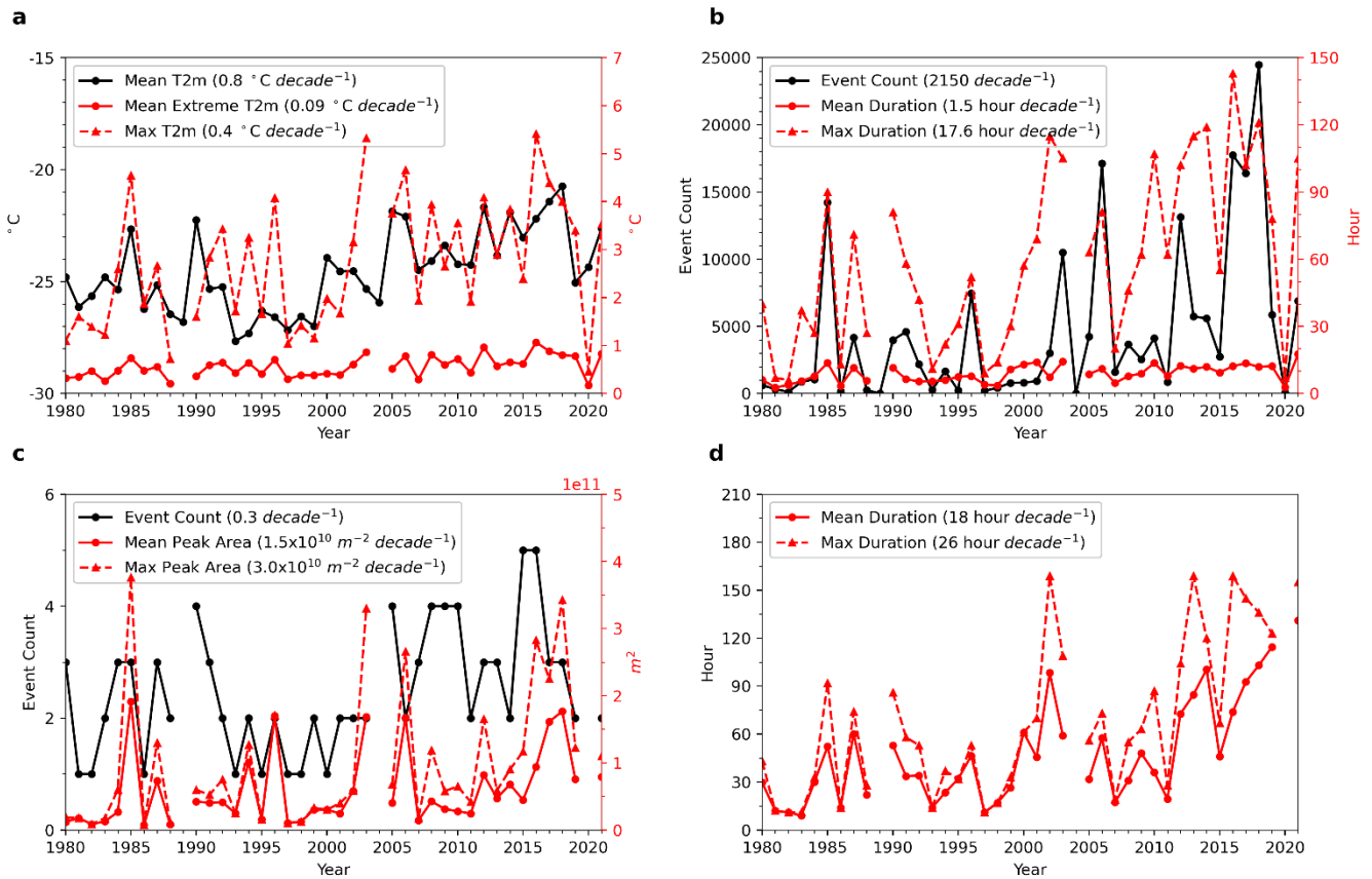
855 Figure 15. Trends in (a) the area-weighted spatial mean T2m over the entire high Arctic (black solid line with circles), mean T2m only for grid points above 0°C (red solid line with circles) and the seasonal maximum hourly T2m (red dashed line with triangles) over the high Arctic. (b) is the same as (a), but for the trends in extreme warming event count (black solid line with circles), mean event duration (red solid line with circles) and seasonal maximum event duration (red dashed line with triangles). (c) and (d) show trends in the characteristics of the 96 concurrent warming events identified in Section 3.3. Trends in (c) the event count (black solid line with circles), mean peak area (solid 860 red line with circles) and seasonal maximum peak area (red dashed line with triangles) of the concurrent warming events. (d) shows the mean duration (red solid line with circles) and seasonal maximum duration (red dashed line with triangles) of the concurrent warming events. For those seasons with only one concurrent warming event, the mean peak area would be the same as the maximum peak area in (c) and the mean duration would be the same as the maximum duration in (d). All trends are significant at the 0.05 level based on the Student's t-test.
