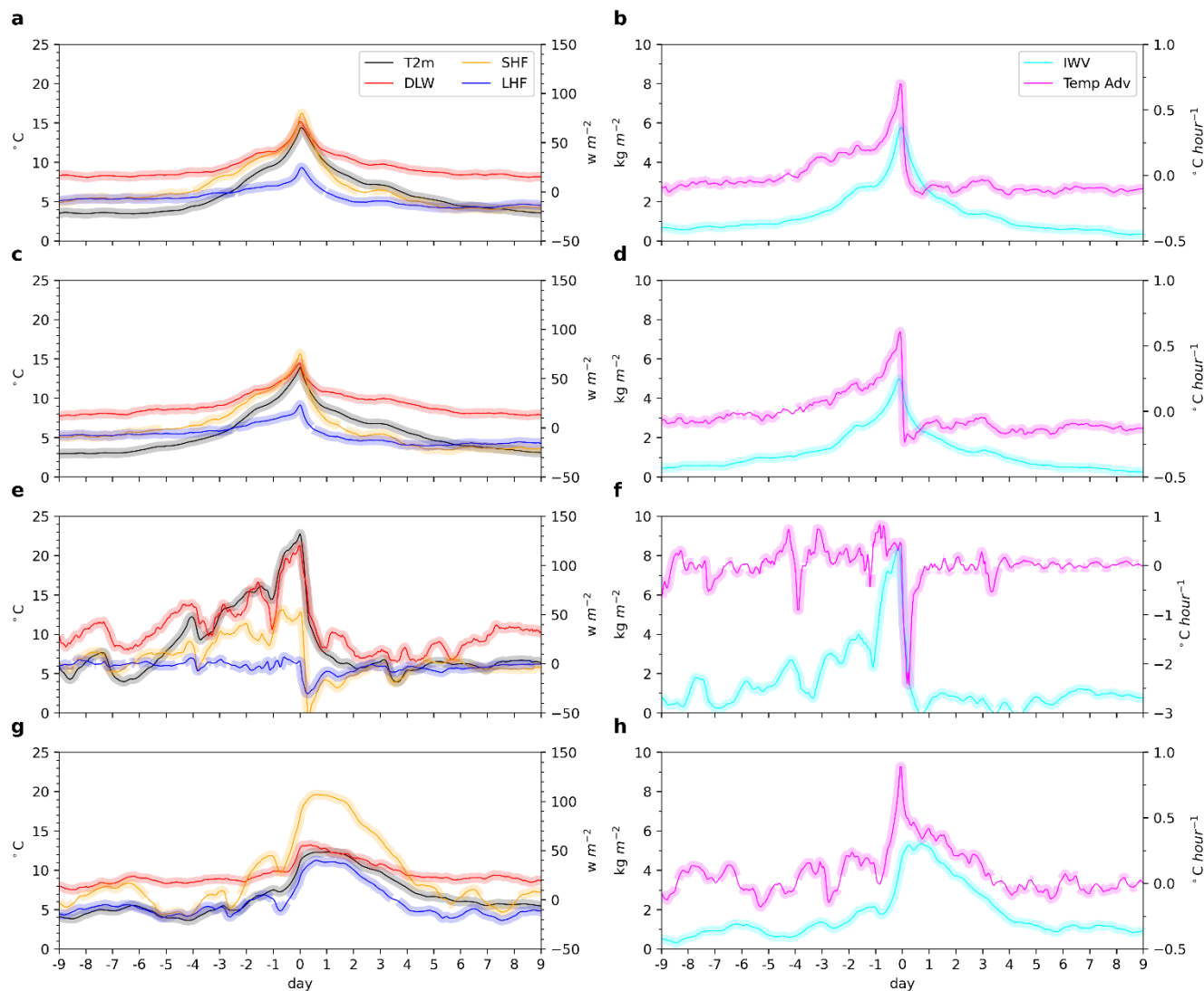
Figure 6. Temporal evolution of the anomalies of T2m, DLW, SHF, LHF, IWV and temperature advection for all the extreme warming events defined as any grid points with T2m \geq 0^\circ\text{C} (a, b), short duration events (i.e., grid points with T2m \geq 0^\circ\text{C} for 1 hour) equatorward of 83^\circ\text{N} (c, d), short duration events poleward of 85^\circ\text{N} (e, f), and long duration events (i.e., grid points with T2m \geq 0^\circ\text{C} for at least 40 hours; 790 (g, h). Note that long duration events occur only over regions equatorward of 83^\circ\text{N} . These curves are constructed by averaging the temporal evolution of various anomaly terms across all extreme warming events within the respective groups. There are 191555, 18586, 1642, and 10097 events included in the groups of all events, short duration events equatorward of 83^\circ\text{N} , short duration events poleward of 85^\circ\text{N} and long duration events, respectively. Day 0 corresponds to the start of an extreme warming event when a grid point's T2m first exceeds 0^\circ\text{C} . The shading indicates that the anomalies are significant at the 0.05 level based on the Student's t-test.
