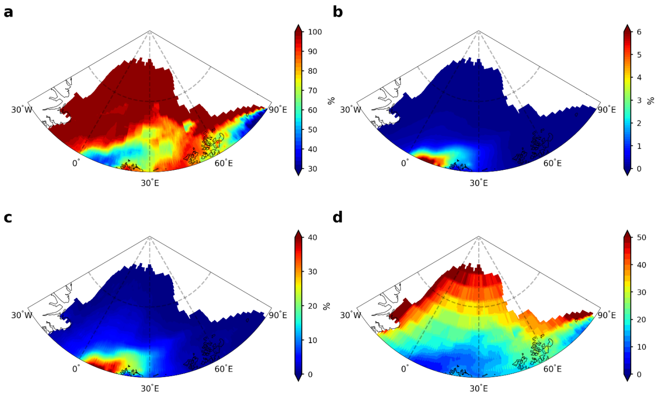
835 Figure 13. Spatial distribution of (a) the fraction of extreme warming events defined as a grid point with T_{2m} \geq 0^\circ\text{C} that occurs during AR days, (b) the fraction of time for all winter hourly snapshots from 1979-2021 with T_{2m} above 0^\circ\text{C} , (c) the fraction of time for all AR day hourly snapshots from 1979-2021 with T_{2m} above 0^\circ\text{C} , and (d) the risk ratio, which is calculated by dividing (c) by (b).
