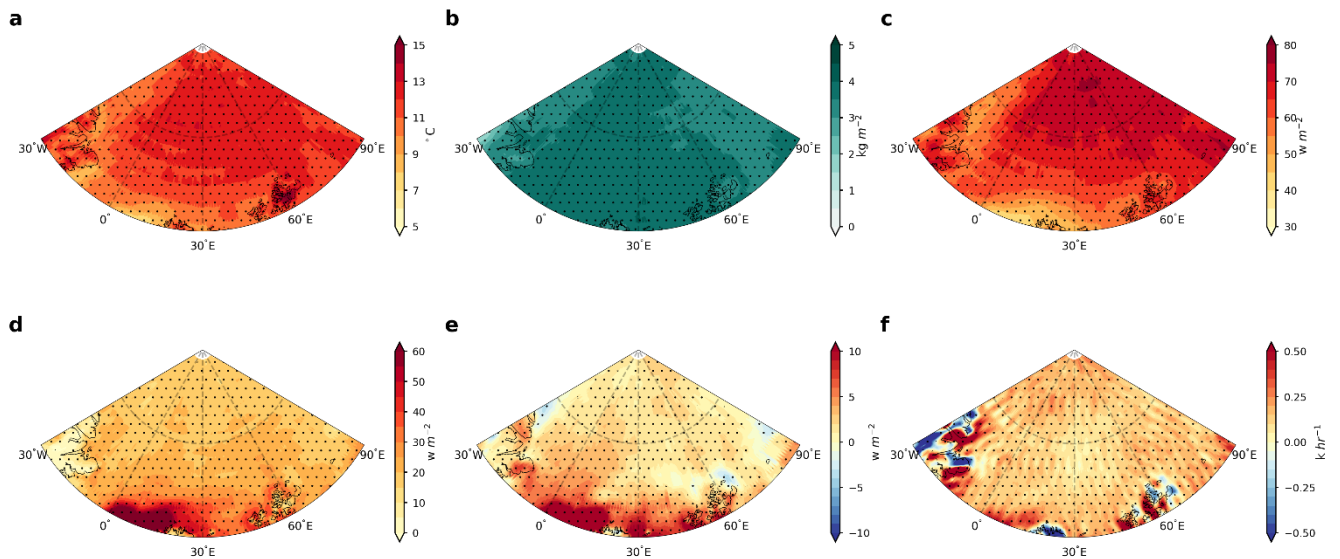
830 Figure 12. Spatial distribution of the anomalies of (a) T2m, (b) IWV, (c) DLW, (d) SHF, (e) LHF and (f) temperature advection during AR days. Stippled areas indicate anomalies are significant at the 0.05 level based on the Student's t-test.
