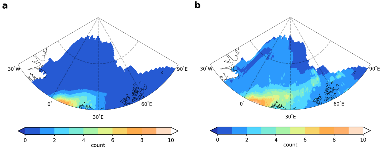
760 Figure 3. Spatial distribution of (a) the seasonal mean event count for all winters and for (b) only those winters with at least one extreme 765 warming event from 1979-2021.
