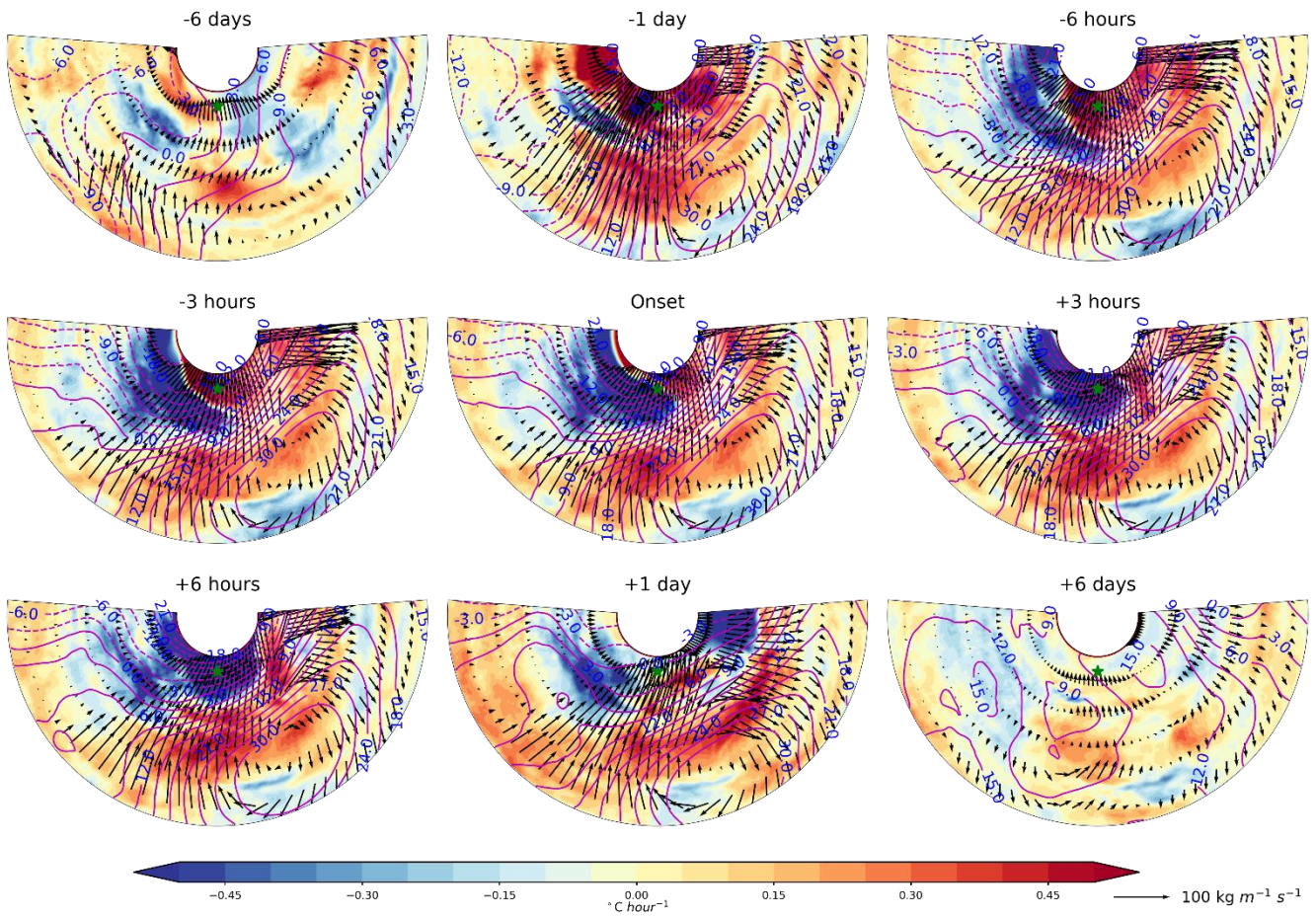
Figure 8. Same as Fig. 7, but for the short duration events ( i.e. , grid points with T_{2m} \geq 0^{\circ}\text{C} for 1 hour) poleward of 85^{\circ}\text{N} . Regions 2^{\circ} poleward, 20^{\circ} equatorward, 100^{\circ} westward/eastward of the event grid point are included in the composites.
