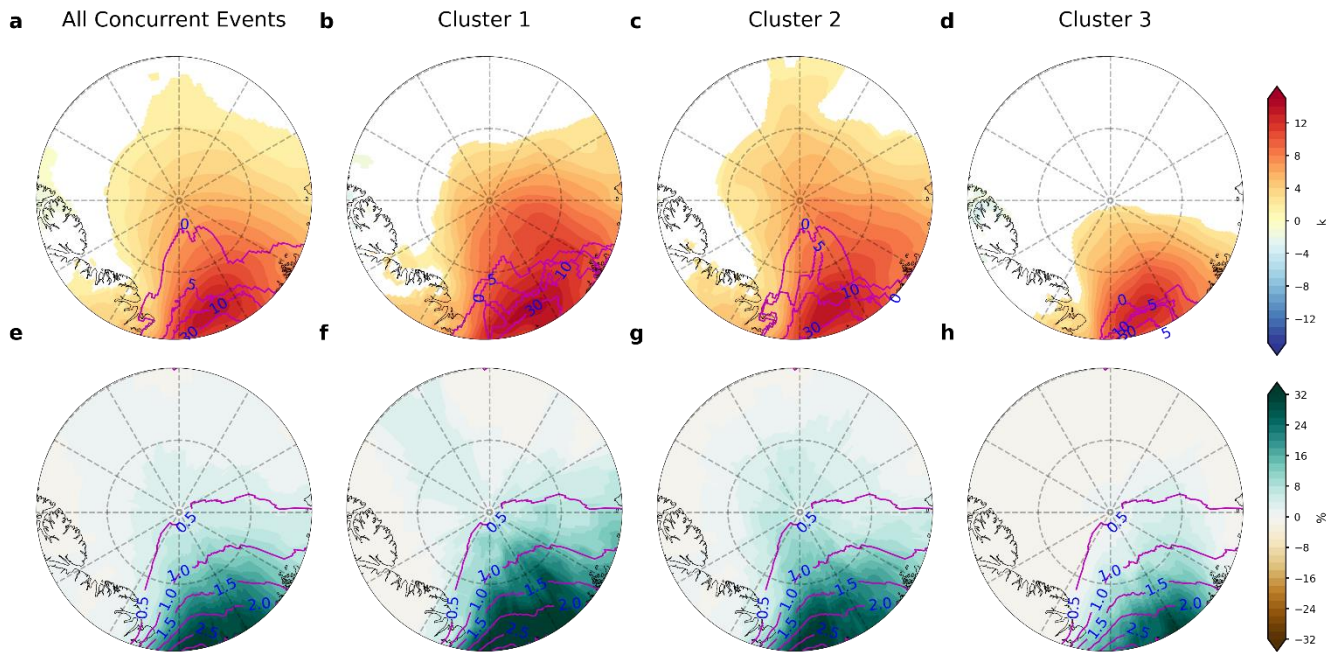
825 Figure 11. Same as Fig. 10, but for the T2m anomalies and AR frequency during the peak of the concurrent warming events. The peak of the concurrent warming events is defined as the time when the areas with temperature above 0°C reach maximum. The purple line contours in (a)-(d) depict the fraction of time when the T2m over a grid point reaches or exceeds 0°C during the peak of the concurrent warming events and (e) – (h) the climatology of winter AR frequency.
