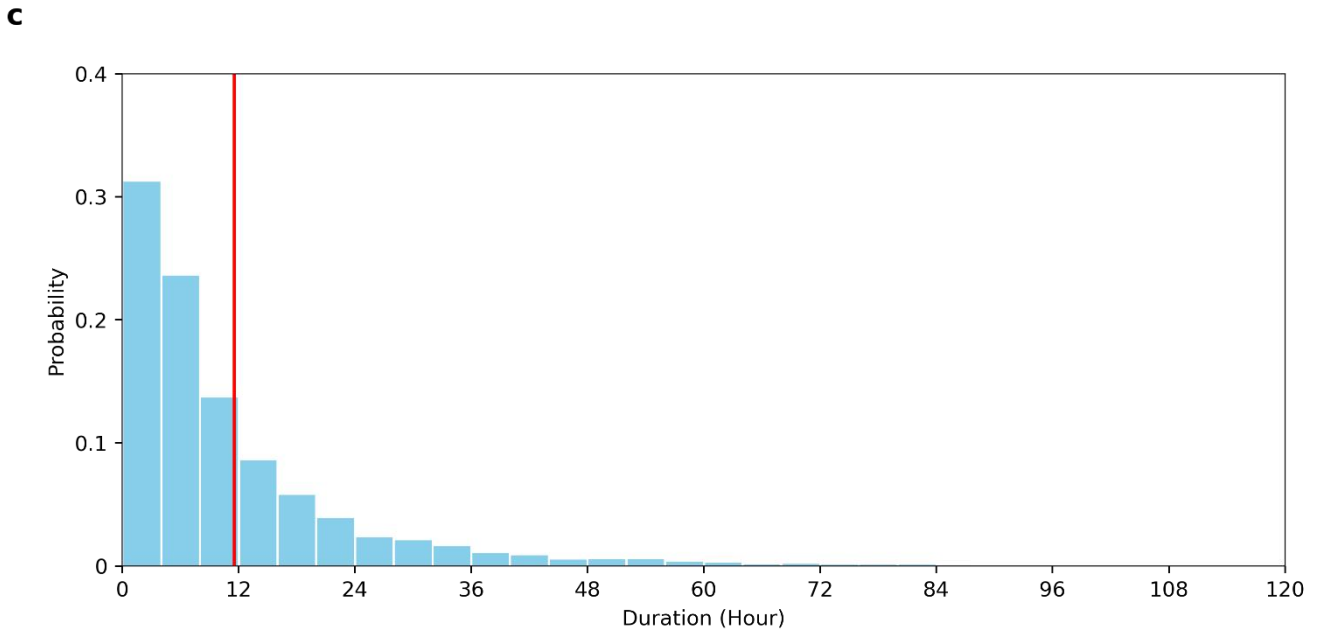
Figure 2. Spatial distribution of the (a) mean duration and (b) extreme duration of the high Arctic extreme warming events defined as a grid point with T2m \geq 0^{\circ}\text{C} . Extreme duration is defined as the local 95 th percentile of the duration distribution. (c) Probability density function of the duration distribution for all events happened during winter from 1979 to 2021. The red vertical line in (c) marks the mean of the distribution (11.55 hours).
