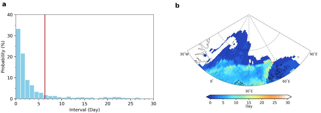
770 Figure 4. (a) Probability density function of the time interval between the termination of an extreme warming event ( i.e., time when a grid point's T2m first falls below 0°C ) and the start of the following extreme warming event ( i.e., time when a grid point's T2m first exceeds 0°C ) over the same grid point. (b) Spatial distribution for the mean time interval. Grid points never experienced an extreme warming event
