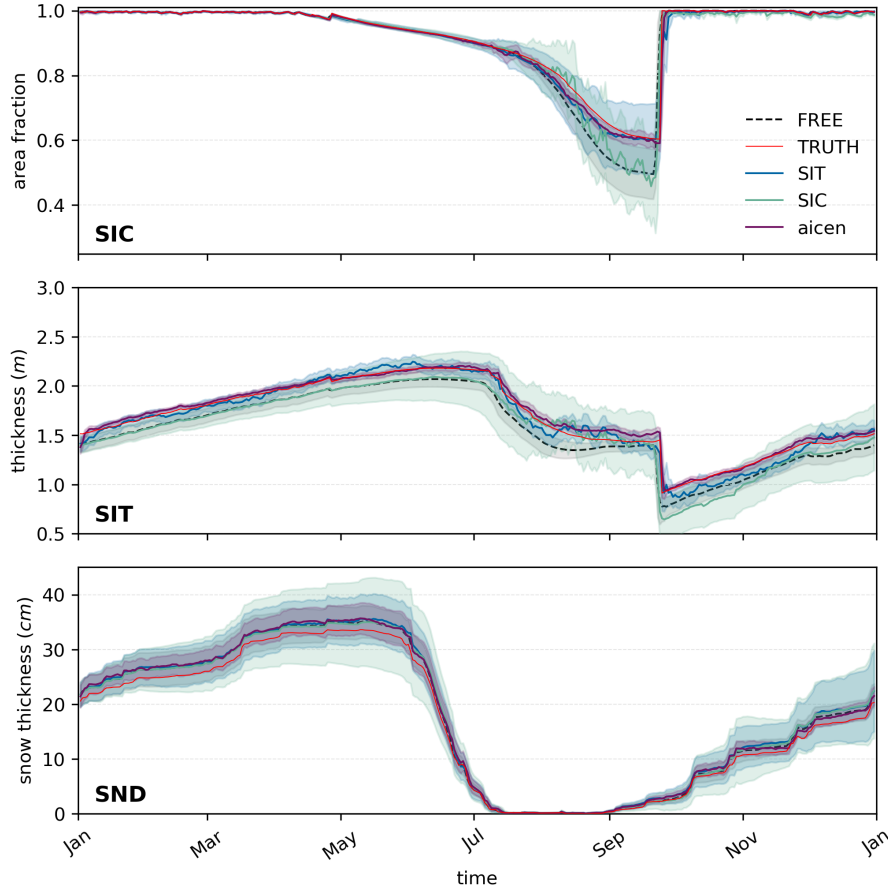
Figure 5. Assimilating with bounded algorithms. Same as Fig. 4 but for case in which observations are assimilated using the f101_BNRH (fully bounded) filter.
