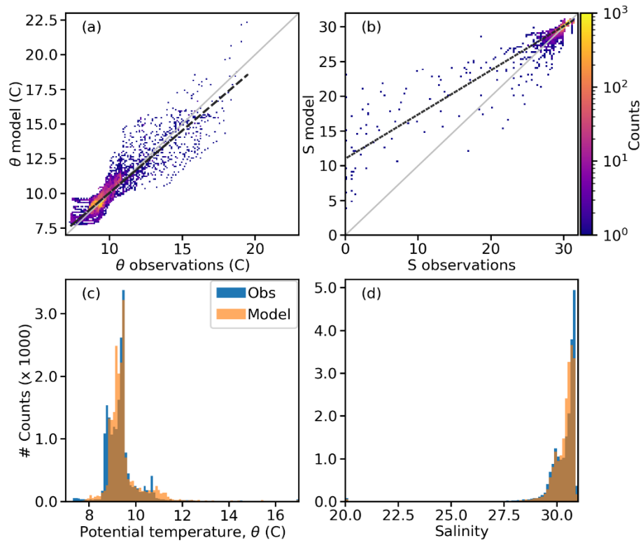
Figure 2. Two-dimensional histograms for (a) potential temperature and (b) salinity; the gray line shows the 1:1 slope and the dashed black line, the linear regression fit. Overlapped model and observed histograms for (c) potential temperature and (d) salinity.
