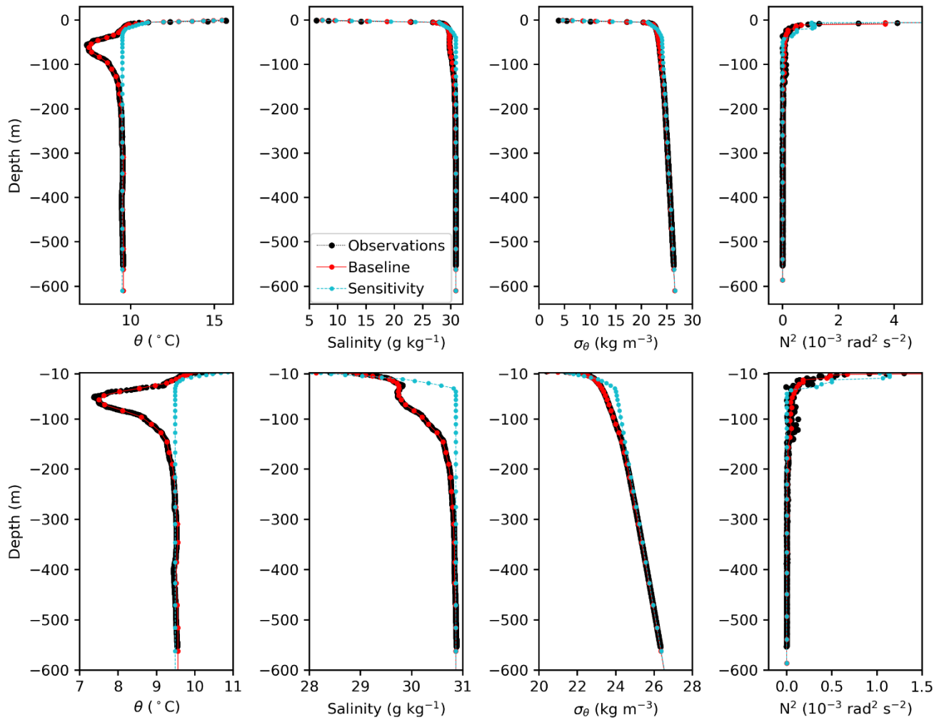
565 Figure A1. Profiles of potential temperature, salinity, density (as \sigma_\theta ), and Brunt-Väisälä frequency ( N^2 ) at station BU4 (middle of the inlet at 50.6^\circ\text{N} and 124.9^\circ\text{W} ) for the observations on 23 May 2019 (black) and the initial conditions for the baseline (red) and sensitivity (blue) simulations. Top row shows the whole water column and bottom row focuses on values below 10 m.
