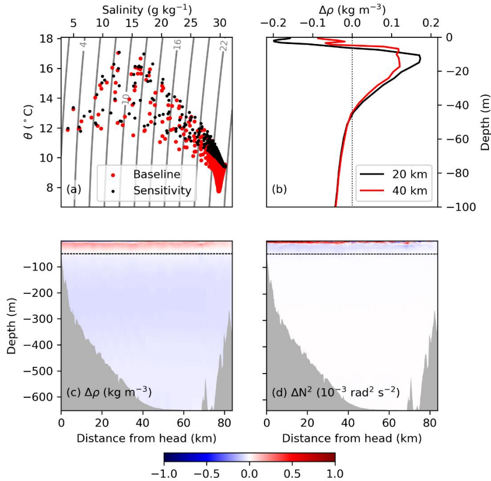
545 Figure 6. (a) Temperature-salinity diagram for the baseline (red) and sensitivity (black) simulations in Bute Inlet. Model results shown at the time and location of the observations (12 and 26 June 2019; location in Fig. 4g); for reference, four isopycnals were labelled according to their \sigma_\theta (kg m -3 ). (b) Profiles of mean density difference between of both simulations ( \Delta\rho ) at 20 and 40 km away 550 from the head of the inlet, shown in the top 100 m of the water column. Bottom panels show along-inlet transects of the difference in (c) mean density and (d) mean Brunt-Väisälä frequency ( N^2 ) between baseline and sensitivity experiments ( \Delta = 29-day average baseline minus 29-day average sensitivity; negative values indicate that the baseline is less dense/stratified than the sensitivity simulation).
