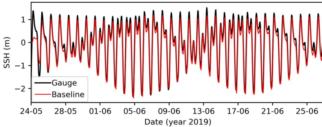
570 Figure A2. Observed (black) and modelled (red) time series of sea surface height (SSH) at Campbell River. Location of tidal gauge shown as a triangle in Fig. 1b.
