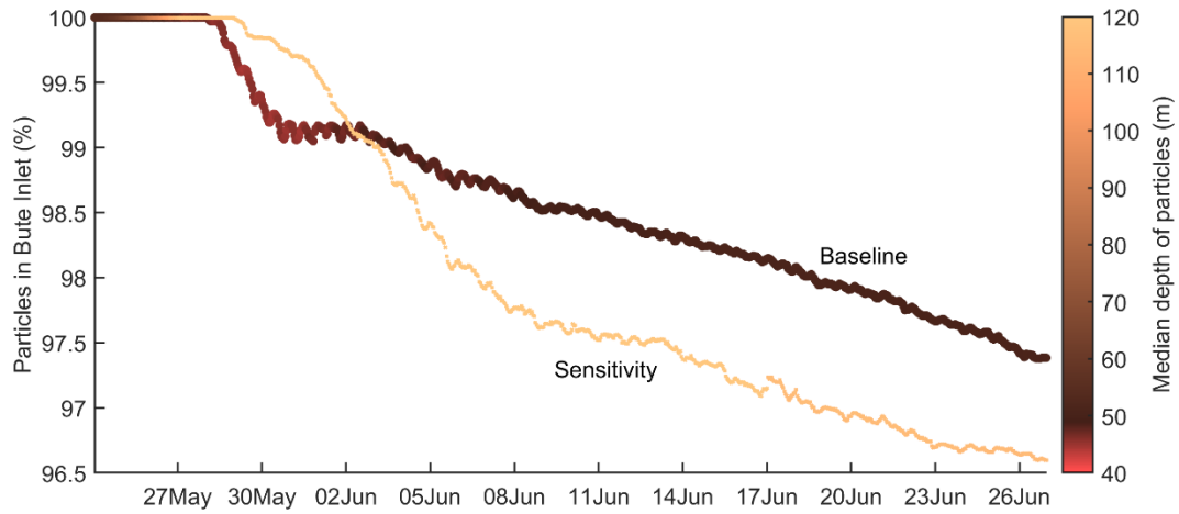
555 Figure 7. Time series of total percent of particles retained in Bute Inlet (north of 50.45 °N) in the particle tracking experiments using the velocity fields from the baseline and sensitivity simulations. Lines are coloured according to the median depth of the particles inside the inlet at any given time. Particles were removed from the analysis if and as they reached the coastline or the seafloor.
