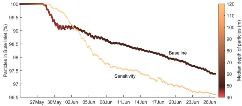
Figure 7. Time series of total percent of particles retained in Bute Inlet (north of 50.45 °N) in the particle tracking experiments using the velocity fields from the baseline and sensitivity simulations. Lines are coloured according to the median depth of the particles inside the inlet at any given time. Particles were removed from the analysis if and as they reached the coastline or the seafloor.
