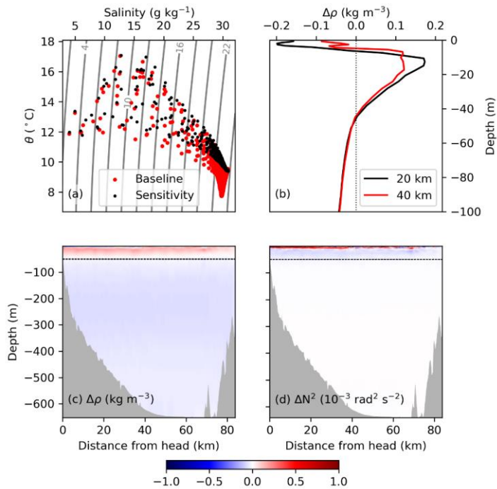
Figure 6. (a) Temperature-salinity diagram for the baseline (red) and sensitivity (black) simulations in Bute Inlet. Model results shown at the time and location of the observations (12 and 26 June 2019; location in Fig. 4g); for reference, four isopycnals were labelled according to their \sigma_\theta ( \text{kg m}^{-3} ). (b) Profiles of mean density difference between of both simulations ( \Delta\rho ) at 20 and 40 km away from the head of the inlet, shown in the top 100 m of the water column. Bottom panels show along-inlet transects of the difference in (c) mean density and (d) mean Brunt-Väisälä frequency ( N^2 ) between baseline and sensitivity experiments ( \Delta = 29 -day average baseline minus 29-day average sensitivity; negative values indicate that the baseline is less dense/stratified than the sensitivity simulation).
