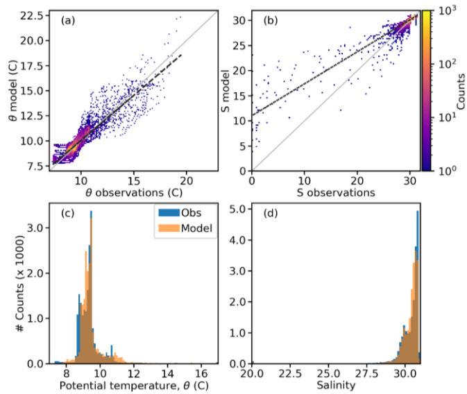
Figure 2. Two-dimensional histograms for (a) potential temperature and (b) salinity; the gray line shows the 1:1 slope and the cyan dashed black line, the linear regression fit. Overlapped model and observed histograms for (c) potential temperature and (d) salinity.
