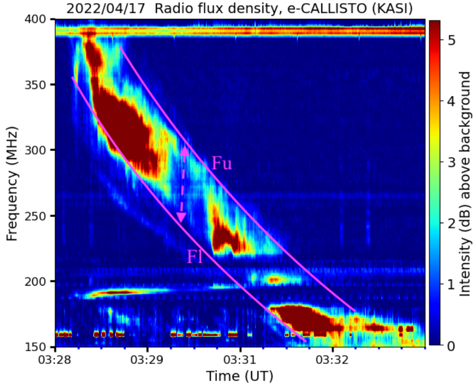
Figure 1. Type II radio burst from 03:28:25 UT to 03:32:30 UT observed by Korean Astronomy and Space science Institute (KASI) on April 17, 2022. F_u and F_1 denote the upper and lower frequencies of the fundamental band of the type II radio emission.
