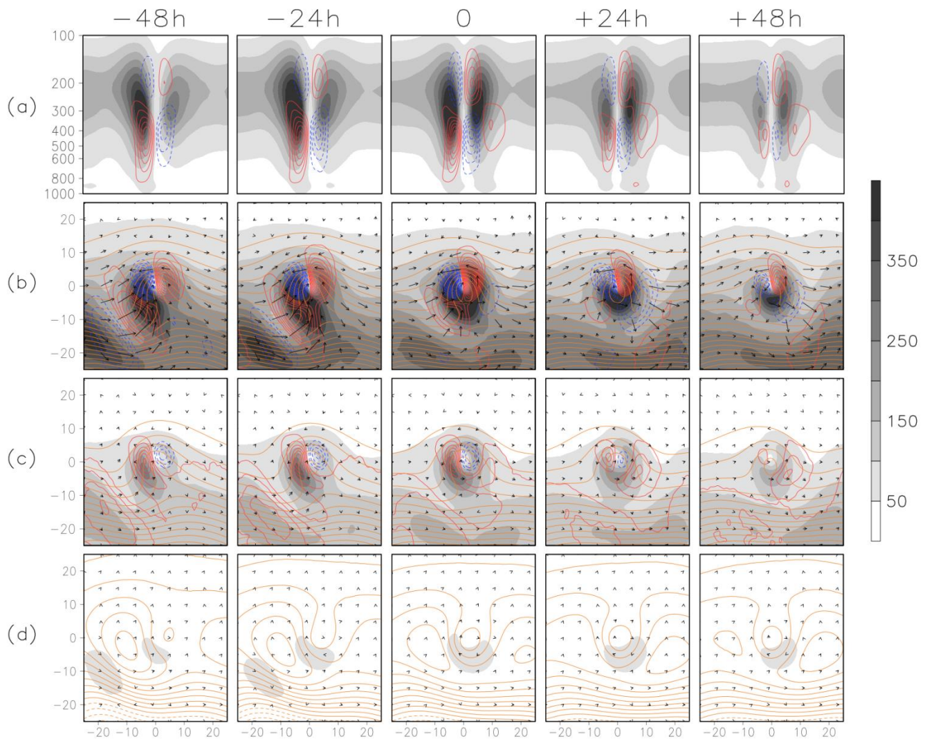
340 Figure 6: Same as Figure 5 but for deep COLs in the Southern Hemisphere. Dashed lines at the bottom indicate negative geopotential height at 1000 hPa.
