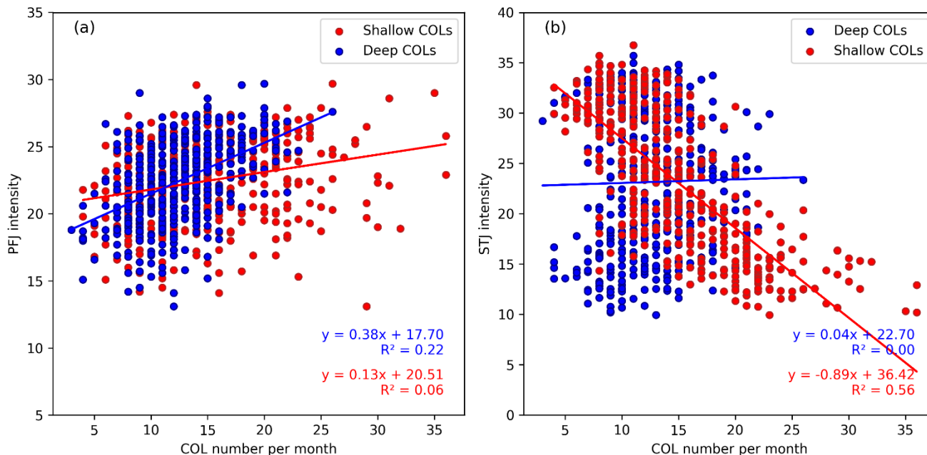
Figure 4: Scatter plots indicating the relationships between monthly mean COL number and jet intensity for (a) polar front jet and (b) subtropical jet, and COL intensity and jet intensity for (c) polar front jet and (d) subtropical jet. Deep and shallow COLs are depicted by blue and red colors, respectively. Unit is in \text{m}\cdot\text{s}^{-1} for jet intensity and 10^{-5}\cdot\text{s}^{-1} for COL intensity (scaled by -1 ).
