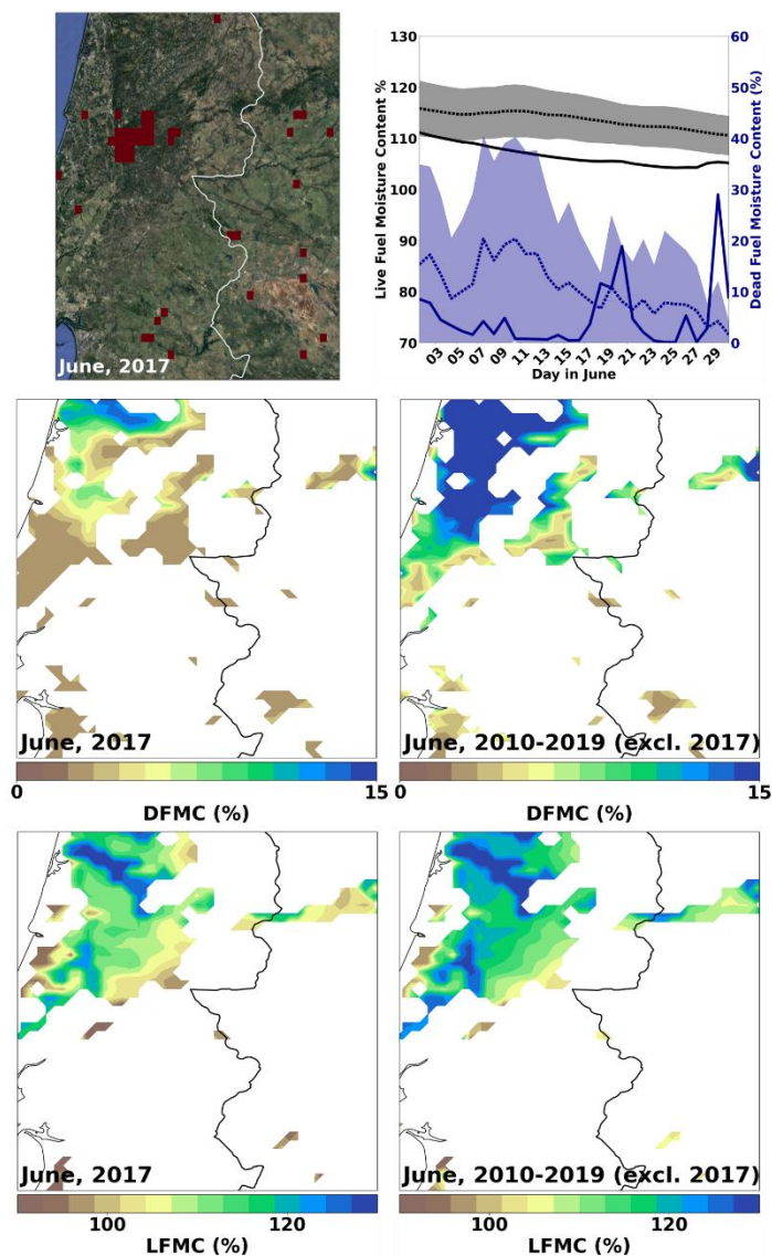
835 Figure 10. Spatial distribution of June 2017 active fire detections from MODIS over central Portugal where red indicates positive detection (top left). The June 2017 (solid line) and June 2010-2019 excluding 2017 (dashed line) regional average live fuel moisture content (black) and dead fuel moisture content (blue) for the same domain (top right). Also shown is a spatial representation at ~9km of the average June 2017 (left) and June 2010-2019 excluding 2017 (right) dead (middle row) and live (bottom row) fuel moisture content.
