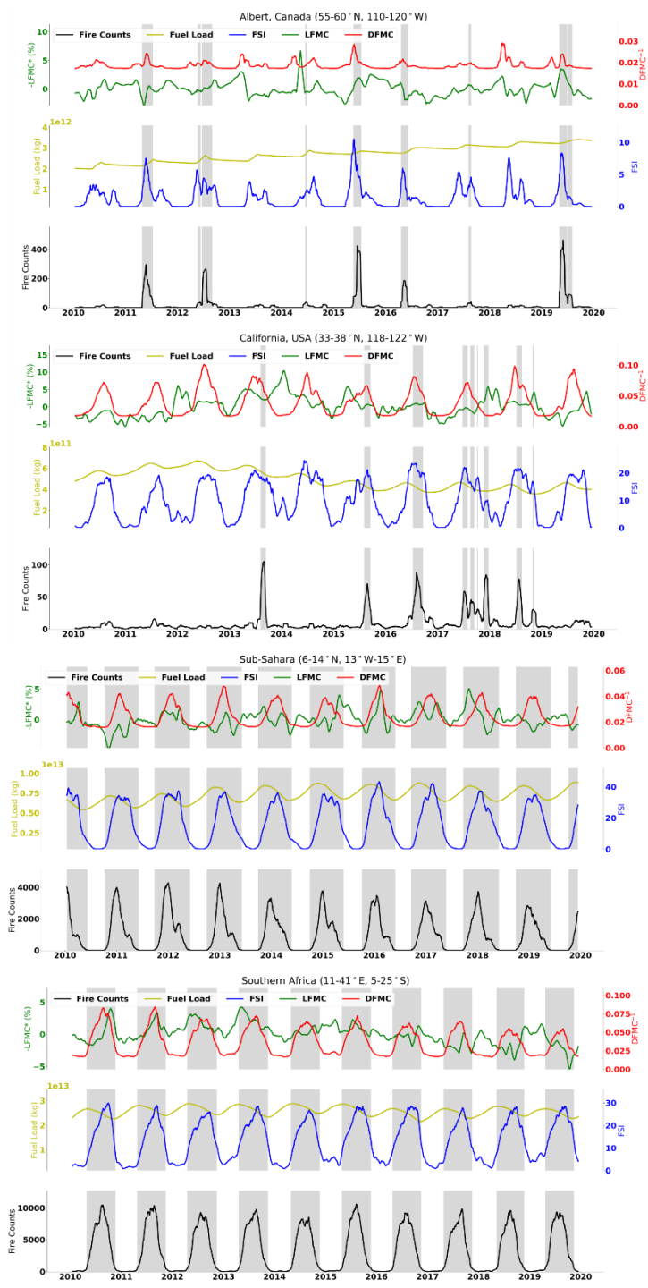
Figure 12. Timeseries between 2010 and 2019 of fire counts (black), fuel load (yellow), FSI (blue), negative LFMCA anomaly (green), DFMC -1 (red) for Alberta, Canada (top), California, USA (second panel), Northern Sub-Saharan Africa (third panel) and Southern Africa (bottom) using a 30-day average. Shaded regions denote active fire seasons.
