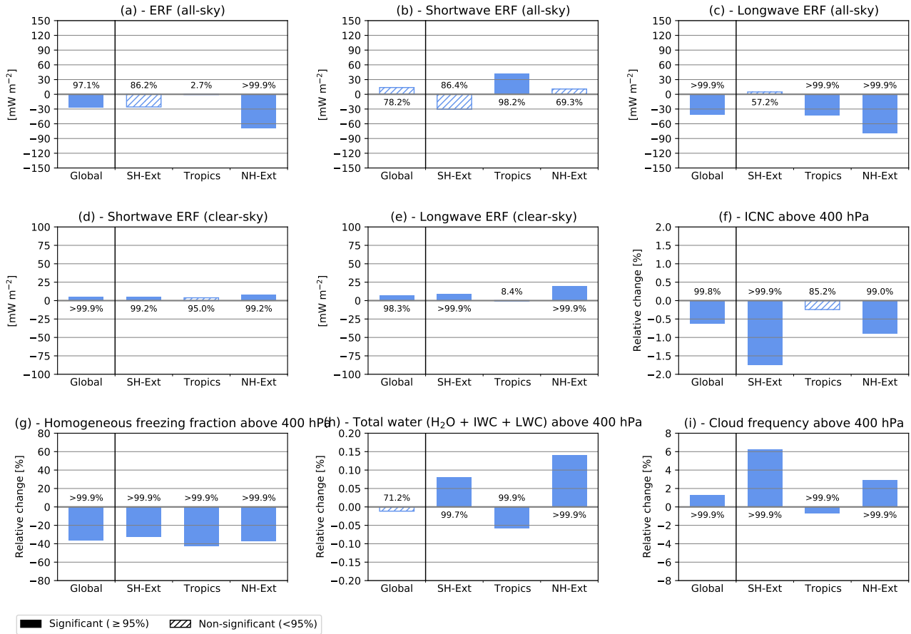
Figure 4. As in Fig. 2, but showing the INP-cirrus effect induced by mineral dust and soot INPs only, considering the central f_{act} value, calculated from the difference between a simulation including these INPs and a simulation with only homogeneous freezing. Global and latitude-specific, regional differences are shown for (a) total all-sky, (b) all-sky shortwave, (c) all-sky longwave, (d) clear-sky shortwave, (e) clear-sky longwave top-of-the-atmosphere ERFs. Panels (f-i) depict relative changes in the all-sky ICNC, fraction of homogeneously formed ice crystals, total water (as the sum of water vapour and ice water), and cloud occurrence frequency, all spatially averaged above the 400 hPa level, considering multi-year averages over the simulated period (2001–2010).
