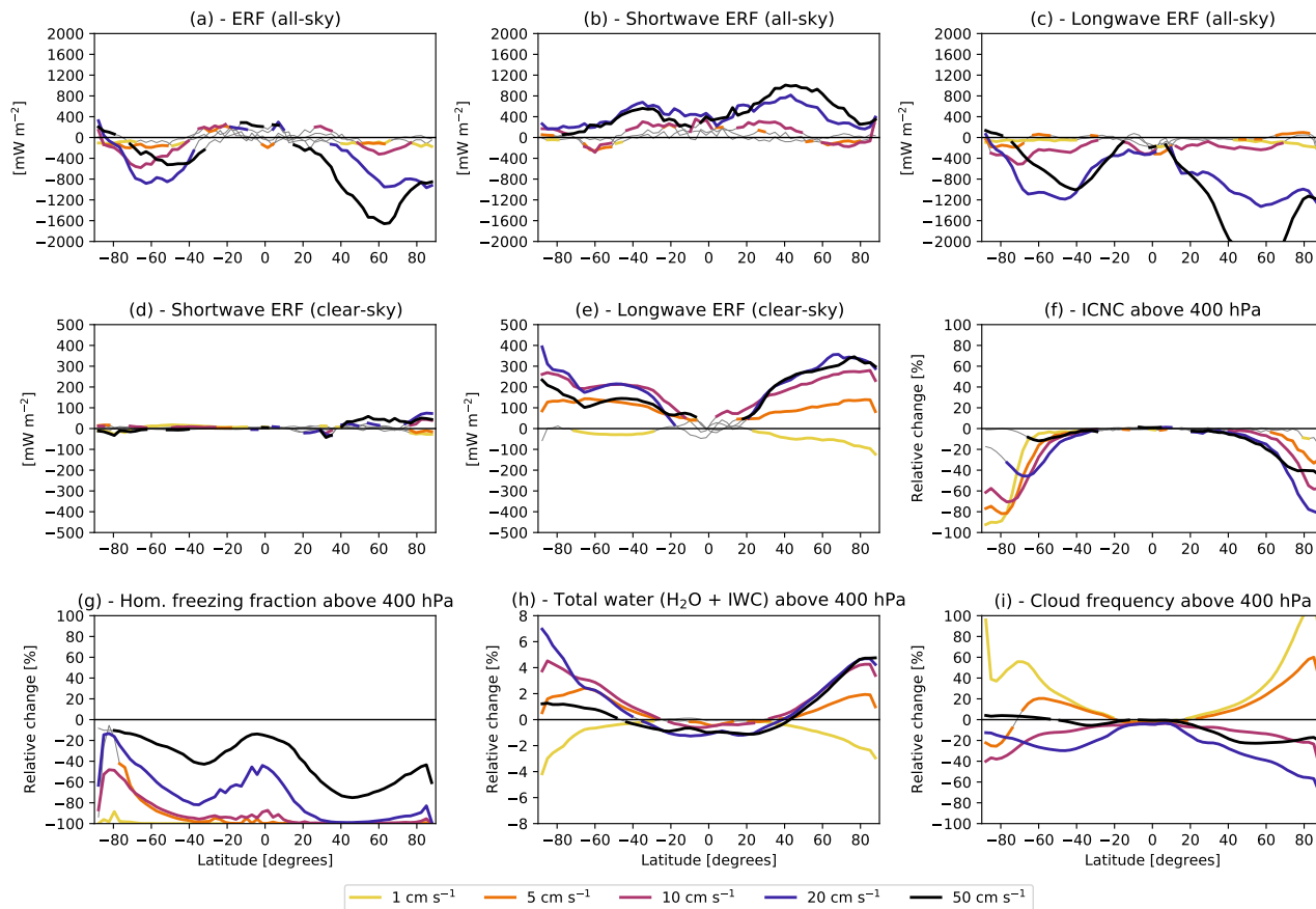
Figure 8. As in Fig. 7, but showing zonal averages of changes in (a) total all-sky, (b) all-sky shortwave, (c) all-sky longwave, (d) clear-sky shortwave, (e) clear-sky longwave top-of-the-atmosphere ERFs, and relative changes averaged above the 400 hPa level for (f) all-sky ICNC, (g) the fraction of homogeneously formed ice crystals, (h) total water (as the sum of water vapour and ice water), and (i) cloud occurrence frequency, considering multi-year averages over the simulated period (2001–2010). Non-significant values are shaded in grey.
