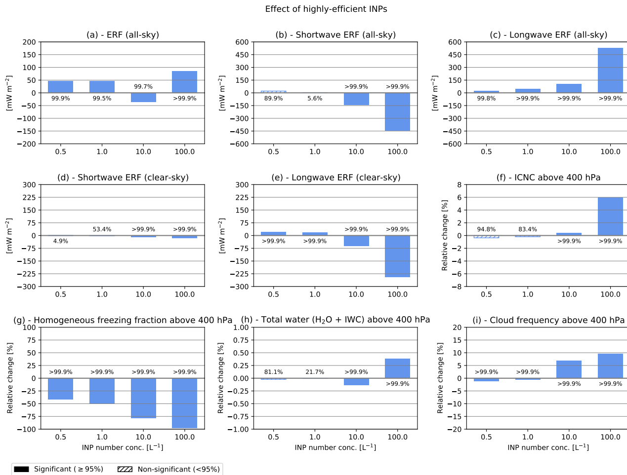
Figure 9. As in Fig. 7, but showing multi-year averages (years 2001–2010) of the effect of highly efficient INPs (assuming S_c = 1.05 , f_{act} = 1.0 ) for different prescribed concentrations, considering changes in (a) total all-sky, (b) all-sky shortwave, (c) all-sky longwave, (d) clear-sky shortwave, (e) clear-sky longwave top-of-the-atmosphere ERF, and relative changes averaged above the 400 hPa level for (f) all-sky ICNC, (g) the fraction of homogeneously formed ice crystals, (h) total water (as the sum of water vapour and ice water), and (i) cloud occurrence frequency.
