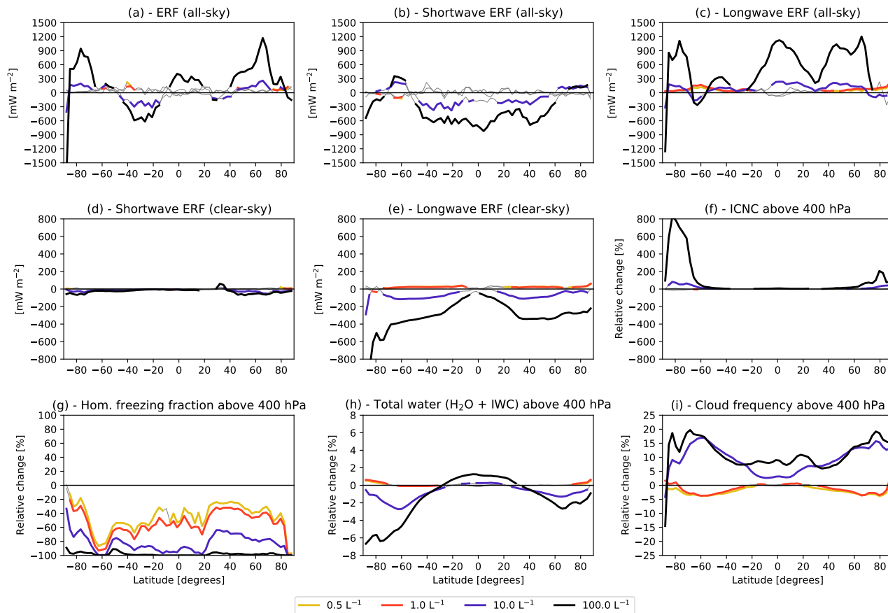
Figure 10. As in Fig. 7, but showing zonal averages of changes in (a) total all-sky, (b) all-sky shortwave, (c) all-sky longwave, (d) clear-sky shortwave, (e) clear-sky longwave top-of-the-atmosphere ERFs, and relative changes averaged above the 400 hPa level for (f) all-sky ICNC, (g) the fraction of homogeneously formed ice crystals, (h) total water (as the sum of water vapour and ice water), and (i) cloud occurrence frequency, considering multi-year averages over the simulated period (2001–2010). Non-significant values are shaded in grey.
