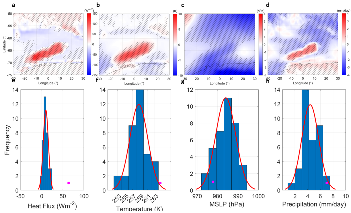
Figure 8: ERA5 heat flux (a) difference between 1974 and the 1980-2015 average for September-October mean. (b) as (a) for surface temperature. (c) as (a) but for MSLP. (d) as (a) but for precipitation. Stippling indicates the 95% significance level by t-test and the Benjamini-Hochberg procedure. (e) Histogram of 1980:2015 September-October mean heat flux over the WSP region (red box in Fig. 1) for the years 1980 through 2015. A best fit normal distribution is shown in solid red line while a pink star denotes the 1974 value (f) as (e) but for surface temperature. (g) as (e) but for MSLP. (h) as (e) but for precipitation.
