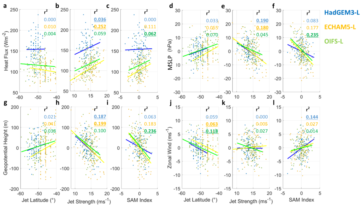
605 Figure 7: Heat flux response to the WSP (averaged over 10° E – 10° W, 63° S – 68° S; red box in Fig. 1) against jet latitude (a) jet strength (b), and SAM index (c) for the low-resolution versions of the models. Blue for HadGEM3-L, yellow for ECHAM5-L and green for OIFS-L. Each dot represents each ensemble member for September. (d-f) as (a-c) but for MSLP, (g-l) as (a-c) but for geopotential height at 850 hPa, and (j-l) as (a-c) but for zonal wind at 850 hPa. Bold underline shows the dominant processes for each model.
