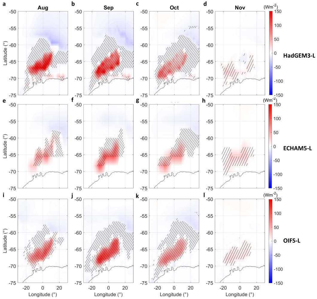
550 Figure 2: (a-d) The low-resolution turbulent heat flux (positive into the atmosphere) response to the WSP (Polynya simulation minus non-polynya simulation) for HadGEM3-L from August (a) to November (d). (e-h) as (a-d) but for ECHAM5-L. (i-l) as (a-d), but for OIFS-L. Turbulent heat flux is calculated as the combined sensible and latent heat flux. Stippling indicates the 95% significance level by t-test and the Benjamini-Hochberg procedure.
