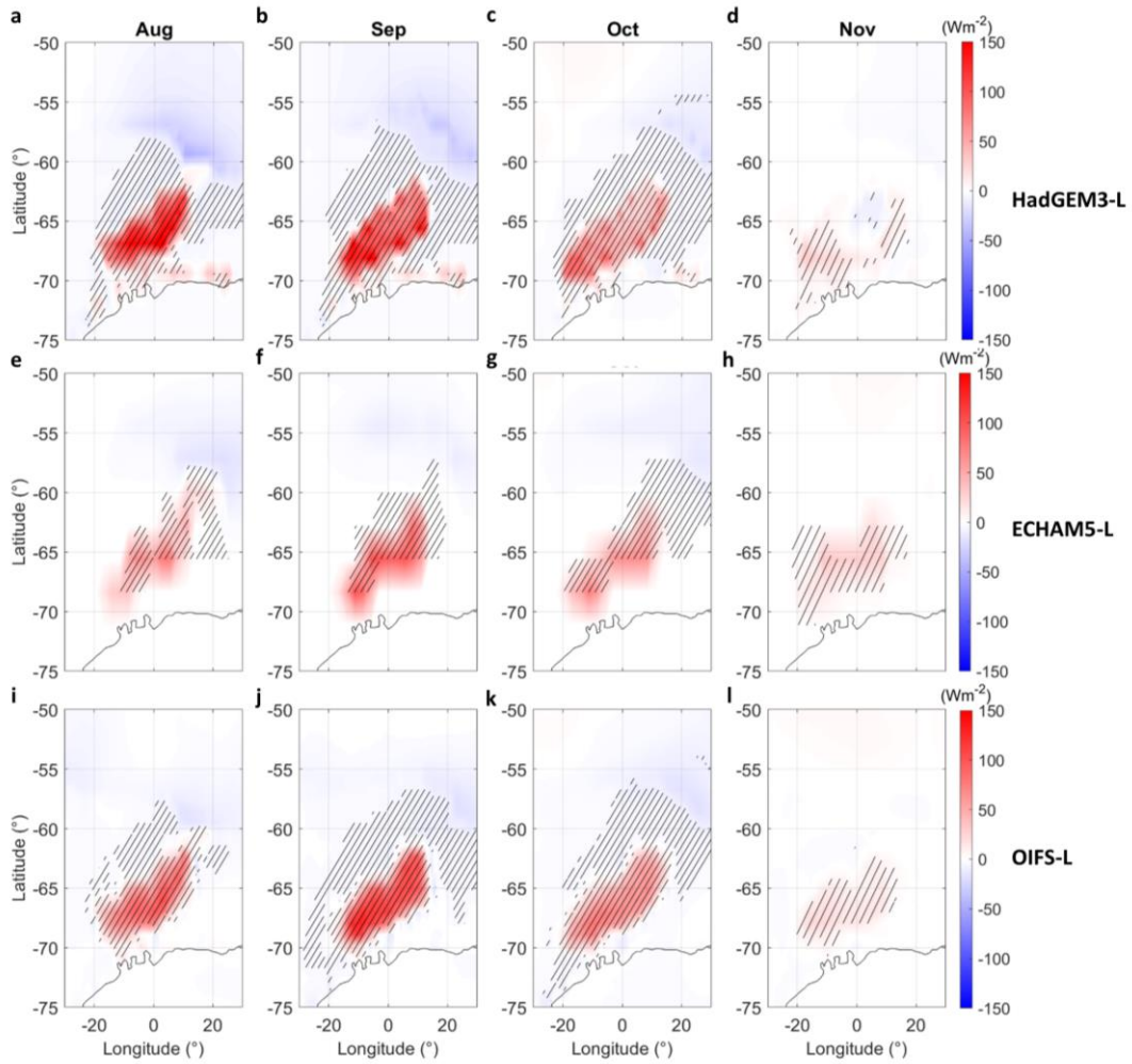
535 Figure 2: (a-d) The low-resolution turbulent heat flux (positive into the atmosphere) response to the WSP (Polynya simulation minus non-polynya simulation) for HadGEM3-L from August (a) to November (d). (e-h) as (a-d) but for ECHAM5-L. (i-l) as (a-d), but for OIFS-L. Turbulent heat flux is calculated as the combined sensible and latent heat flux. Stippling indicates the 95% significance level by t-test and False Discovery Rate.
