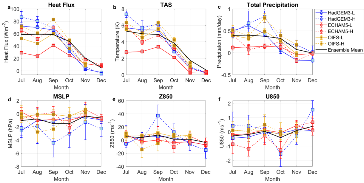
Figure 6: (a) Monthly mean and standard error of heat flux response to the WSP averaged over ( 10^{\circ} \text{ E} - 10^{\circ} \text{ W}, 63^{\circ} \text{ S} - 68^{\circ} \text{ S} ) (red box in Figure 1), with HadGEM3 (blue), ECHAM5 (red) and OIFS (yellow). Low-resolution and high-resolution are denoted by solid and dashed lines, respectively. The ensemble mean of all three models and both resolutions is denoted by the black solid line. (b) as (a) for surface temperature. (c) as but (a) for precipitation. (d) as (a) but for MSLP. (e) as (a) for geopotential at 850 hPa. (f) as (a) but for zonal wind at 850 hPa.
