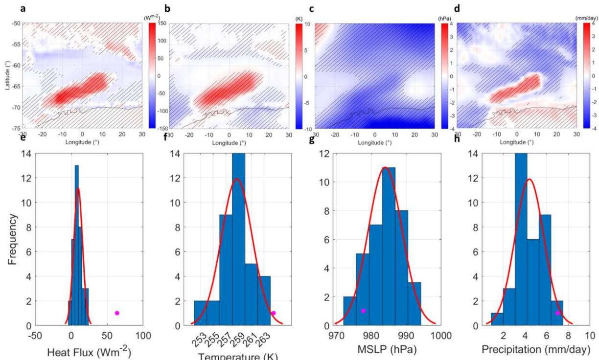
595 Figure 8: ERA5 heat flux (a) difference between 1974 and the 1980-2015 average for September-October mean. (b) as (a) for surface temperature. (c) as (a) but for MSLP. (d) as (a) but for precipitation. Stippling indicates the 95% significance level by t-test and False Discovery Rate. (e) Histogram of 1980:2015 September-October mean heat flux over the WSP region (red box in Fig. 1) for the years 1980 through 2015. A best fit normal distribution is shown in solid red line while a pink star denotes the 1974 value (f) as (e) but for surface temperature. (g) as (e) but for MSLP. (h) as (e) but for precipitation.
