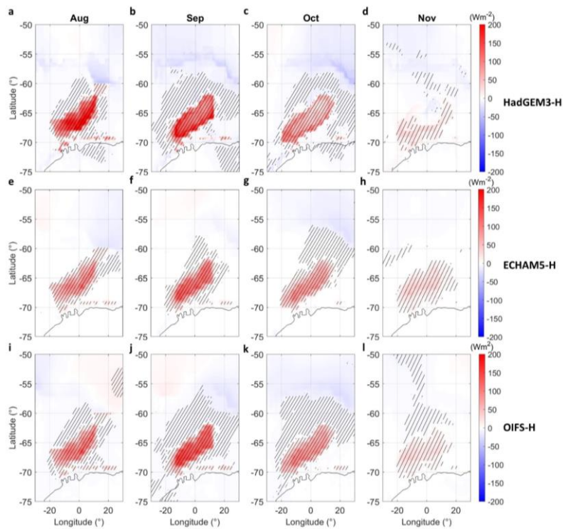
595 Figure5: The high-resolution turbulent heat flux (positive in the atmosphere) response to the WSP for HadGEM3-H from August (a) to November (d). (e-h) as (a-d) but for ECHAM5-H. (i-l) as (a-d) but for OIFS-H. Turbulent heat flux is calculated as the combined sensible and latent heat flux. Stippling indicates the 95% significance level by t-test.
