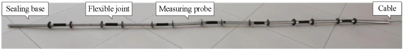
Figure 2: Schematic diagram of continuous full-hole inclinometer probe configuration.
