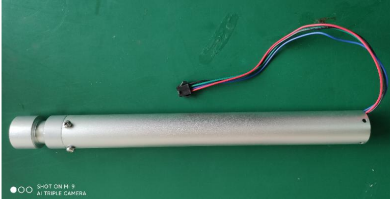
Figure 7: Assembled sensors.
