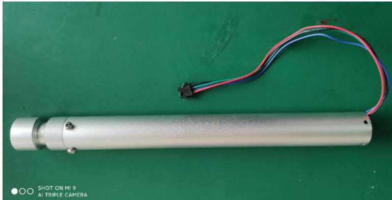
Figure 7: Assembled sensors.
