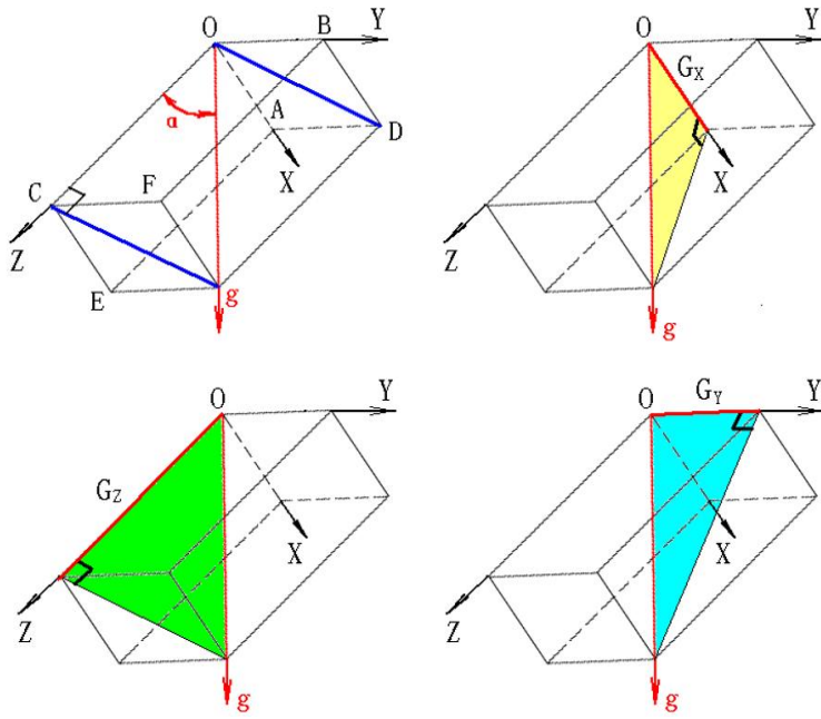
155 Figure 4: Vertex angle measurement coordinate system.
