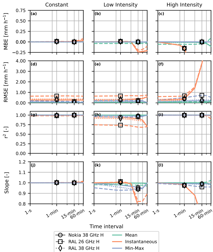
Figure 6. Statistical metrics as function of time interval for three theoretical rain events (Fig. 3) for all sampling methods (line colour) and added noise levels that resemble the three devices (line style). The markers indicate the values for the 15-minute min-max and 1-minute instantaneous sampling strategies.
