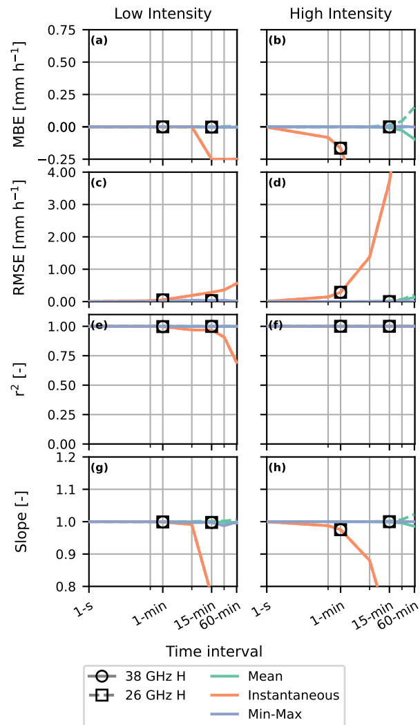
Figure 7. Statistical metrics as function of time interval for for a theoretical low intensity and high intensity rain event (Fig. 3) for all sampling methods (line colour) for 38 GHz and 26 GHz horizontally polarized noiseless devices (line style). The markers indicate the values for the 15-minute min-max and 1-minute instantaneous sampling strategies.
