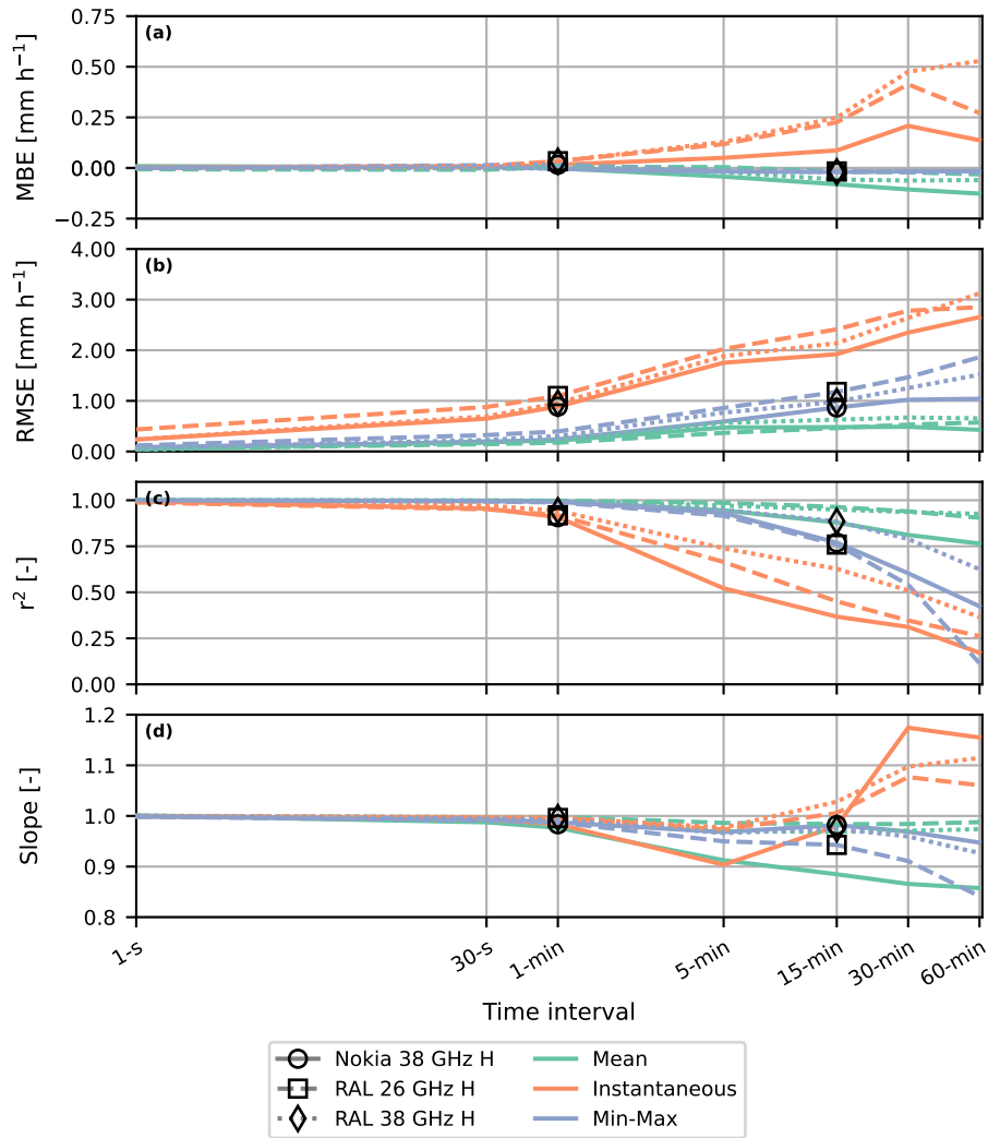
Figure 10. Statistical metrics as function of time interval for all devices (line style) and sampling methods (line colour). The markers indicate the values for the 15-minute min-max and 1-minute instantaneous sampling strategies. The values for the metrics are obtained from Figs. S1 to S4.
