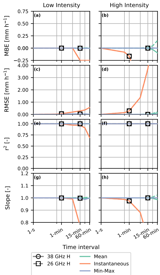
Figure 7. Statistical metrics as function of time interval for for a theoretical low intensity and high intensity rain event (Fig. 3) for all sampling methods (line stylecolour ) for 38 GHz and 26 GHz horizontally polarized noiseless devices (line colourstyle ). The markers indicate the values for the 15-minute min-max and 1-minute instantaneous sampling strategies.
