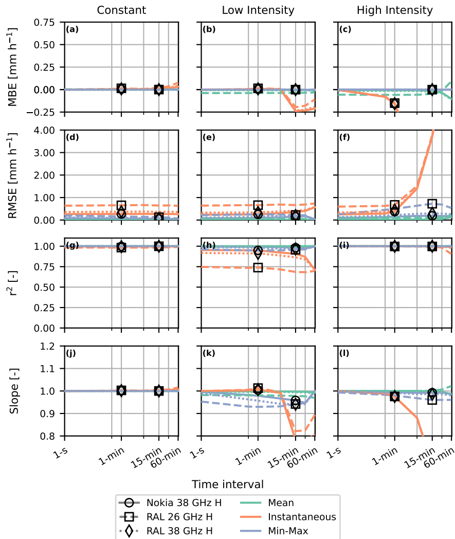
Figure 6. Statistical metrics as function of time interval for three theoretical rain events (Fig. 3) for all sampling methods (line stylecolour) and added noise levels that resemble the three devices (line colourstyle). The markers indicate the values for the 15-minute min-max and 1-minute instantaneous sampling strategies.
