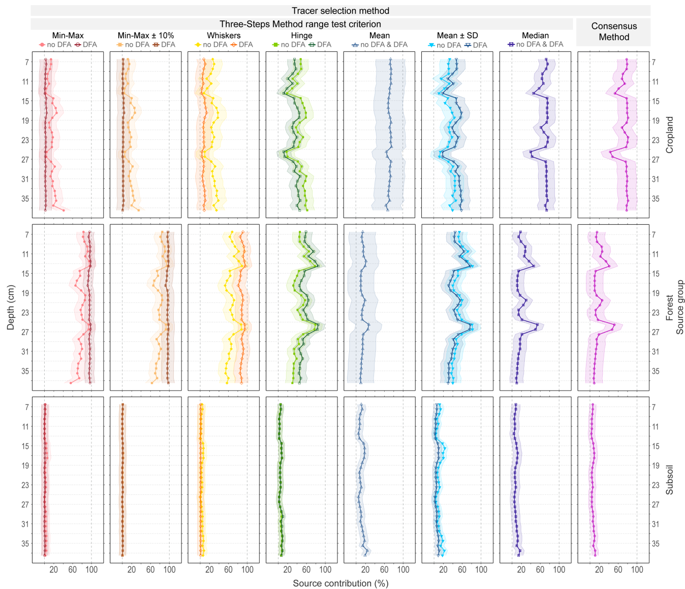
Figure 8. Predicted source contributions for the sediment core samples according to each tracer selection approach. The different range tests criteria of the three-step method (TSM): minimum-maximum (red circle), minimum-maximum \pm 10% (brown crossed circle), whiskers (yellow/orange diamond), hinge (green square), mean (blue triangle), mean \pm SD (light blue triangle point down), median (purple crossed square) and consensus method (CM; light purple circle plus). Empty and filled symbols correspond to the use of DFA or not. The error buffer ribbons around the plotted values correspond to the respective RMSE values calculated on virtual mixtures.
