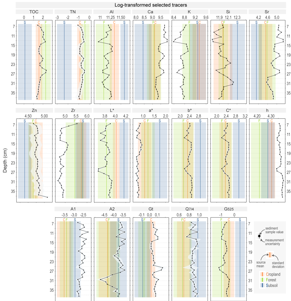
Figure 9. Log-transformed values of selected tracers along the sediment core (black dot; and measurement uncertainty represented with a grey buffer) and in the potential source signatures (vertical line represents mean value and the buffer zone along each lines represents the standard deviation).
