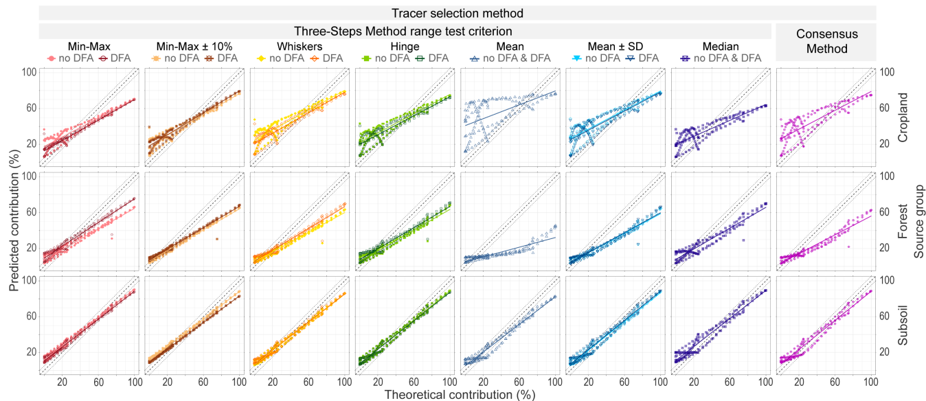
Figure 6. Relationship between theoretical and predicted virtual mixture source contributions: cropland, forest, subsoil, according to each tracer selection approach: three-step method (TSM) range test criteria: minimum-maximum (red circle), minimum-maximum \pm 10\% (brown crossed circle), whiskers (yellow/orange diamond), hinge (green square), mean \pm SD (blue triangle point down) filled and empty symbols correspond to the selection before DFA (no DFA) and after DFA respectively, except for mean (blue triangle) and median (blue crossed square) criteria for which empty symbols correspond to the same selection of tracers before and after DFA, and consensus method (CM; purple circle plus).
