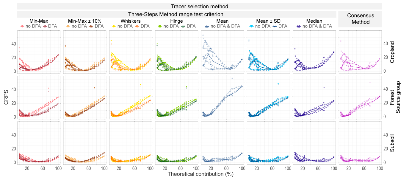
Figure 7. Relationship between theoretical virtual mixture source contributions and continuous ranked probability score (CRPS) across sources: three-step method (TSM) range test criteria: minimum-maximum (red circle), minimum-maximum \pm 10% (brown crossed circle), whiskers (yellow/orange diamond), hinge (green square), mean \pm SD (blue triangle point down) filled and empty symbols correspond to the selection before DFA (no DFA) and after DFA respectively, except for mean (blue triangle) and median (blue crossed square) criteria for which empty symbols correspond to the same selection of tracers before and after DFA, and consensus method (CM; purple circle plus).
