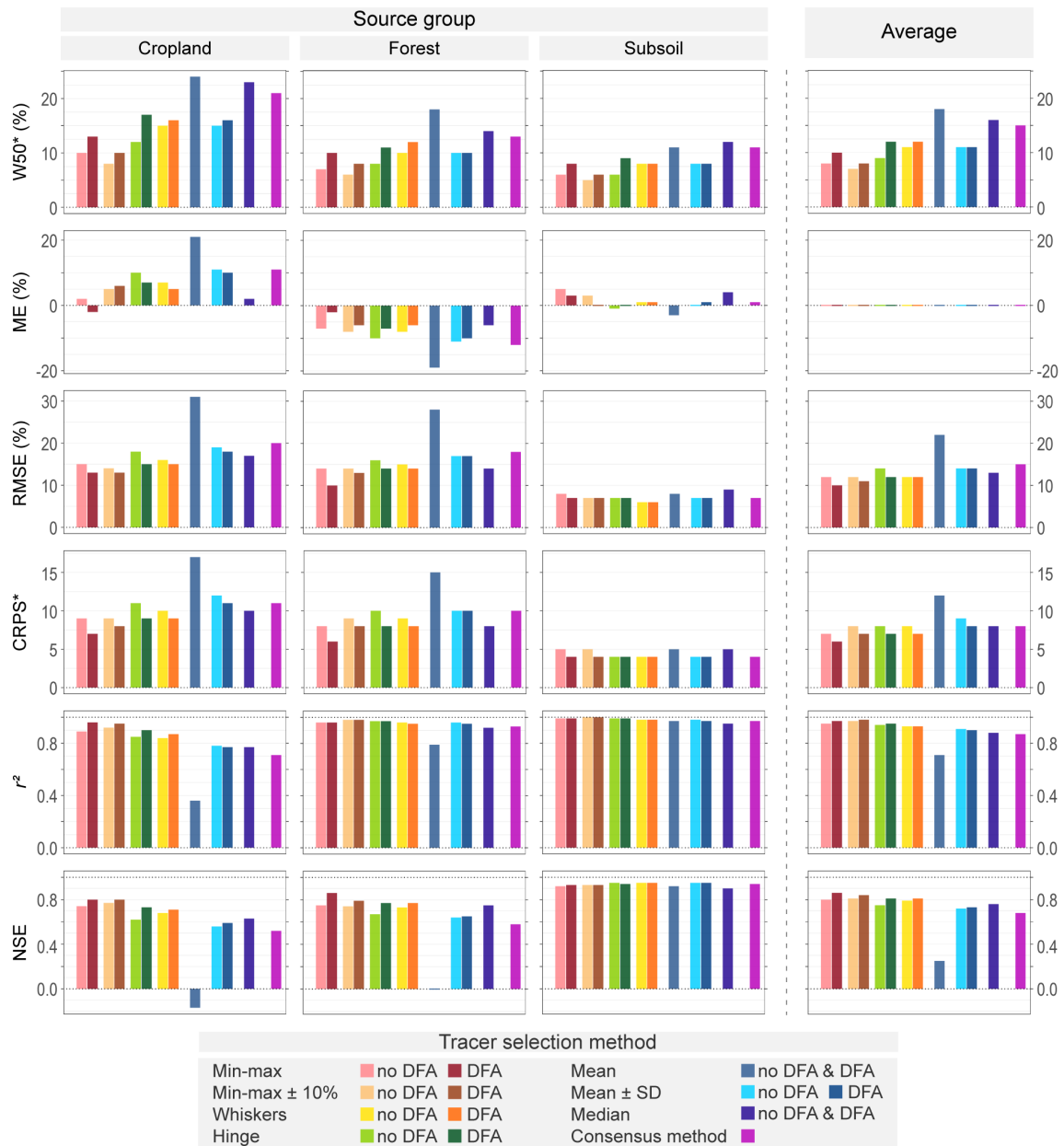
Figure 4. Summary of MixSIAR accuracy statistics calculated on virtual mixtures ( n = 138 ) for each tracer selection method: Three-step Method (TSM) range test criteria and consensus method (CM) for each individual soil source and average of all three sources for each method. Tracers selected by each method are listed in Table 3. Model accuracy statistics were shown by darker barplot for each selection approach. W50*: prediction interval width; ME: mean error; RMSE: root mean square error; r^2 : squared Pearson's correlation coefficient; NSE: Nash-Sutcliffe modelling efficiency coefficient; CRPS: continuous ranked probability score. Note: * = Mean values per source.
