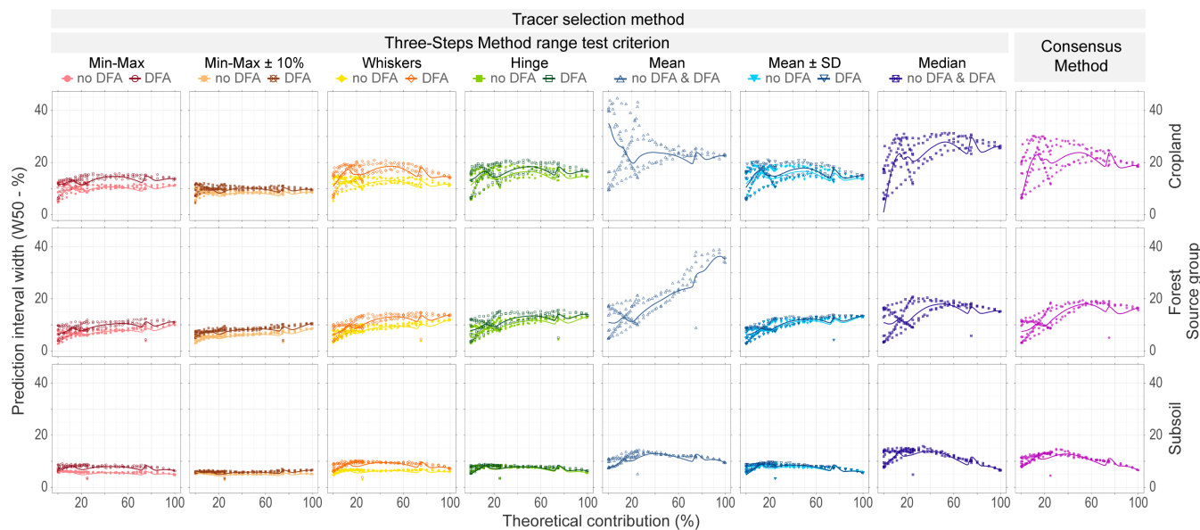
Figure 5. Relationship between theoretical virtual mixture source contributions and prediction interval width (W50) across sources: cropland, forest, subsoil, according to each tracer selection approach: three-step method (TSM) range test criteria: minimum-maximum (red circle), minimum-maximum \pm 10% (brown crossed circle), whiskers (yellow/orange diamond), hinge (green square), mean \pm SD (blue triangle point down) filled and empty symbols correspond to the selection before DFA (no DFA) and after DFA respectively, except for mean (blue triangle) and median (blue crossed square) criteria for which empty symbols correspond to the same selection of tracers before and after DFA, and consensus method (CM; purple circle plus).
