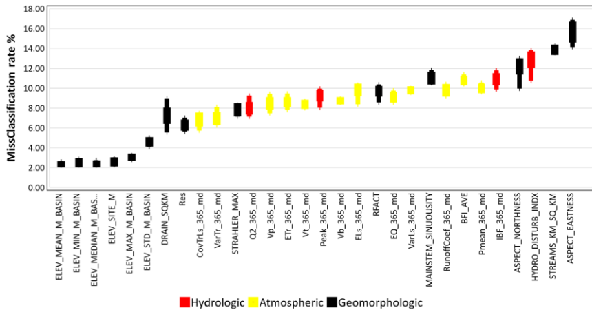
Figure 6: Selected variables based on missclassification rate (%).
