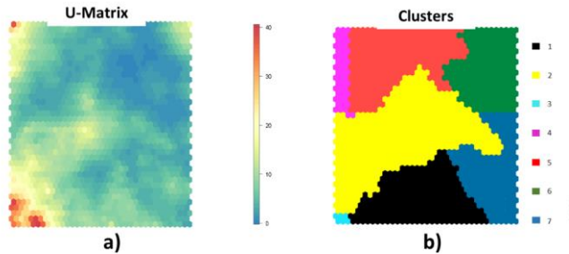
310 Figure 5: Example of (a) U-Matrix and (b) derived clusters. Red colors in the U-Matrix stand for significant distances in the feature space, whereas blue colors are "valleys" that group subsets of related data. The watersheds shown in (b) are collections of related data.
