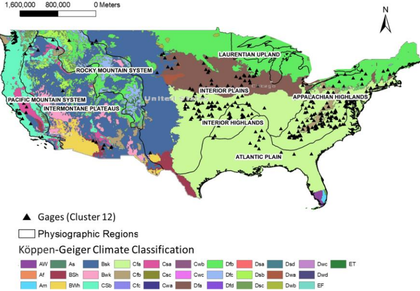
Figure A1: Gages with clustering identification assigned by SOM unsupervised clustering (a-l). For the acronym description of Physiographic regions and climate types please refer to Table A1 and A2.
