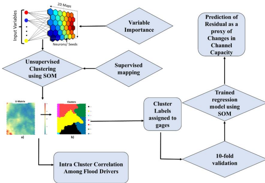
265 Figure 4: Schematic of the SOM framework proposed in this study.
