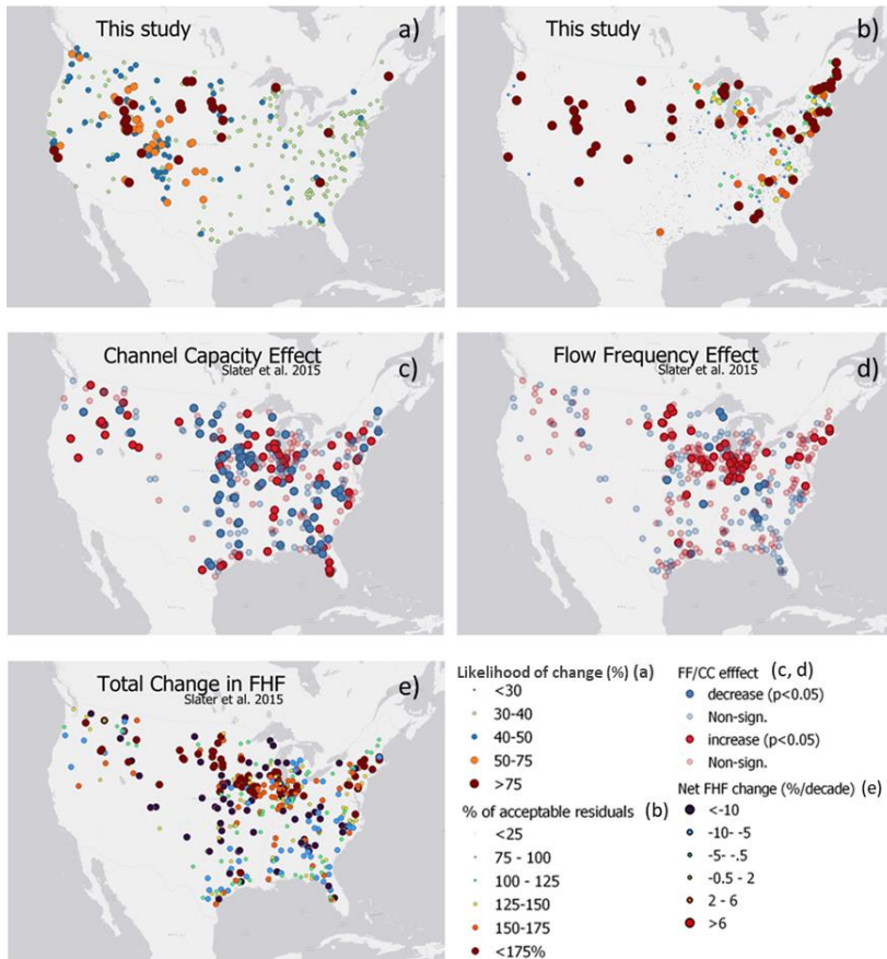
630 Figure 10: Predicted changes as compared to the results of Slater et al. (2015) showing Channel Capacity (CC) and Flow Frequency (FF) effects on flood hazard frequency (FHF). In (a) “Likelihood of change”- the percentage represents the number of times the model predicts a residual change from positive to negative after a major flood (for N = 365 ); in (b) the panel shows the ratio between average prediction and lower 95% confidence bound of the current stage-discharge relationship for the stations showing a drastic change positive to negative. In (a, b) gages with small variations from this study have been reduced for clarity. Panel (c,d, and e) are results from Slater et al. 2015.
