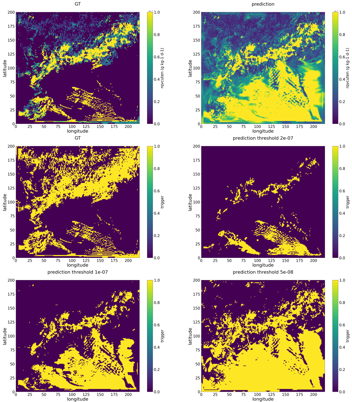
Figure A4. Snapshot examples of rqvcuten summed along the vertical direction, with the top left panel showing the GT values and the top right panel showing the rqvcuten predicted by the Bi-LSTM-tendency model, for the 25-hour WRF simulation initialized at 12UTC on May 20th, 2021. Similarly, snapshot examples of trigger, with the GT shown in the middle left panel, and the predictions from the Bi-LSTM-tendency model using varying threshold values of rqvcuten shown in the middle right column, bottom left panel, and bottom right panel, respectively.
