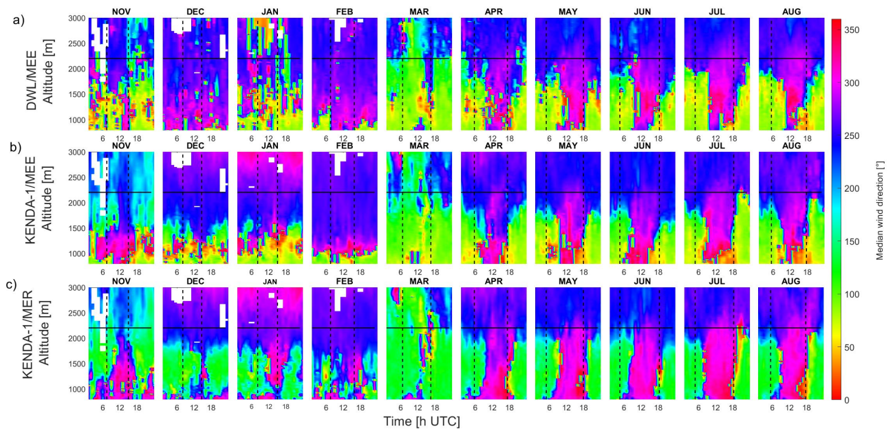
Figure 6. Monthly median wind direction [°] for a) DWL/MEE, b) KENDA-1/MEE and c) KENDA-1/MER (01.11.2021-23.08.2022). The vertical dashed lines correspond to sunrise and sunset and the horizontal line to the mean ridge height.
