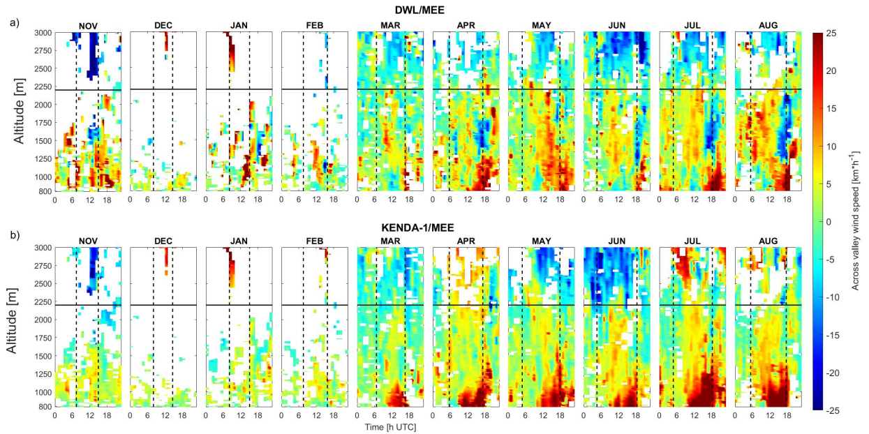
Figure 9. Evolution of the diurnal cycle of the cross-valley wind component [km/h] as a function of altitude for a) the DWL/MEE measurement and b) the KENDA-1/MEE. Winds coming from the south-facing slopes take a positive value (red), for the north-facing slope wind speeds values are negative (blue). Sunrise and sunset at ground level are given by dotted lines.
