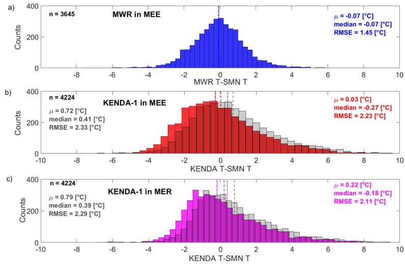
Figure 3. Distribution of the hourly T differences at the lowest level for a) MWR/MEE-SMN/MER b) KENDA-1/MEE-SMN/MER, c) KENDA/MER-SMN/MER. The lowest level corresponds to 576 m for SMN/MER, 625 m for MWR/MEE and 705 m for KENDA-1/MER and 739 m for KENDA-1/MER. The gray distributions indicate ground T differences after ELR corrections are applied. The dotted and dashed lines correspond to the median and the mean, respectively.
