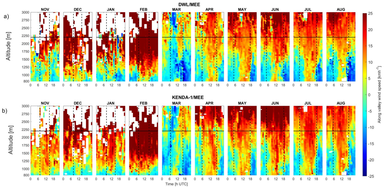
Figure 8. Monthly diurnal cycle of the along-valley wind component [km/h] as a function of altitude for a) the DWL/MEE observation and b) the KENDA-1/MEE data. Sunrise and sunset at ground level are given by dotted lines.
