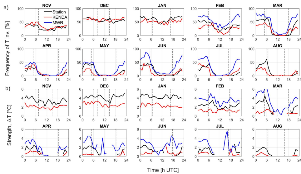
Figure 5. a) Diurnal cycle of the hourly T inversion frequency between T at SMN/MER (576 m) and FEDRO/BRU (998 m) ground stations (black), at the lowest level (625 and 739 m, respectively) and 1000 m of MWR/MEE (blue) and KENDA-1/MEE (red) profiles. b) Mean \Delta T for the time where an inversion is detected. Sunrise and sunset are represented by dotted lines.
