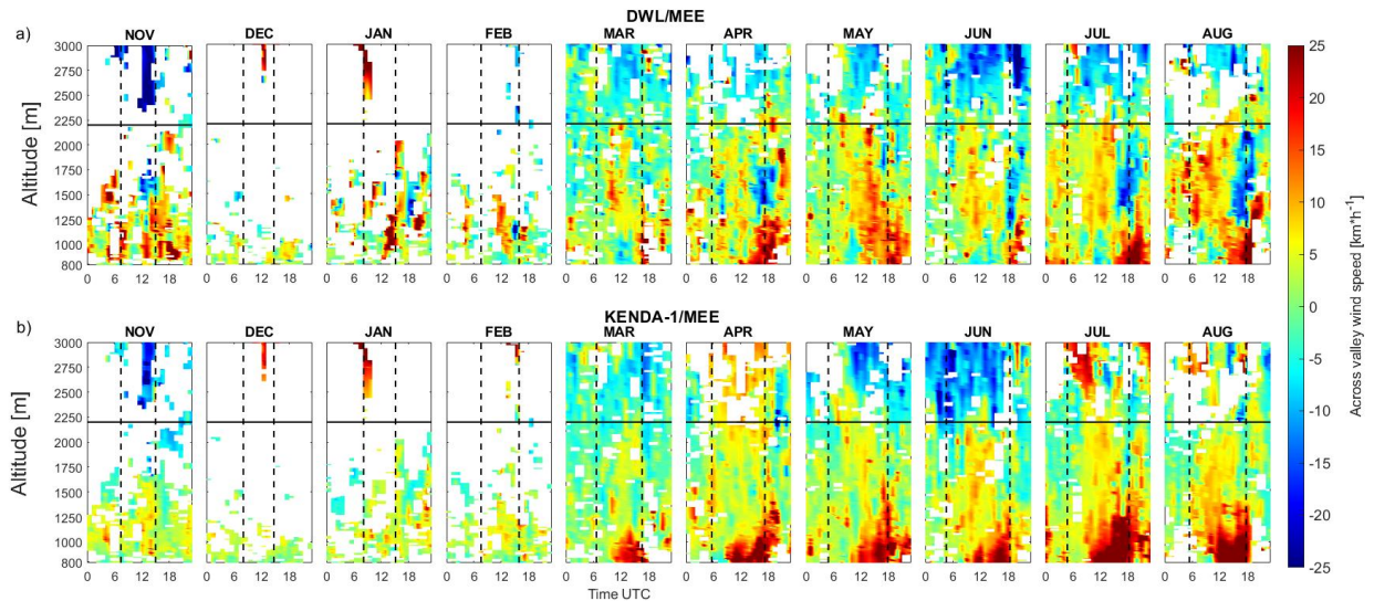
Figure 9. Evolution of the diurnal cycle of the cross-valley wind component [km/h] as a function of altitude for a) the DWL/MEE measurement and b) the KENDA-1/MEE. Winds coming from the south-facing slopes take a positive value (red), for the north-facing slope wind speeds values are negative (blue). Sunrise and sunset at ground level are given by dotted lines.
