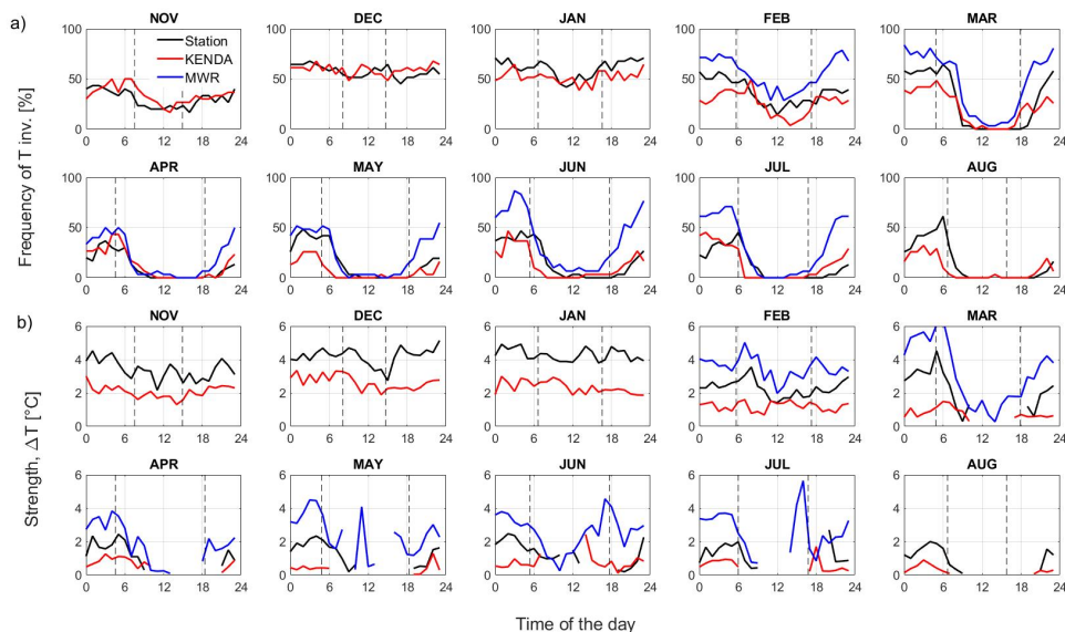
Figure 5. a) Diurnal cycle of the hourly T inversion frequency between T at SMN/MER (576 m) and FEDRO/BRU (998 m) ground stations (black), at the lowest level (625 and 739 m, respectively) and 1000 m of MWR/MEE (blue) and KENDA-1/MEE (red) profiles. b) Mean \Delta T for the time where an inversion is detected. Sunrise and sunset are represented by dotted lines.
