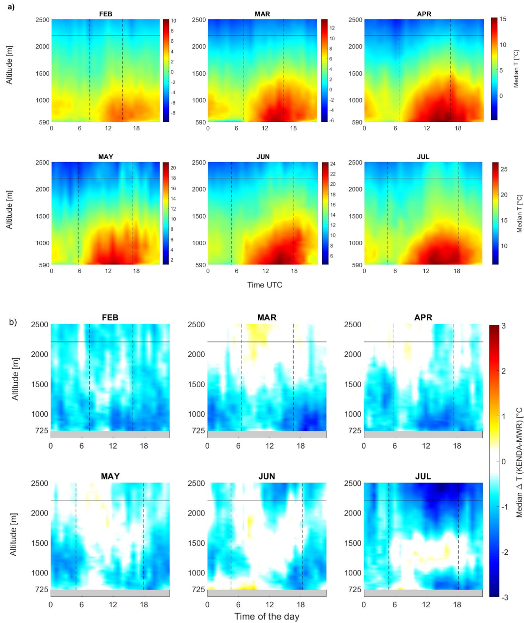
Figure 2. a) Monthly diurnal cycle of MWR/MEE T from February to July 2022. Monthly scales with a range of 20 °C but with minimum T based on the MWR/MEE profiles are used. b) Diurnal cycle of the median T profiles difference [°C] between KENDA-1/MEE and MWR/MEE for each month. The dashed vertical lines correspond to sunrise and sunset and the horizontal line to mean ridges' height.
