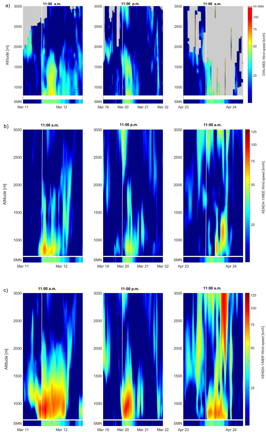
Figure 13. Wind speed profiles [km/h] time series from a) DWL/MEE, b) KENDA-1/MEE and c) KENDA-1/MER during a selection of 3 foehn events: left 11-12.03.2022, middle 19-22.03.2022 and right 23-24.04.2022. Wind speeds [km/h] from the SMN/MER are given in the lower part of each figure. The solid line represents the foehn breakthrough.
