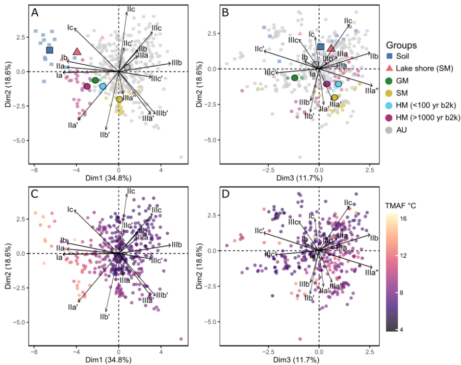
Figure 3: Principal component analysis biplots. Panels A and C show principal components 1 and 2. Panels B and D show principal components 2 and 3. Filled symbols in A and B represent the centroids of the groups (site or sample type). Fill in panels C and D is Raberg21_adj temperatures.
