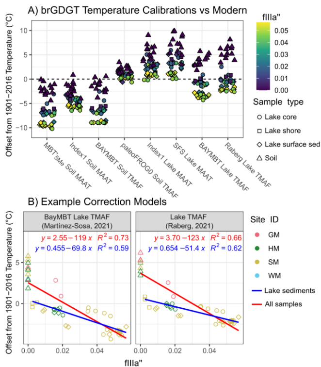
280 Figure 5: A) Offsets between brGDGT-inferred temperatures and 1901–2016 temperature data for eight different calibration models. Symbol shape corresponds to sample type, symbol fill corresponds to the fractional abundance of the IIIa'' isomer. B) Crossplots of temperature offsets and filla'' for the two most recent lacustrine brGDGT temperature calibrations (Martínez-Sosa et al., 2021; Raberg et al., 2021). The regression model fit to lake samples (blue line) was used to correct the temperature reconstructions.
