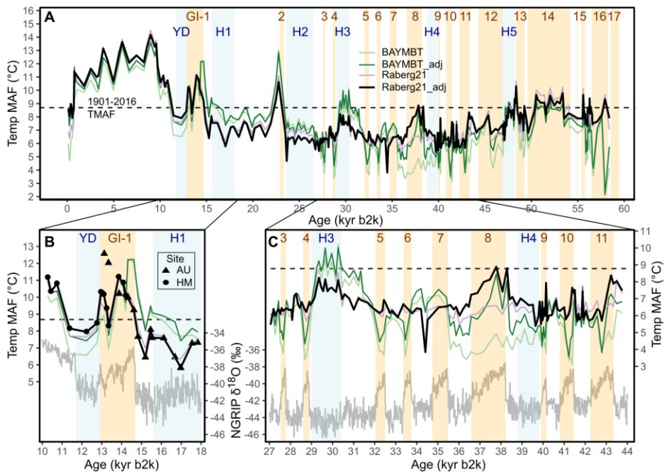
Figure 6: Comparison of brGDGT temperature reconstructions with and without correction for anoxic production of brGDGTs. Close-up panels show comparison with Dansgaard-Oeschger events in NGRIP ice core (gray, Rasmussen et al., 2014). Colored bars indicate Younger Dryas (YD), Greenland interstadials (GI) and Heinrich events (H).
