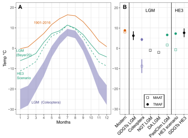
Figure 11: A) Comparison of modern seasonal temperature range for the modern period, LGM based on climate models (Beyer et al., 2020), LGM based on Coleoptera remains (Britzius and Sirocko, 2022), and a hypothetical Heinrich event scenario in which winter temperatures decrease while peak summer temperatures remain the same. B) Comparison of TMAF and MAAT for modern, LGM and HE3 based on different methods. NGT LGM = Noble Gas Temperatures from (Bekaert et al., 2023), DA LGM = data assimilation results from (Tierney et al., 2020). Notes: Coleoptera temperature range was obtained by scaling modern monthly temperatures to match the Coleoptera estimates of warmest and coldest months, the ranges represent likely values based on a simple assumption about the monthly temperature pattern, but are not a calibrated estimate.
