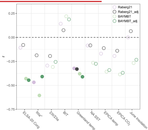
Figure 8: Assessing which factors contribute to offsets between GDGT temperature reconstructions and the Greenland \delta^{15}\text{N} temperature record after scaling mean and variance to match the GDGT temperatures (Kobashi et al., 2017; Kindler et al., 2014). Plotted is the Pearson's r for these offsets and the proxy timeseries on the x-axis. Timeseries were placed in 250-year bins before the correlation was calculated. Filled circles indicate significant correlations ( p < 0.05 after adjusting for autocorrelation and multiple hypothesis testing).
