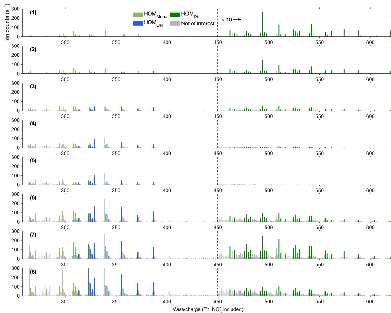
Figure A6. Steady-state spectra (15 min average) at experiment no. 2 from the \text{NO}_3 -CIMS. All spectra were corrected by subtracting the corresponding background signals. The number at each row show the order of the stage, consistent with the time series in Fig. 4. Light green bars show \text{HOM}_{\text{Mono}} , dark green ones show \text{HOM}_{\text{Di}} , blue ones show \text{HOM}_{\text{ON}} while grey ones show peaks not of interest. The peaks larger than 450 Th are multiplied by 10.
