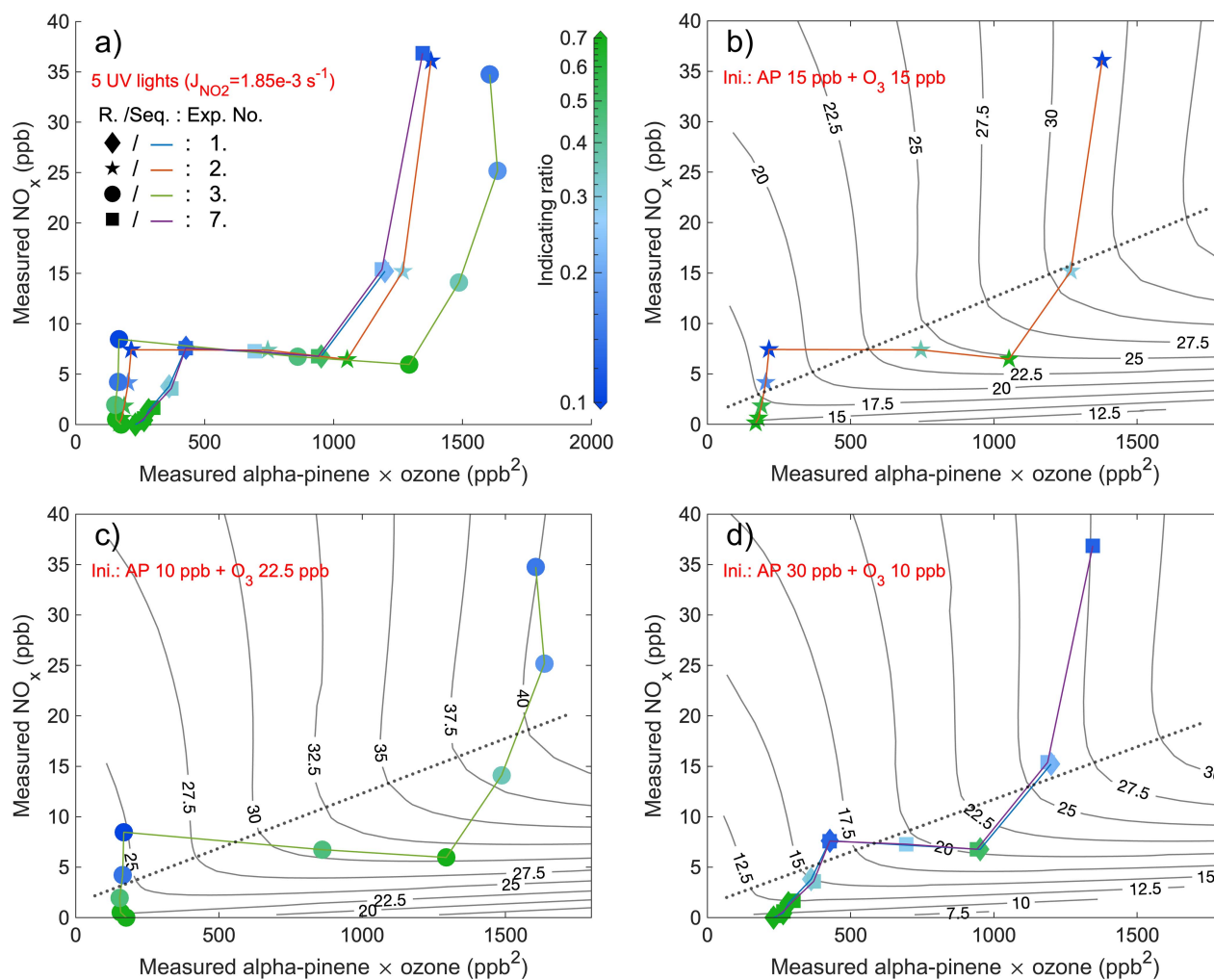
Figure 5. Steady state IR1 ( \frac{\sum \text{HOM}_{\text{Di}}}{\sum \text{HOM}_{\text{ON}, \text{O}>8}} ) of experiments from four days with 5 UV lights. X-axis is the multiplication of measured (steady state) \alpha -pinene and \text{O}_3 concentrations, while y-axis is the measured (steady state) \text{NO}_x . The scatter points (exp. no. 1 (experiment number 1): diamond; exp. no. 2: star; exp. no. 3: round; exp. no. 7: square) are colored by values of IR1 (abbreviated as R. in the figure), and are connected by curves (exp. no. 1: blue; exp. no. 2: orange; exp. no. 3: green; exp. no. 7: purple) showing the sequence (Seq.) of experimental stages. Panel a combines stages of all four days, and the rest three subplots respectively show the stages of experiments with different initial (Ini.) inputs (exp. no. 1 and 7 are in the same panel d due to same initial inputs). EKMA curves (isopleth of \text{O}_3 concentrations in ppb), simulated by the box model, are black solid lines, while dotted lines are corresponding ridge lines.
