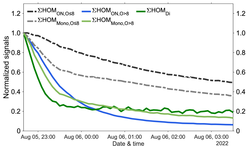
Figure 3. The normalized signal decay of \text{HOM}_{\text{ON}} , \text{HOM}_{\text{Mono}} , and \text{HOM}_{\text{Di}} after experiment no. 2 ended. All signals were normalized first to primary ions and then to the signals at the moment when experiment no. 2 ended. \sum \text{HOM}_{\text{ON},\text{O}>8} (sum of \text{HOM}_{\text{ON}} species with more than 8 oxygen atoms) are in solid blue lines, \sum \text{HOM}_{\text{ON},\text{O}\leq 8} are in dashed black lines, \sum \text{HOM}_{\text{Mono},\text{O}>8} are in solid light green lines, \sum \text{HOM}_{\text{Mono},\text{O}\leq 8} are in dashed grey lines while \sum \text{HOM}_{\text{Di}} are in solid dark green lines.
