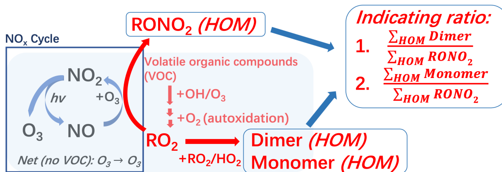
Figure A1. Sketch of the connection between HOM and O 3 formation. Based on the formation connection, two indicating ratios between HOM species are defined. "RONO 2 (HOM)": nitrate-containing HOM monomers, "Dimer (HOM)": non-nitrate HOM dimers, "Monomer (HOM)": non-nitrate HOM monomers.
