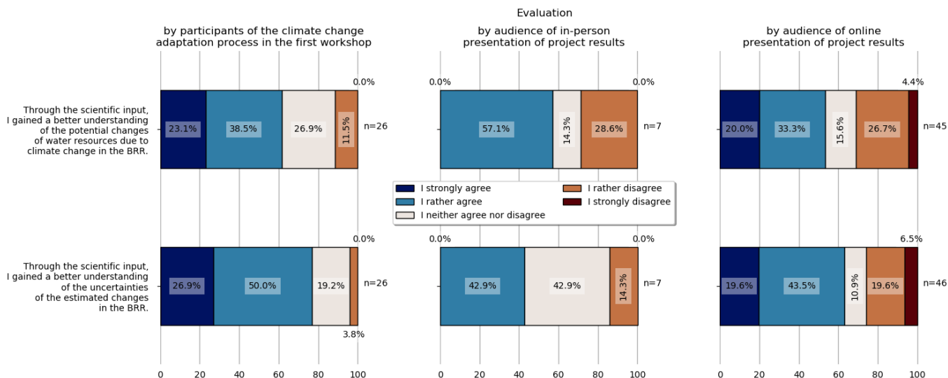
465 Figure 8. Results of the evaluation of the scientific input in the first workshop of the participatory process (left bars), and in the in-person presentation (middle bars) and online presentation (right bars) outside of the participatory process. The stakeholders and the audiences of the project presentations rated their agreement on the statements “Through the scientific input / the results (figures) just presented, I gained a better understanding of the potential changes of water resources due to climate change in the biosphere reserve Rhön” (upper bars) and “Through the scientific input, I gained a better understanding of the uncertainties of the estimated changes in the biosphere reserve Rhön” (lower bars). The bars show the results of the answers of 26 stakeholders (left bars), 7 470 participants (middle bars), and 45 and 46 participants (right bars). BRR: UNESCO biosphere reserve Rhön.
