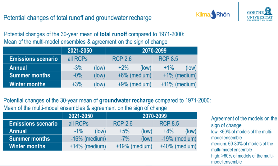
430 Figure 7. With this slide (the original slide was in German), the change in mean total runoff and mean groundwater recharge in the periods 2021-2050 (2035) and 2070-2099 (2084) as compared to 1971-2000 for the whole year (annual), only the summer months and
