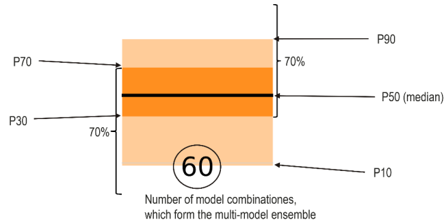
340 Figure 4. Schematic for the explanation of the percentile box, the first diagram that was explained to the stakeholders in the first workshop. The characteristic values P10, P30, P50 (median), P70, and P90 represent the interpolated values of percent change of either total runoff or groundwater recharge that is not exceeded by 10%, 30%, 50%, 70%, and 90% of simulated values of the multi-model ensemble, respectively.
