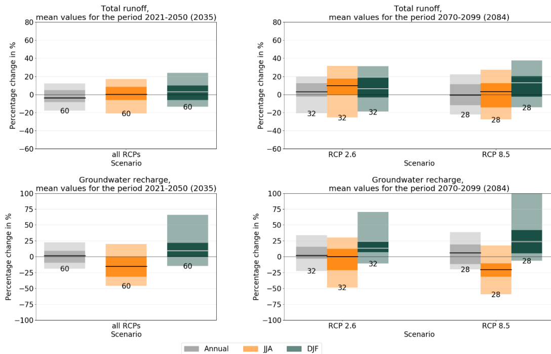
345 Figure 5. Percentile boxes showing the potential percentage changes of the mean total runoff and mean groundwater recharge of the multi-model ensemble in the periods around 2035 (2021-2050) and 2084 (2070-2099) relative to the reference period around 1985 (1971-2000) in the BRR. The figure shows the annual and seasonal (summer months June, July, and August JJA as well as winter months December, January, and February DJF) means. For the period around 2084, the results are shown separately for the emissions scenarios RCP 2.6 and 8.5. In the period around 2035, the simulations of both emissions scenarios RCP 2.6 and 8.5 are shown together in one percentile box (“all RCPs”). The black numbers below the percentile boxes show the number of model combinations of the multi-model ensemble. For groundwater recharge in winter months under RCP 8.5 in the period around 2084, the percentile box was cut for better visualization, as its P90 lies at around 150% (Figure 1). This figure was shown to the stakeholders directly after Figure 4 and was explained as shown in Section 3.2.2.1. An interpretation of the results is given in 350 Appendix A10.
