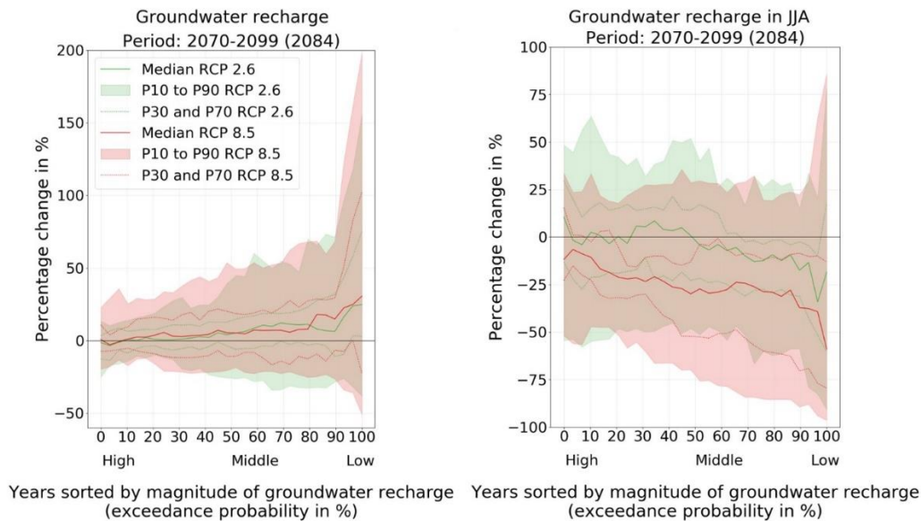
395 Figure 6. The third diagram, which was explained to the stakeholders in the first workshop, shows changes in the interannual variability of groundwater recharge. Percentage change of annual groundwater recharge (left diagram) and summer groundwater recharge in June, July, and August (JJA; right diagram) in the period around 2084 (2070-2099) relative to the reference period around 1985 (1971-2000) in the BRR. The 30 yearly groundwater recharge values are sorted according to their magnitude and the relative changes were calculated between the values of the same rank in the future and reference period. This sorting corresponds to the exceedance probability, which is shown in percent. As an example, an exceedance probability of 90% in the left diagram refers to the year in which groundwater recharge is lower than in 90 % of all years, i.e., lower than in 27 out of 30 years. If the percentage change for this unusually dry year is -10%, this means that the model projects that the groundwater recharge that is exceeded only in 3 out of 30 years in the future is 10% lower than in the respective year of the reference period. This figure was shown to the stakeholders directly after Figure 5 and was explained as shown in Section 3.2.2.2. An interpretation of the results is given in Appendix A11.
