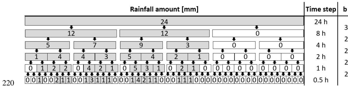
Figure 2: Multiplicative cascade model scheme for the first five disaggregation steps with branching numbers b , starting with a daily rainfall amount of 24 mm.
