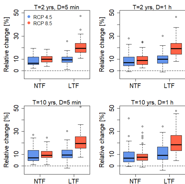
480 Figure 10: Relative change of the rainfall amount for a rainfall duration ( D ) of 5 min and 1 h with a return period of two years ( T = 2 yrs) and ten years ( T = 10 yrs) between the control period C20 (1971-2000) and the near-term future NTF (2021-2050) and the long-term future LTF (2071-2100), respectively for RCP 4.5 and RCP 8.5 across all locations.
