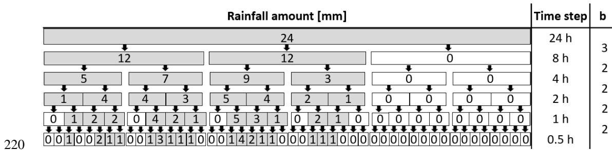
220 Figure 2: Multiplicative cascade model scheme for the first five disaggregation steps with branching numbers b , starting with a daily rainfall amount of 24 mm.
