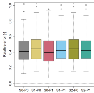
360 Figure 6: Relative error of the rainfall intensity with a return period of two years for all parameter reduction model variants over all locations.
