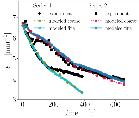
Figure 5. The time evolution of the SSA s for both series with coarse and fine temporal resolution for the best previously found values \alpha_{\text{Series 1}}^{\text{best}} , \alpha_{\text{Series 2}}^{\text{best}} .
