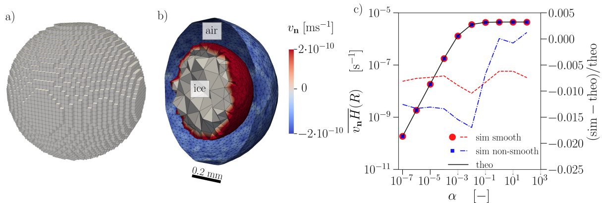
Figure 2. a) Voxeled sphere obtained from a binary image and used to constrain the problem. b) Clip of the outer and inner spherical shells with visible elements colored by the interface velocity v_n (sublimation in blue, deposition in red). c) Comparison of the growth rate \overline{v_n H} on the inner radius R of theoretical (theo) and simulated (sim) solution of the spherical shell test case for different values of the condensation coefficient \alpha . Two different surface mesh qualities with (smooth) and without (non-smooth) smoothing are employed. The red dots, blue squares and black solid line correspond to \overline{v_n H} on the left y-axis while the dashed red and blue lines correspond to simulation error on the right y-axis.
