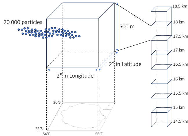
Figure 1: Illustration of the release of particles in FLEXPART
