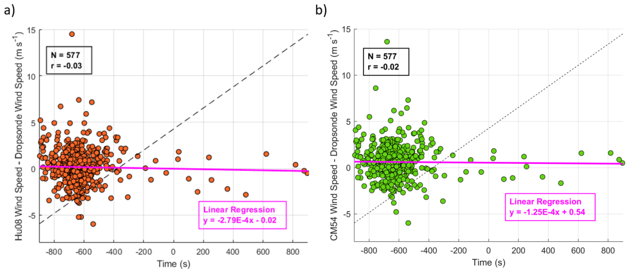
Figure S2: Time between HSRL-2 retrieval and dropsonde measurement versus a) Hu08 minus dropsonde wind speed and b) CM54 minus dropsonde wind speed to observe how time affects agreement in wind speed intercomparisons.
