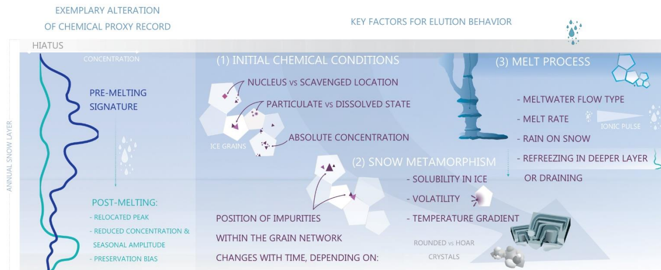
485 Figure 7: Schematic display of issues associated with melt-affected ice-core chemistry using a qualitative drawing (left), and key factors for elution behaviour of impurities (right) include (1) initial chemical conditions of the deposited snow, (2) segregation of impurities during snow metamorphism, and (3) the melt process itself.
