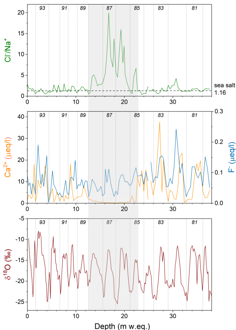
Figure 5: Records of \text{Cl}^-/\text{Na}^+ ratio (green), \text{Ca}^{2+} (orange) and \text{F}^- (blue) concentrations, and \delta^{18}\text{O} (brown) within the upper 38 m w.eq. of an ice core from Grenzgletscher (Swiss Alps, Eichler et al., 2001), covering the time period 1980–1994 (individual years are indicated, dotted lines): Meltwater inflow through a crevasse system led to (a) high \text{Cl}^-/\text{Na}^+ ratios, exceeding the sea-salt ratio (1.16, dashed line) in the melt-disturbed range (grey background), (b) preferential elution of \text{Ca}^{2+} compared to \text{F}^- , with the latter still showing well-preserved concentration seasonality in the depth range ~12–23 m w.eq., (c) whereas \delta^{18}\text{O} is mainly undisturbed; observations suggest lack of refreezing of the percolating meltwater but drainage along the firn-ice transition.
