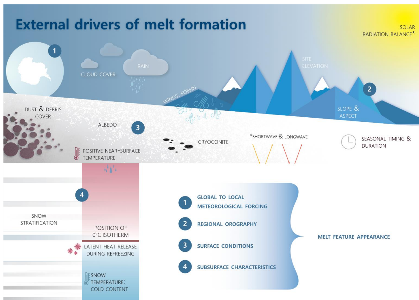
125 Figure 2: Schematic overview of the diverse, external drivers and constraints of near-surface snow melt discussed in Sect. 2.1., including global to local meteorological forcing, regional orography, surface conditions, and subsurface characteristics.
