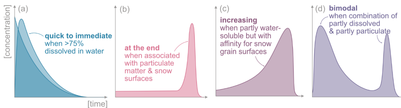
Figure 6: Differences in behaviour during melt elution of (a) water-soluble impurities, (b) particle-bound matter, (c) species that are partly water-soluble and partly sorbed to ice grain surfaces, and (d) impurities combining the dissolved type (a) and particulate type (b); this is a schematic summary based on modelling of organic compounds during melt by Meyer and Wania (2011).
