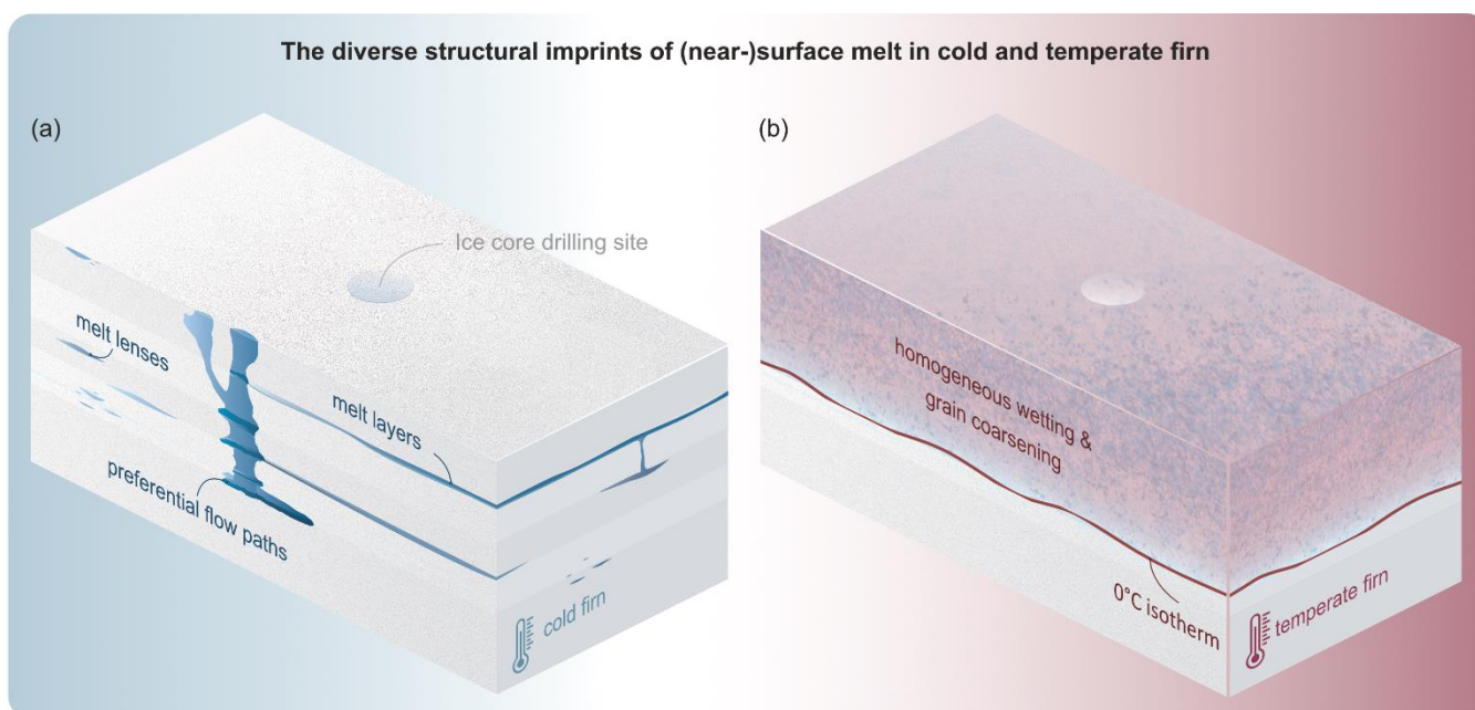
375 Figure 3: Examples of structural imprints of melt for the extreme scenarios of (a) cold firn and (b) temperate subsurface. Subsurface temperatures influence the meltwater flow through the differing refreezing capacity of the snowpack and therefore can lead to different melt features in firn. The profiles above show extreme examples of (a) cold firn with distinct melt layers, lenses and vertical flow fingers, and (b) temperate snow characterized by more homogeneous progression of the melting front and wide-spread grain coarsening. A continuum between these extremes allows for unique site- and event-specific structural manifestations of melt events under natural conditions.
