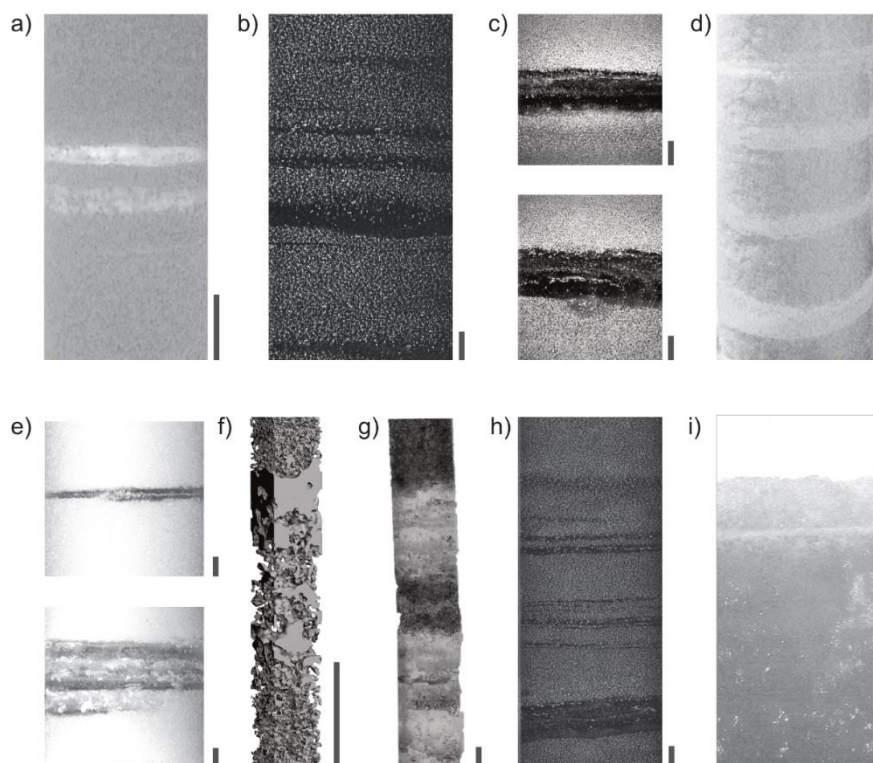
100 Figure 1: Examples of melt layers reported in snow and ice profiles from around the world using various techniques; a) two melt layers, 4–6 mm thick, from the NEEM Greenland ice core at ~44.3 m depth (digital photo, credit Kaitlin Keegan, Orsi et al., 2015); b) sequence of melt layers ranging 3–13 mm at EastGRIP, Greenland ice core at ~138.04 m depth, (line scan image, Westhoff et al., 2022, CC-BY 4.0); c) two distinct melt layers ~15–20 mm thick at RECAP, Renland Ice Cap, at 78.1–79.2 m depth (line scan image, Taranczewski et al., 2019); d) four ~20–35 mm melt layers at 0.3–0.5 m depth in an ice core from the Agassiz Ice Cap, Canada (digital 105 photo, credit James Zheng, Fisher et al., 2012); e) varying appearance of 3–7 mm and 25–41 mm melt layers in an ice core from Mount Hunter, Alaska (digital photo, Winski et al., 2018); f) ~15–20 mm melt at ~0.04 m depth in surface snowpack from Davos, Swiss Alps (3D X-ray tomography scan, Heggli et al., 2011); g) segment at ~3 m depth from the Young Island ice core with melt >45 mm thick (digital photo, Moser et al., 2021, CC-BY 4.0); h) melt sequence between 133.82–1.92 m depth in ice core from James Ross Island, Antarctic Peninsula (line scan image, Abram et al., 2013); i) a 1-mm melt layer in the surface snow at 0.008 m depth at Siple 110 Dome, Antarctica (digital photo, Das and Alley, 2005); the grey scale bar at the bottom right of each panel equals 1 cm; the top of each snow/firn/ice section is at the top of each panel.
