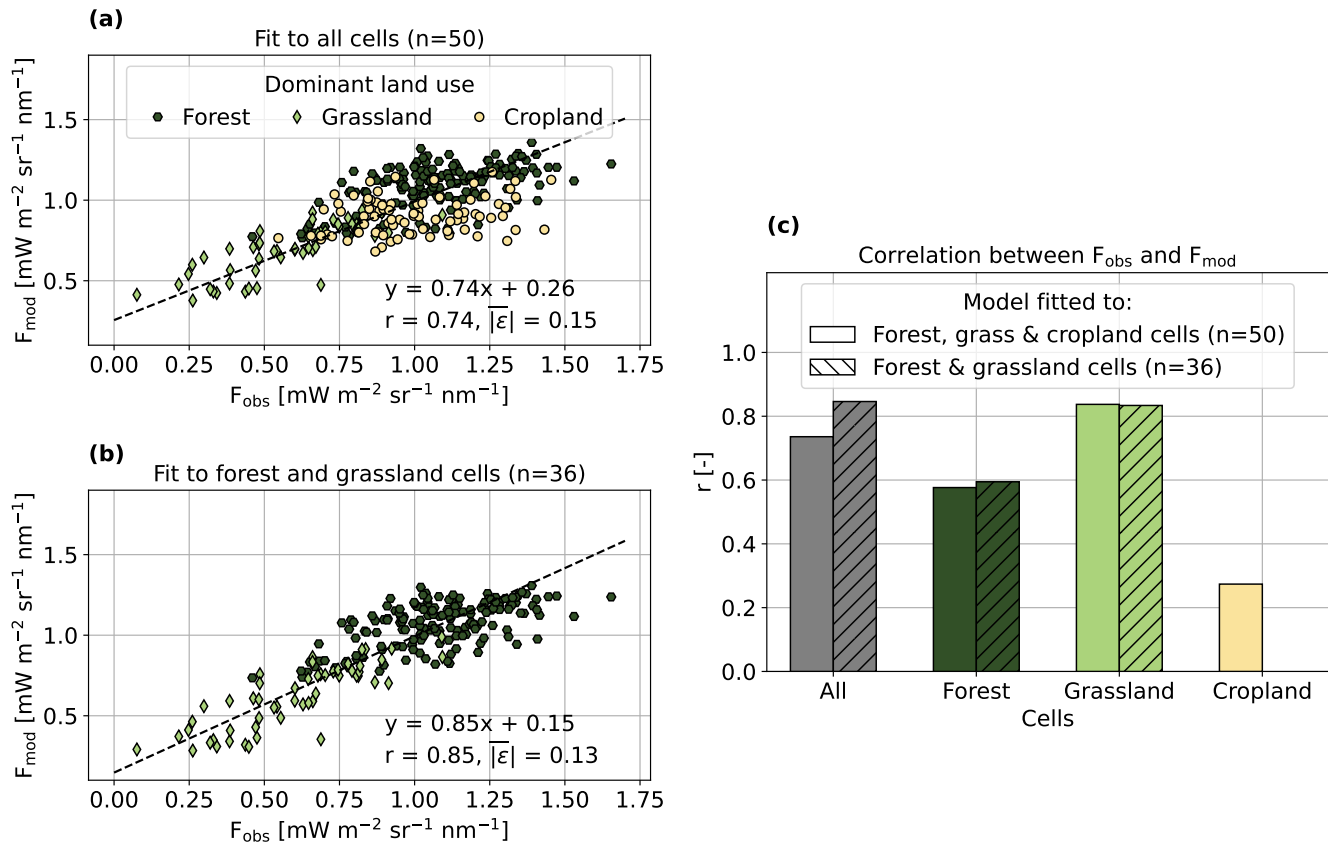
Figure 8. Results from the regression model in Eq. (3) fitted to (a) all cells ( n=50 ) and (b) exclusively to forest and grassland cells ( n=36 ). (c) Shows the correlation between observed ( F_{\text{obs}} ) and modelled ( F_{\text{mod}} ) SIF for each dominant land use type and for both fits.
