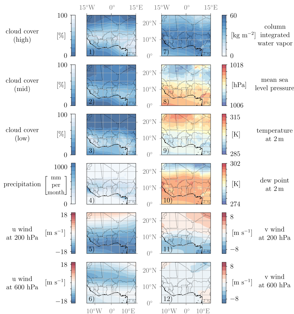
Figure 6. Average of selected output fields over the evaluation period (Augusts 2016–2019), averaged over all available ICON simulations. Figure numbers are chosen in accordance with the variables and labels in Figs. 7–9. All scales are linear.
