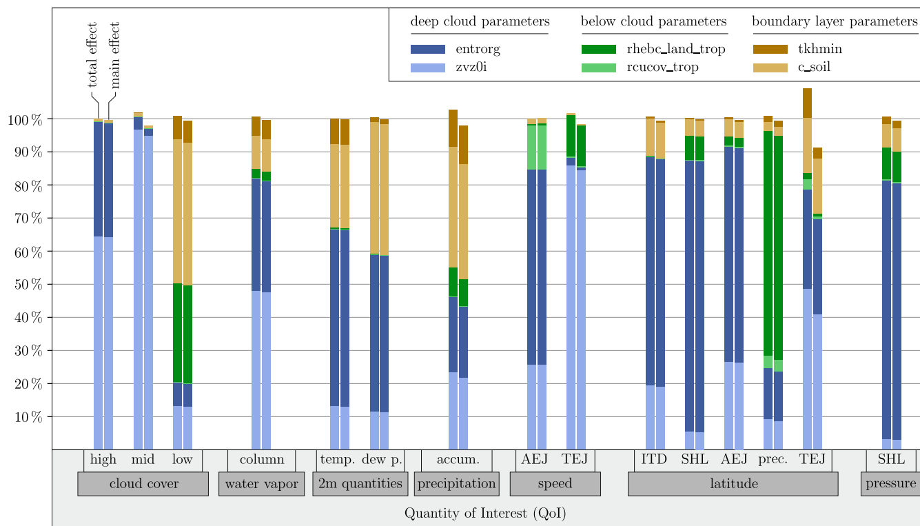
Figure 4. Main and total effect sensitivity indices of the six selected uncertain model parameters for all QoIs, respectively, as result of the global sensitivity analysis FAST.
