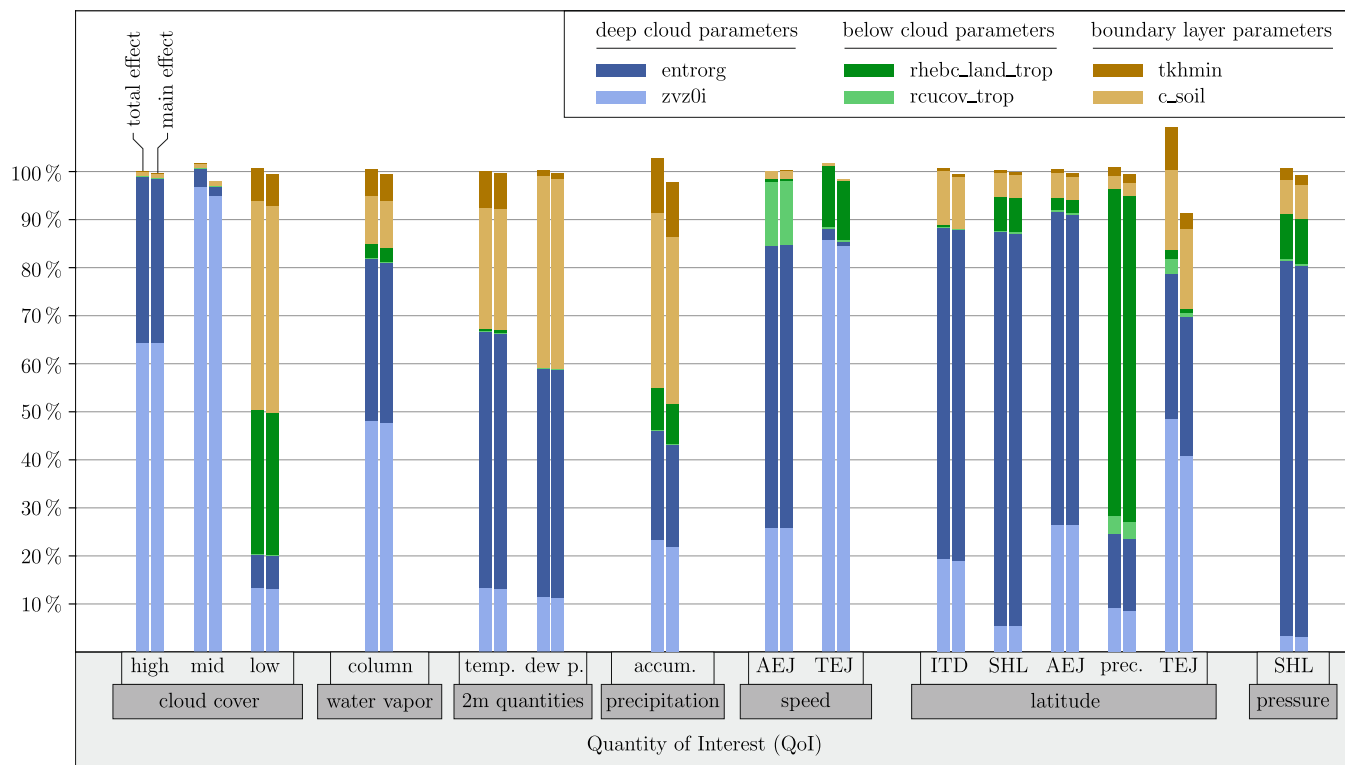
Figure 4. Main and total effect sensitivity indices of the six selected uncertain model parameters for all QoIs, respectively, as result of resulting from the global sensitivity analysis FAST.
