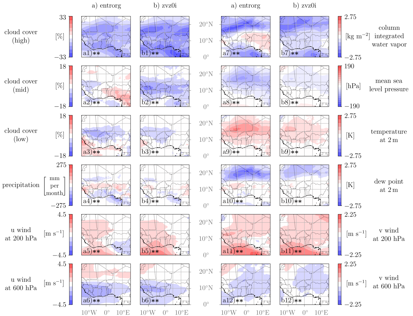
Figure 7. Spatial variability of selected output fields for the uncertain model parameters entrorg and zVz0i . The difference of the output quantity with respect to an increase of the model parameter value based on the sets \mathbf{X}_{i,\text{low}} and \mathbf{X}_{i,\text{high}} (see Sect. 2.5) is shown. Results of the statistical test are denoted with (**): very-high statistical significance on a 5% level, p < 0.05 , (*): high statistical significance ; 0.05 < p < 0.10 on a 10% level . All scales are linear.
