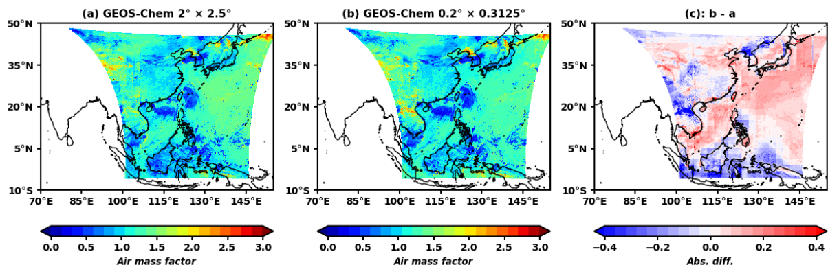
605 Fig. 3. GEMS HCHO air mass factor (3 August 2020, 12:45 KST (03:45 UTC)): The GEMS algorithm with initial a priori profile (a), GEMS with the updated a priori profile (b), and the absolute differences of b-a (c).
