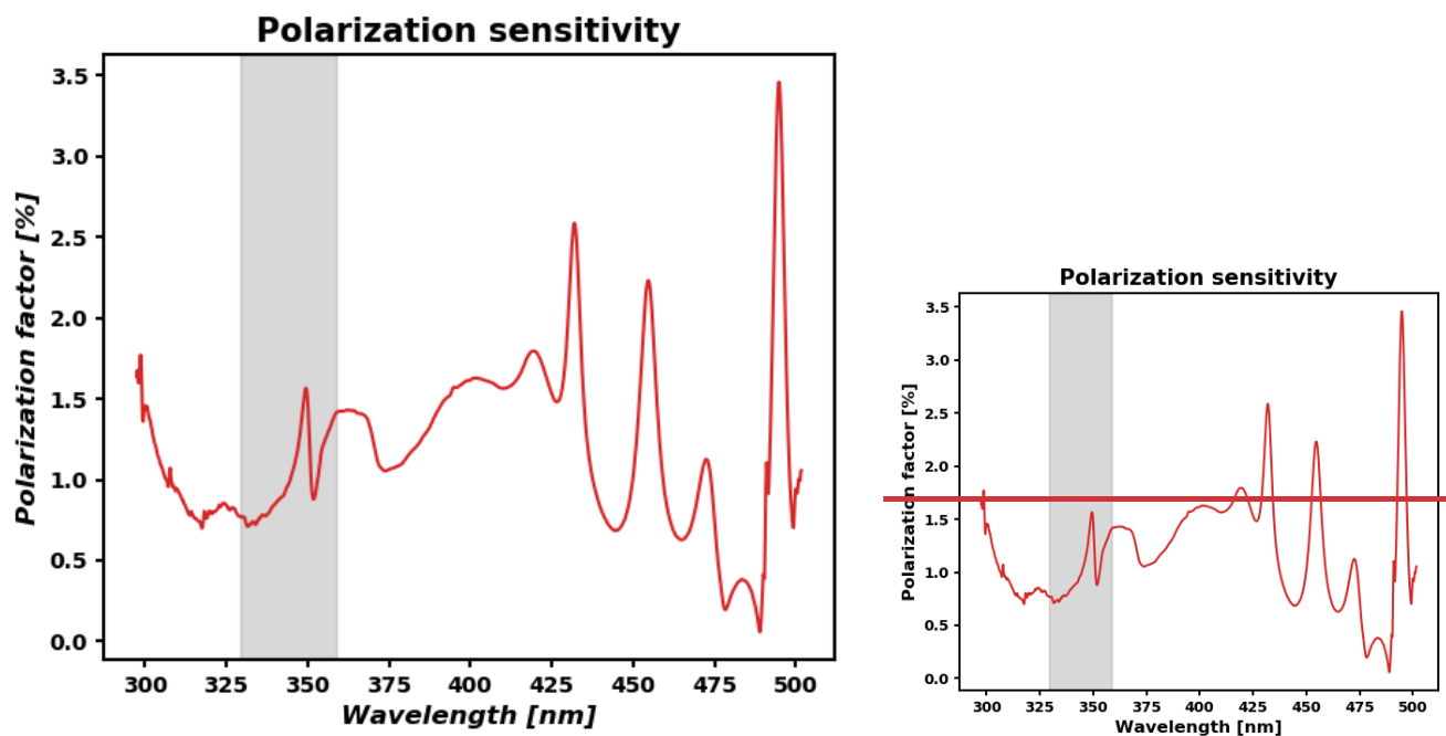
Fig. 4. Polarization sensitivity vector of the GEMS instrument (shaded area: fitting window of the GEMS HCHO).
