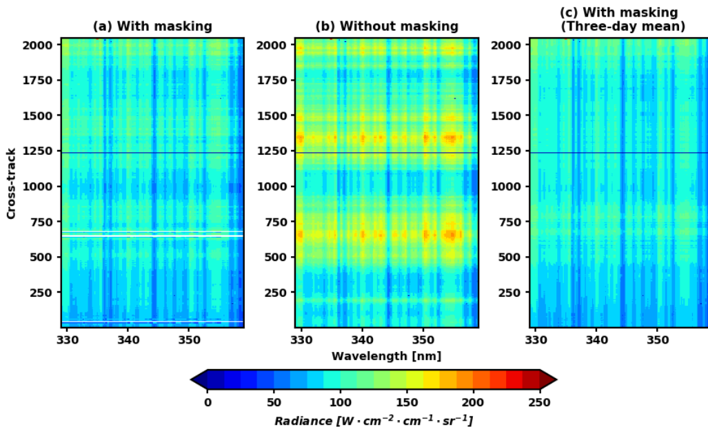
595 Fig. 1. Latitudinally averaged radiance references of GEMS (03:45 UTC (12:45 KST), 6 December 2020): With cloud masking (cloud radiance fraction > 0.4) (a), without cloud masking (b), and cloud masking with three-day mean radiances (c). The shadings are radiance spectra. The radiance spectra in the 1233–1241 cross tracks have bad L1C quality flags.
