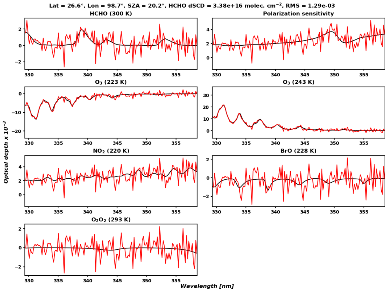
600 Fig. 2. Fitted optical depths (black solid line) and optical depths plus the fitting residuals (red solid line) of the operational GEMS HCHO retrieval algorithm in Northern Myanmar at 12:45 KST (03:45 UTC), 3 August 2020.
